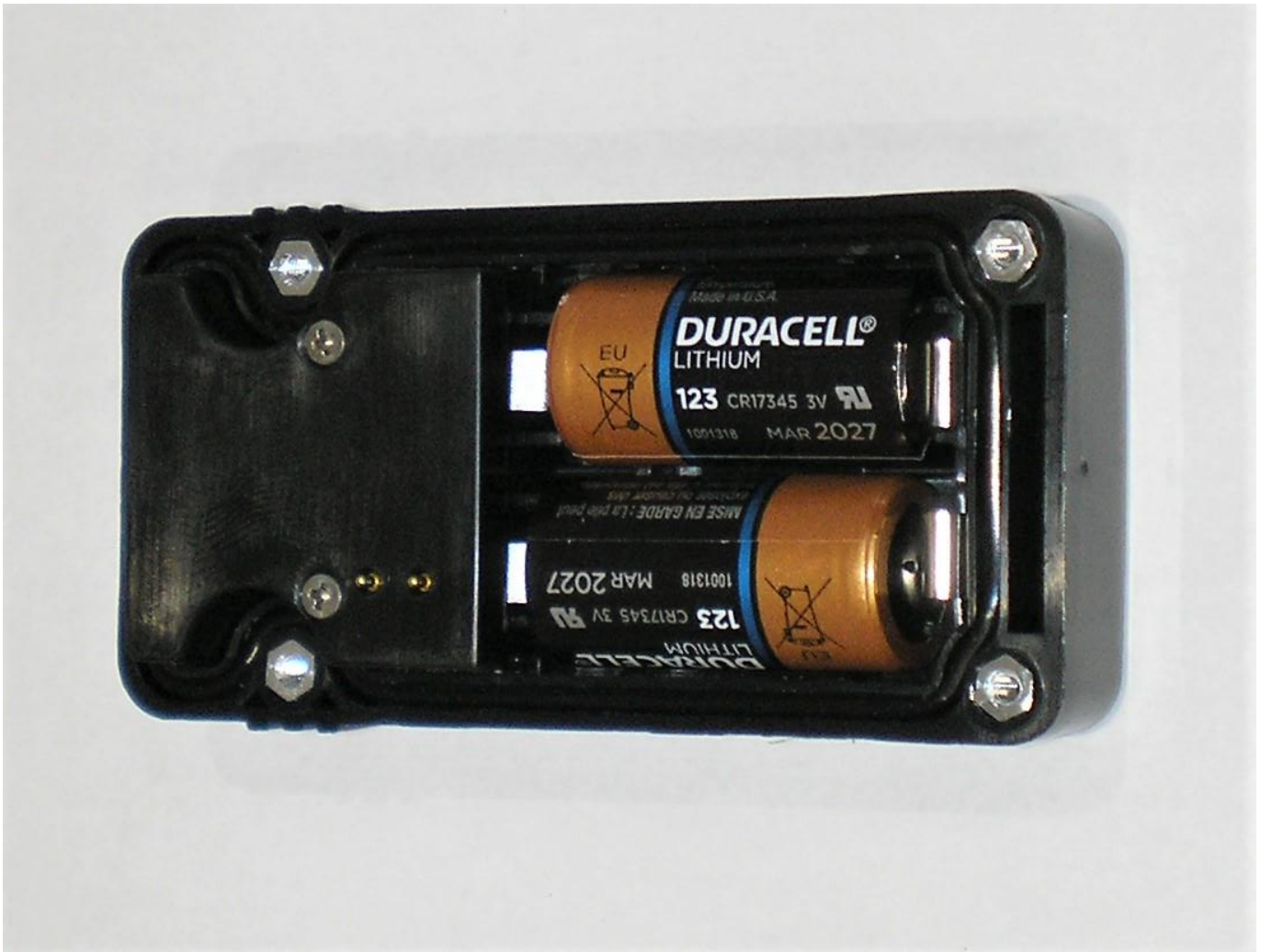
Interior with PCBs, inner PCB cover, and batteries installed
