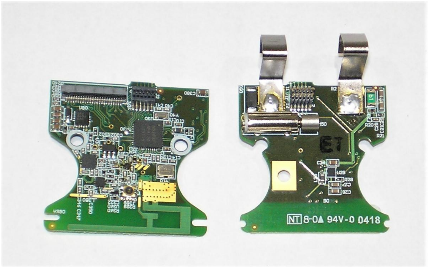
PCB Inner Surfaces (These surfaces face one another in the assembled unit)
