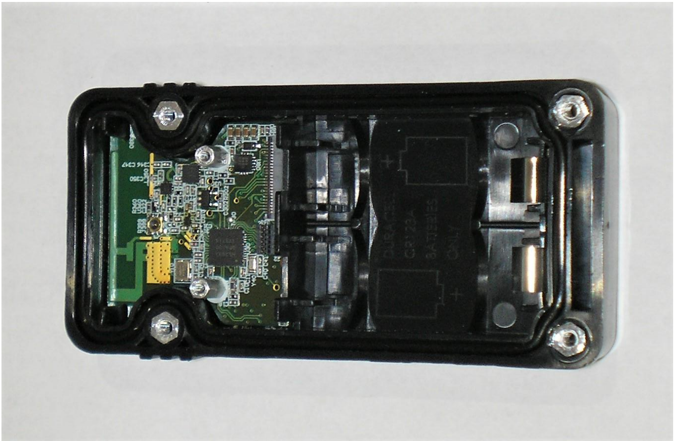
Case with first PCB installed.
