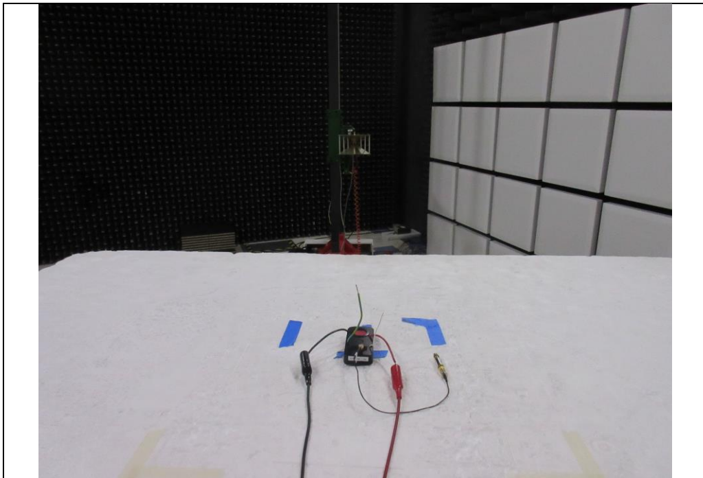
RF Radiated #6
