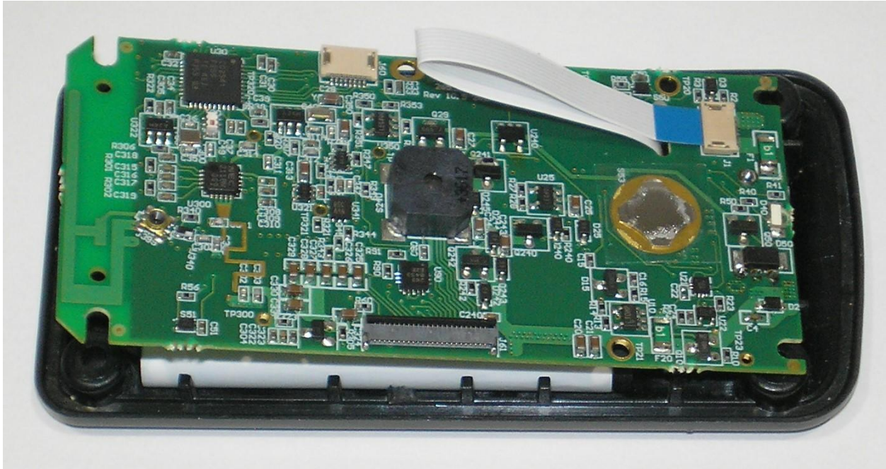
Interior, PCB Component Side, View from Left
