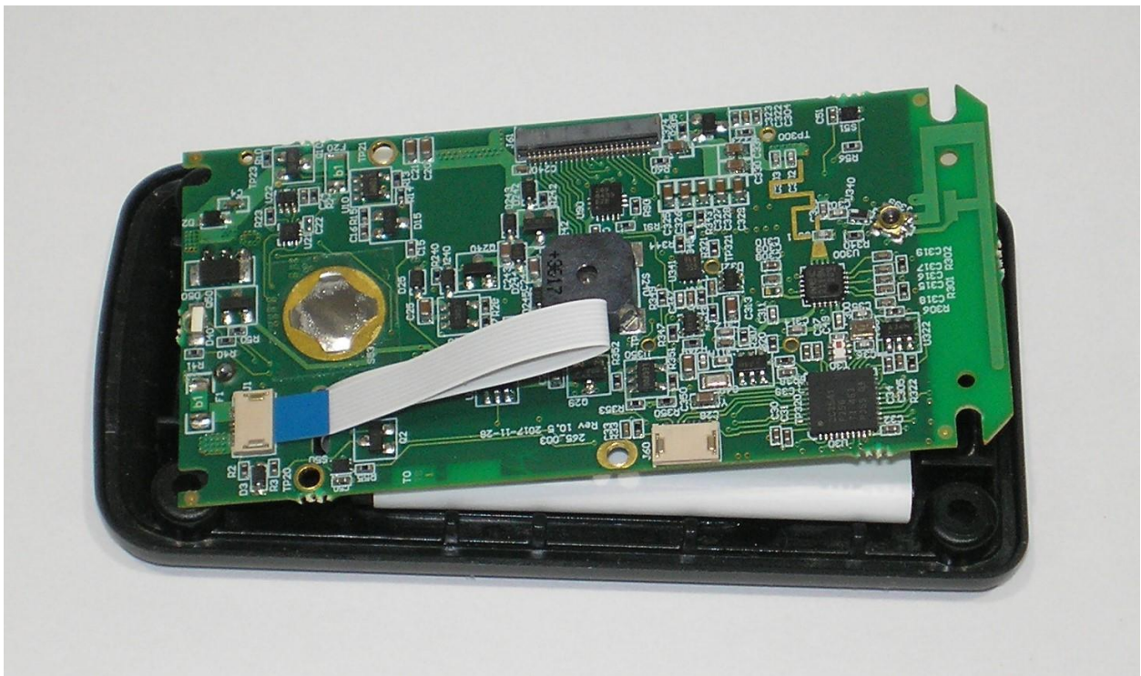
Interior, PCB Component Side, View from Right
