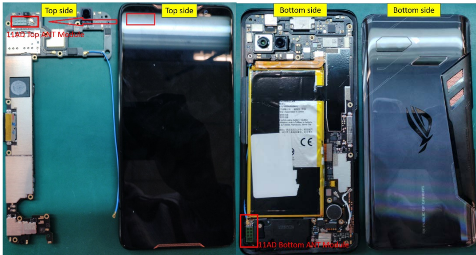
Figure C-1 802.11ad antenna module inside ASUS_Z01QD
