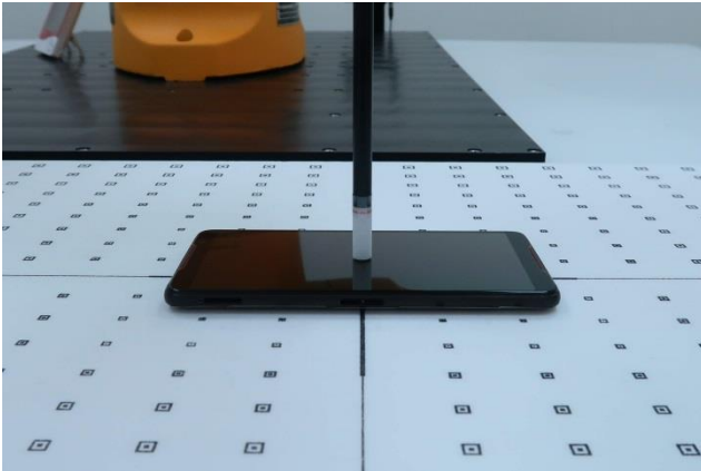
Front, Probe sensor to EUT surface distance 2mm Back, Probe sensor to EUT surface distance 2mm
