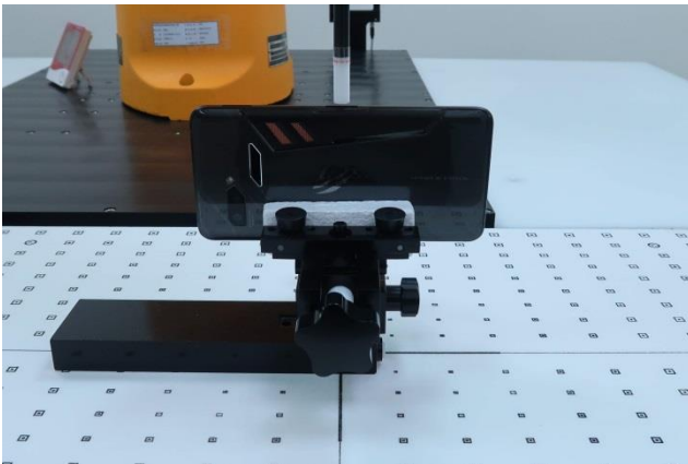
Left Side, Probe sensor to EUT surface distance 2mm Right Side, Probe sensor to EUT surface distance 2mm
