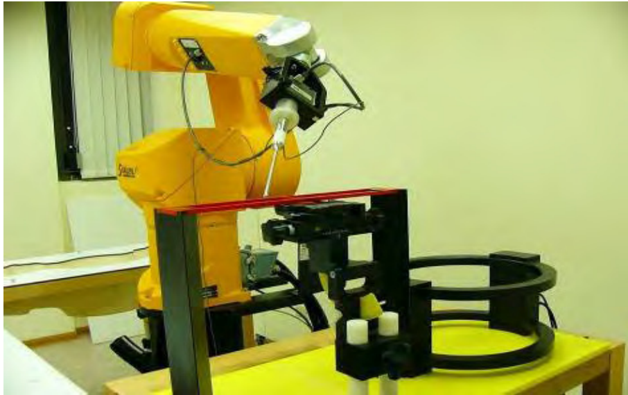
Fig. 1 Photograph of the DASY 5 measurement system
