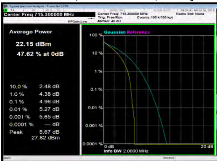
1.4MHz BW LTE-Band 12(16QAM Number: 6 Offset: 0) Channel High
