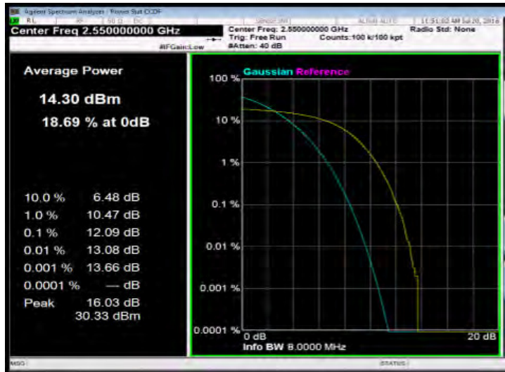
10MHz BW LTE-Band 41(16QAM Number: 50 Offset: 0) Channel Mid
