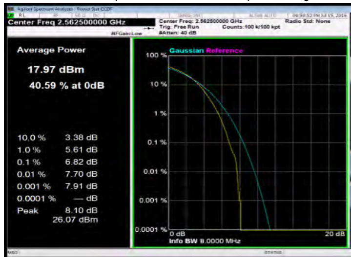
15MHz BW LTE-Band 7(16QAM Number: 75 Offset: 0) Channel High
