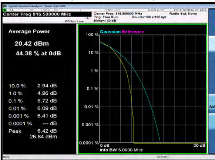
5MHz BW LTE-Band 26 (16QAM Number: 25 Offset: 0) Channel Low
