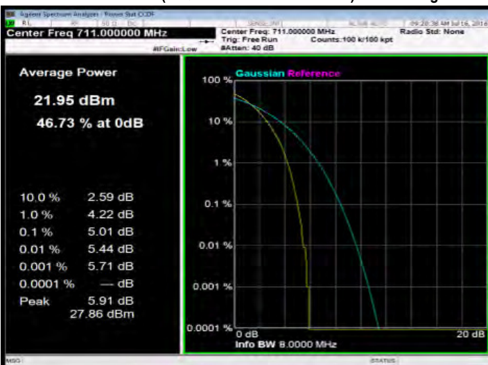
10MHz BW LTE-Band 12(16QAM Number: 50 Offset: 0) Channel High
