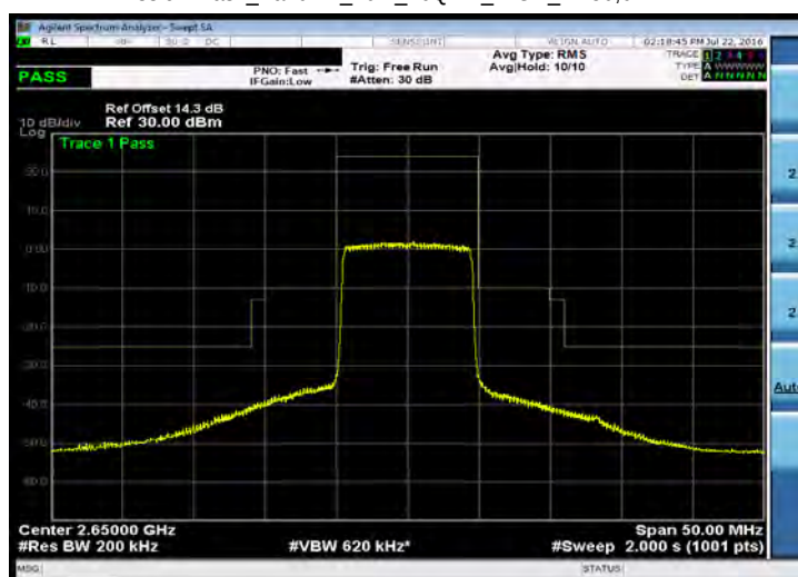
Emission Mask_Band 41_10M_16QAM_HIGH_RB50,0
