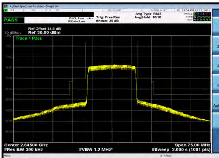
Emission Mask_Band 41_20M_16QAM_HIGH_RB100,0
