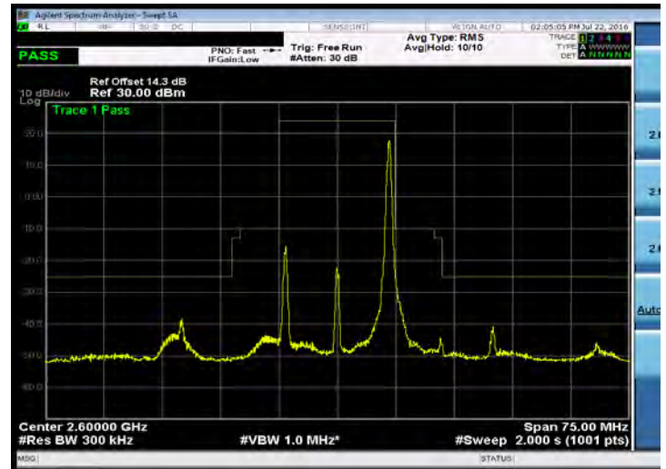
Emission Mask_Band 41_15M_16QAM_MID_RB1,74
