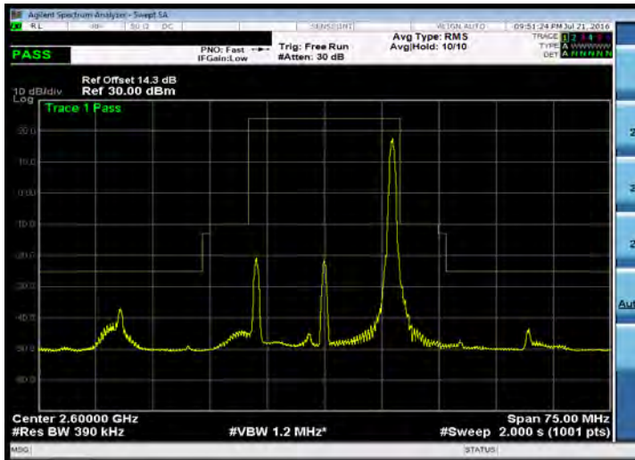
Emission Mask_Band 41_20M_QPSK_MID_RB100,0
