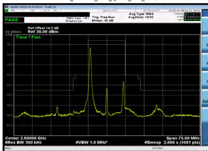
Emission Mask_Band 41_15M_QPSK_MID_RB1,0
