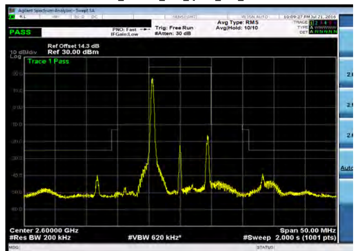
Emission Mask_Band 41_10M_QPSK_MID_RB1,0
