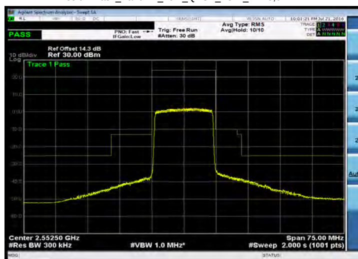
Emission Mask_Band 41_15M_QPSK_LOW_RB75,0
