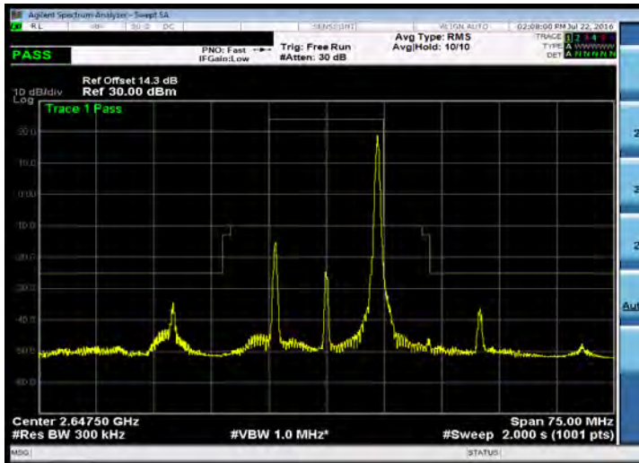
Emission Mask_Band 41_15M_16QAM_HIGH_RB1,74
