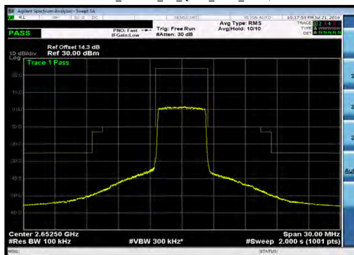
Emission Mask_Band 41_5M_QPSK_HIGH_RB25,0
