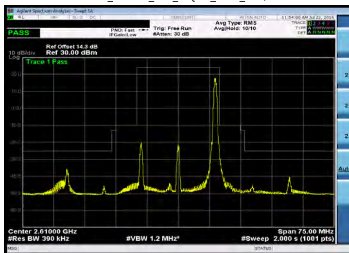
Emission Mask_Band 38_20M_16QAM_HIGH_RB1,99
