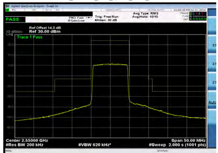
Emission Mask_Band 41_10M_QPSK_LOW_RB50,0
