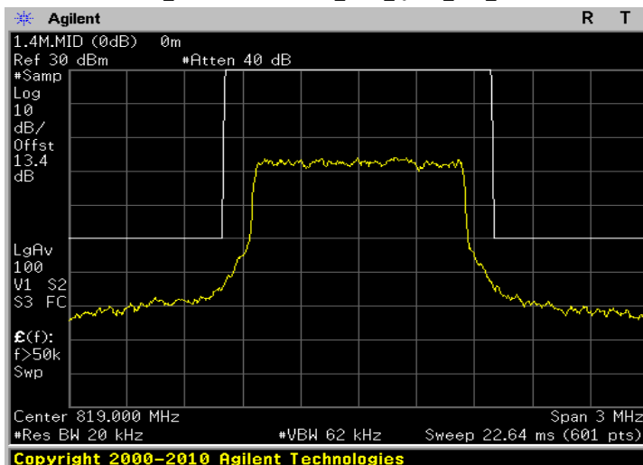
Emission Mask_Band26 for Part 90S_1.4M_QPSK_MID_RB6,0
