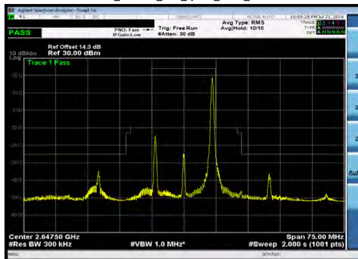
Emission Mask_Band 41_15M_QPSK_HIGH_RB75,0
