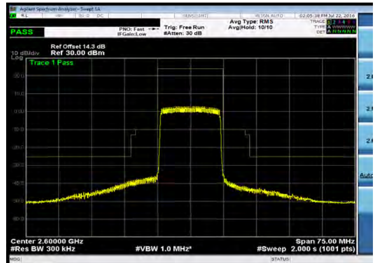
Emission Mask_Band 41_15M_16QAM_MID_RB75,0
