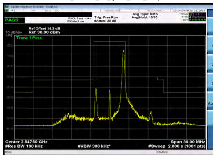
Emission Mask_Band 41_5M_QPSK_LOW_RB1,24
