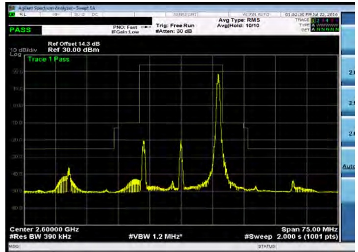
Emission Mask_Band 41_20M_16QAM_MID_RB1,99
