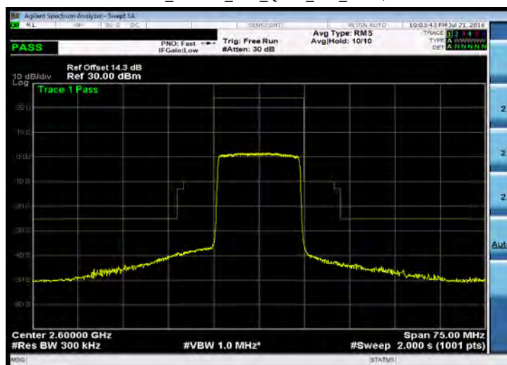
Emission Mask_Band 41_15M_QPSK_MID_RB75,0
