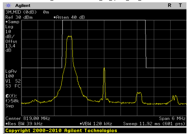
Emission Mask Band26 for Part 90S 3M QPSK MID RB1,0
