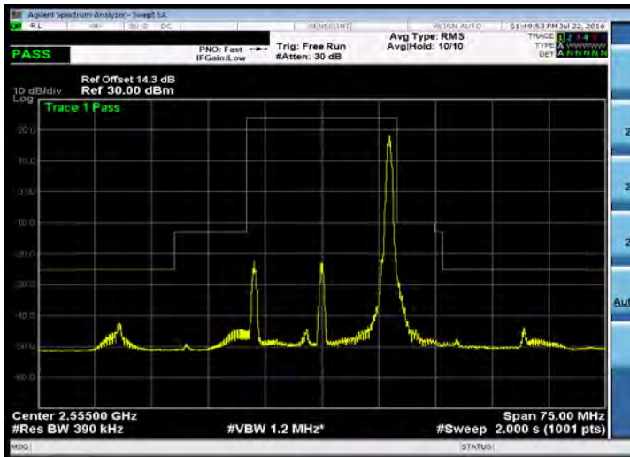
Emission Mask_Band 41_20M_16QAM_LOW_RB1,99
