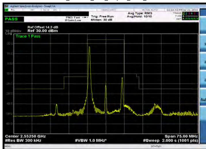
Emission Mask_Band 41_15M_16QAM_LOW_RB1,0
