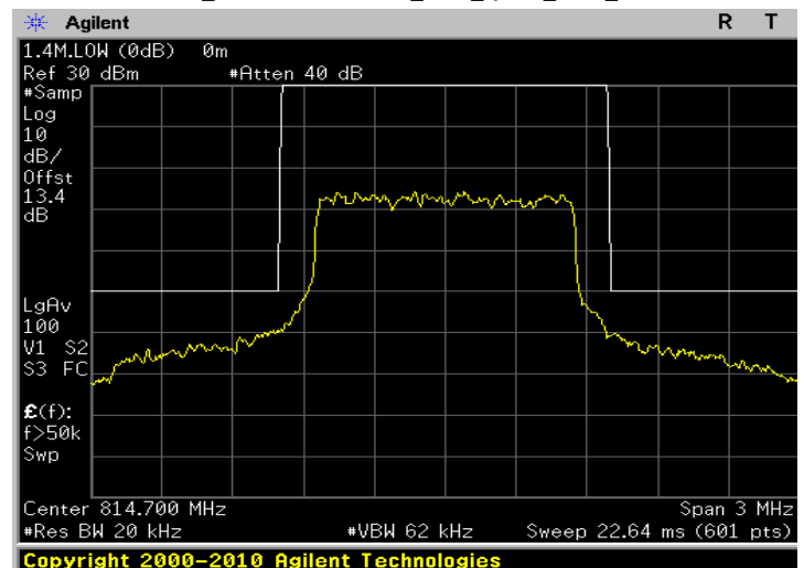
Emission Mask_Band26 for Part 90S_1.4M_QPSK_LOW_RB6,0
