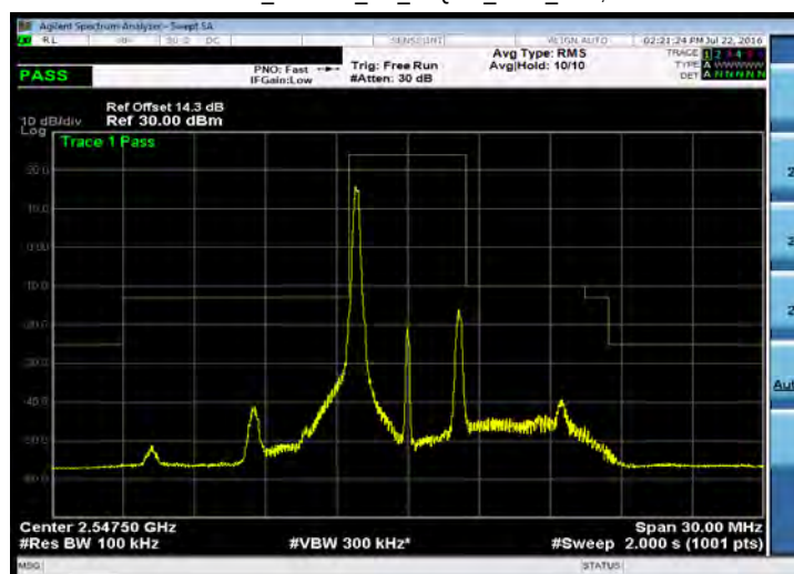
Emission Mask_Band 41_5M_16QAM_LOW_RB1,0
