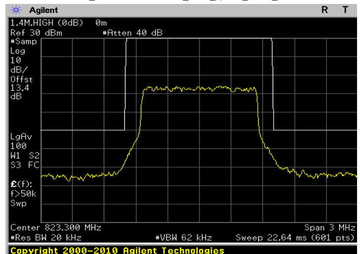
Emission Mask_Band26 for Part 90S_1.4M_QPSK_HIGH_RB6,0
