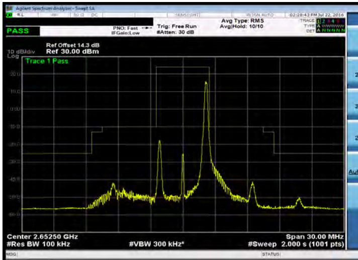
Emission Mask_Band 41_5M_16QAM_HIGH_RB1,24
