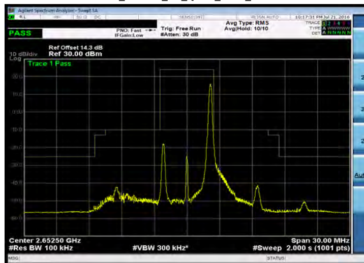
Emission Mask_Band 41_5M_QPSK_HIGH_RB1,24
