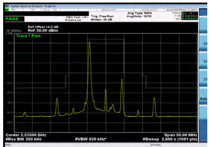
Emission Mask_Band 7_10M_QPSK_MID_RB1,0
