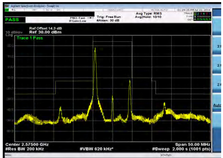
Emission Mask_Band 38_10M_16QAM_LOW_RB1,0
