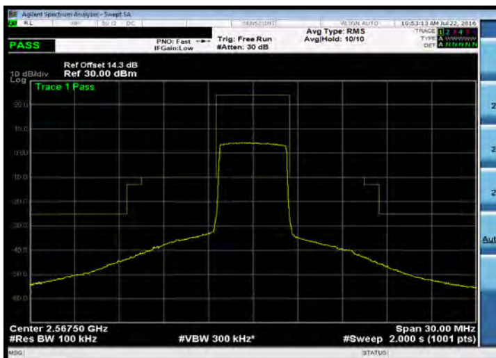
Emission Mask_Band 7_5M_16QAM_HIGH_RB25,0
