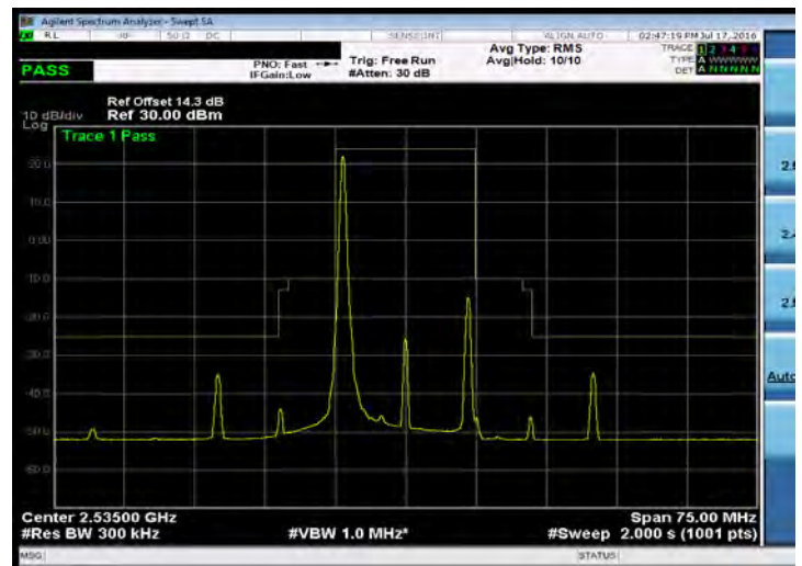
Emission Mask_Band 7_15M_QPSK_MID_RB1,0
