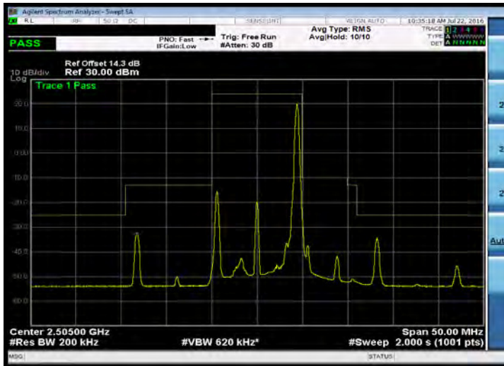
Emission Mask_Band 7_10M_16QAM_LOW_RB1,49
