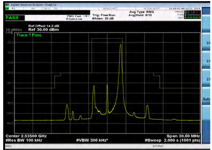
Emission Mask_Band 7_5M_16QAM_MID_RB25,0
