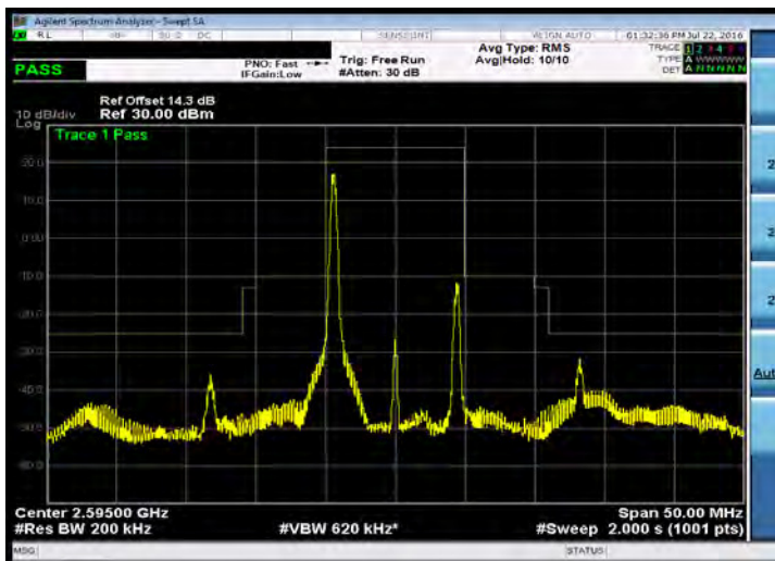
Emission Mask_Band 38_10M_16QAM_MID_RB1,0
