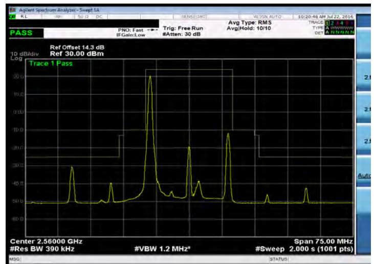
Emission Mask_Band 7_20M_16QAM_HIGH_RB1,0
