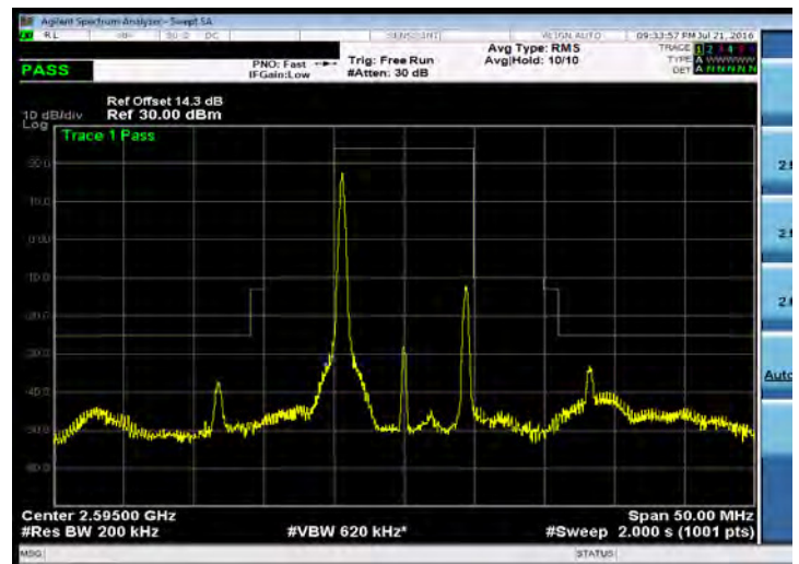
Emission Mask_Band 38_10M_QPSK_MID_RB1,0
