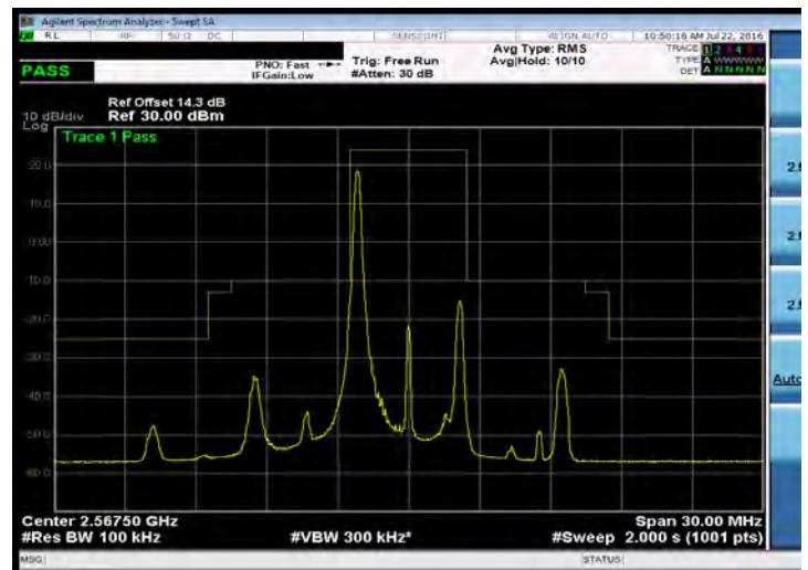
Emission Mask_Band 7_5M_16QAM_HIGH_RB1,0
