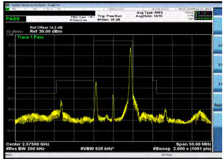
Emission Mask_Band 38_10M_QPSK_LOW_RB50,0
