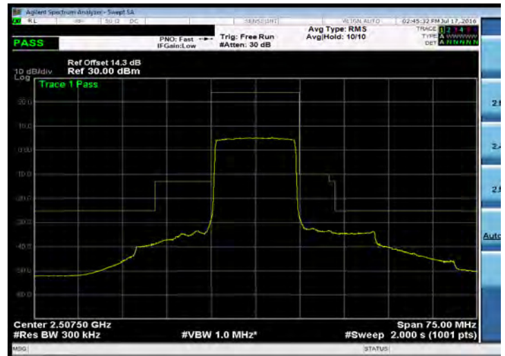
Emission Mask_Band 7_15M_QPSK_LOW_RB75,0
