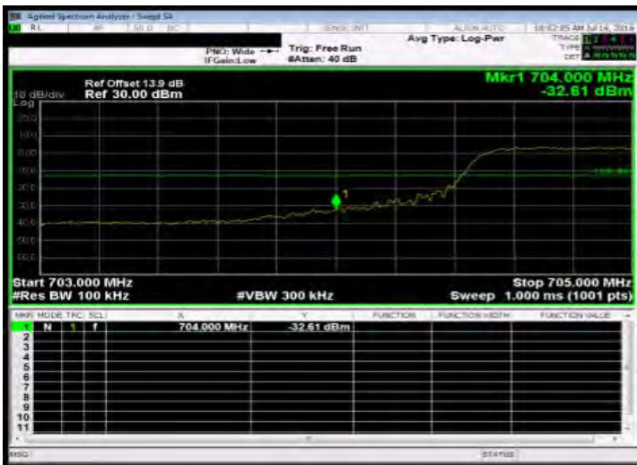
Band Edge_Band17 10MHz_QPSK 50 0_LowCH23780-709
