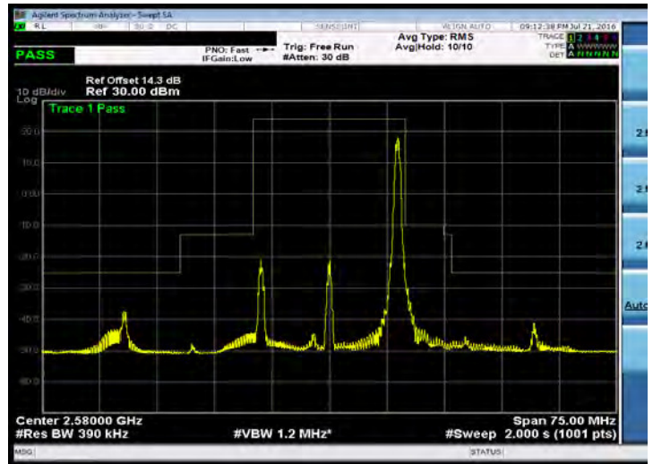
Emission Mask_Band 38_20M_QPSK_LOW_RB100,0
