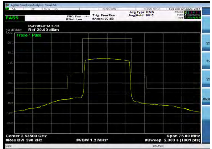
Emission Mask_Band 7_20M_16QAM_MID_RB100,0
