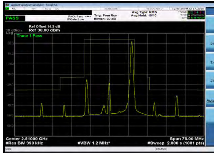
Emission Mask_Band 7_20M_QPSK_LOW_RB100,0
