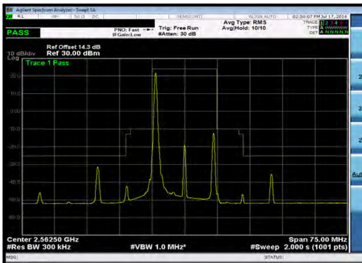
Emission Mask_Band 7_15M_QPSK_HIGH_RB1,0
