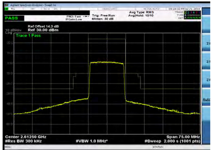
Emission Mask_Band 38_15M_QPSK_HIGH_RB75,0
