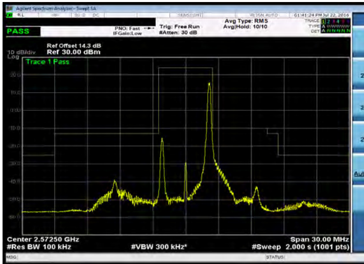
Emission Mask_Band 38_5M_16QAM_LOW_RB25,0
