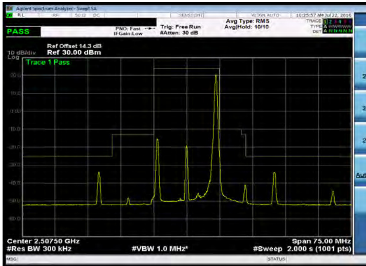
Emission Mask_Band 7_15M_16QAM_LOW_RB75,0
