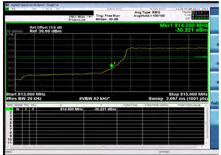
Band Edge_Band 26 for Part 90S_1.4M-QPSK-6 0-HIGH
