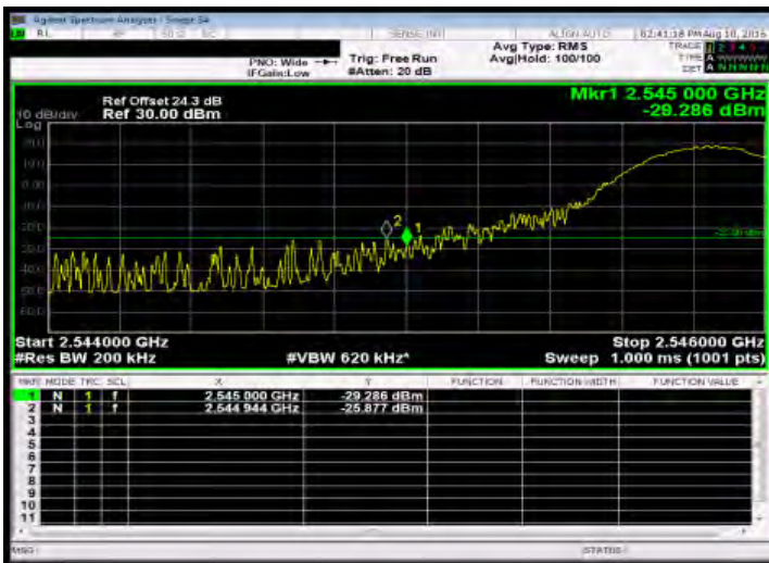
Band Edge_Band41 15MHz_QPSK 1 0_LowCH40215-2552.5
