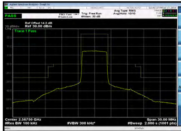
Emission Mask_Band 7_5M_16QAM_LOW_RB1,0
