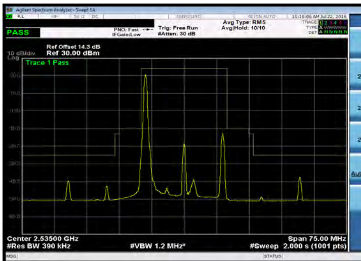
Emission Mask_Band 7_20M_16QAM_MID_RB1,0
