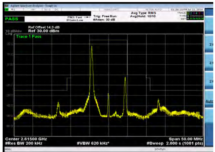
Emission Mask_Band 38_10M_16QAM_HIGH_RB1,0
