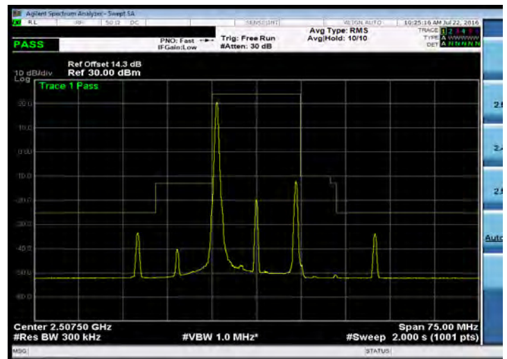
Emission Mask_Band 7_15M_16QAM_LOW_RB1,0
