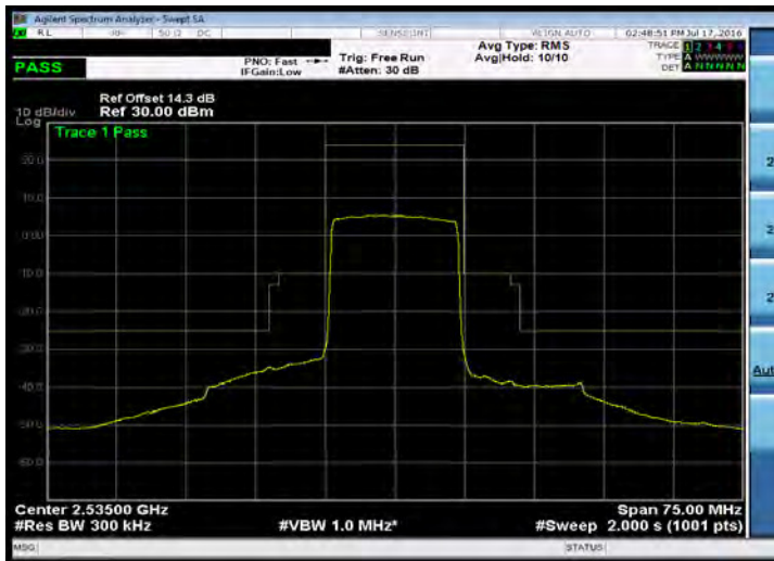
Emission Mask_Band 7_15M_QPSK_MID_RB75,0
