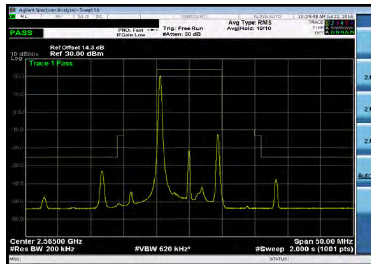
Emission Mask_Band 7_10M_16QAM_HIGH_RB1,0
