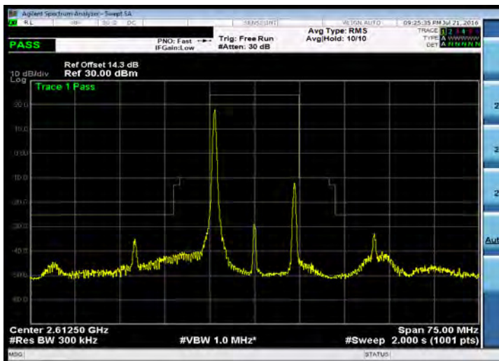
Emission Mask_Band 38_15M_QPSK_HIGH_RB1,0
