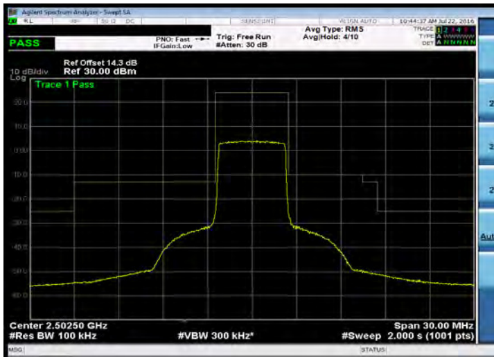
Emission Mask_Band 7_5M_16QAM_LOW_RB25,0
