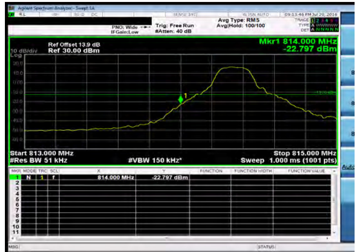
Band Edge_Band 26 for Part 90S_5M-16QAM-1 24-HIGH
