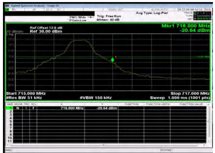
Band Edge_Band12 5MHz_QPSK 1 24_HighCH23155-713.5
