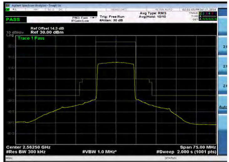
Emission Mask_Band 7_15M_QPSK_HIGH_RB75,0
