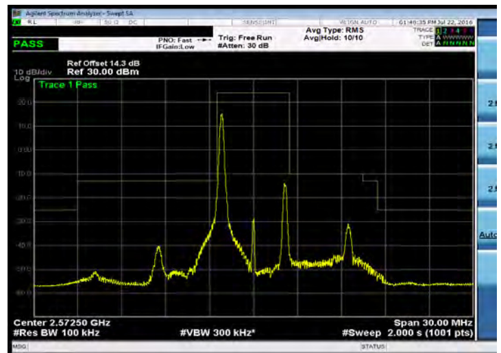
Emission Mask_Band 38_5M_16QAM_LOW_RB1,0
