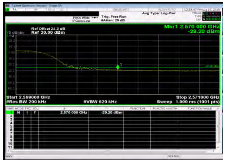
Band Edge_Band7 15MHz_QPSK 75 0_HighCH21375-2562.5
