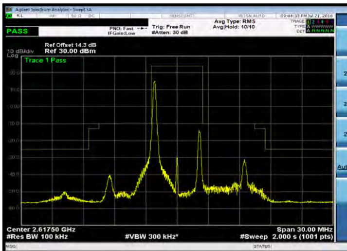
Emission Mask_Band 38_5M_QPSK_HIGH_RB1,0
