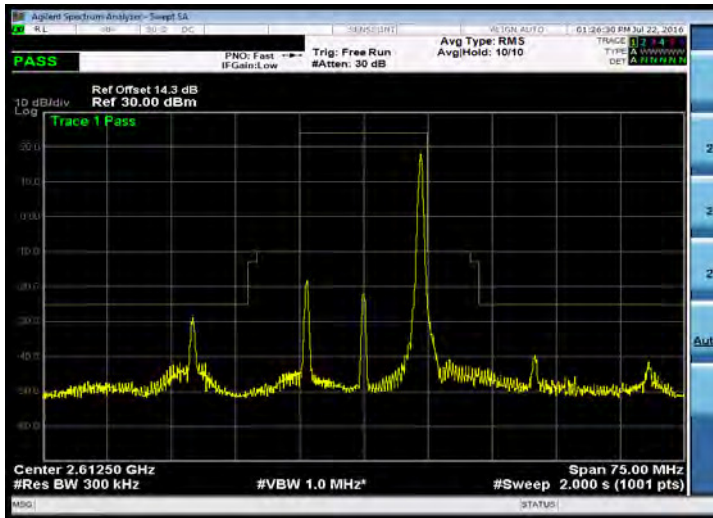
Emission Mask_Band 38_15M_16QAM_HIGH_RB75,0
