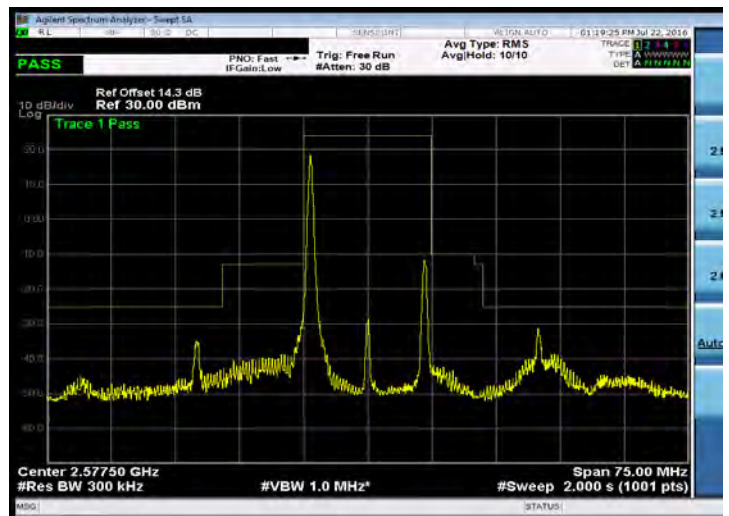
Emission Mask_Band 38_15M_16QAM_LOW_RB1,0
