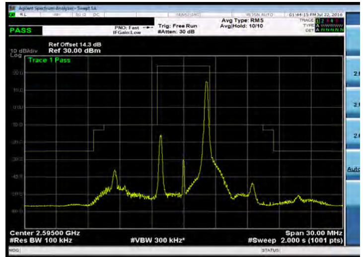
Emission Mask_Band 38_5M_16QAM_MID_RB25,0
