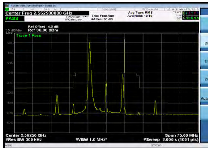
Emission Mask_Band 7_15M_16QAM_HIGH_RB1,0
