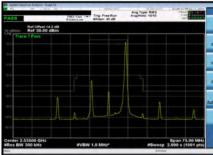
Emission Mask_Band 7_15M_QPSK_MID_RB1,74
