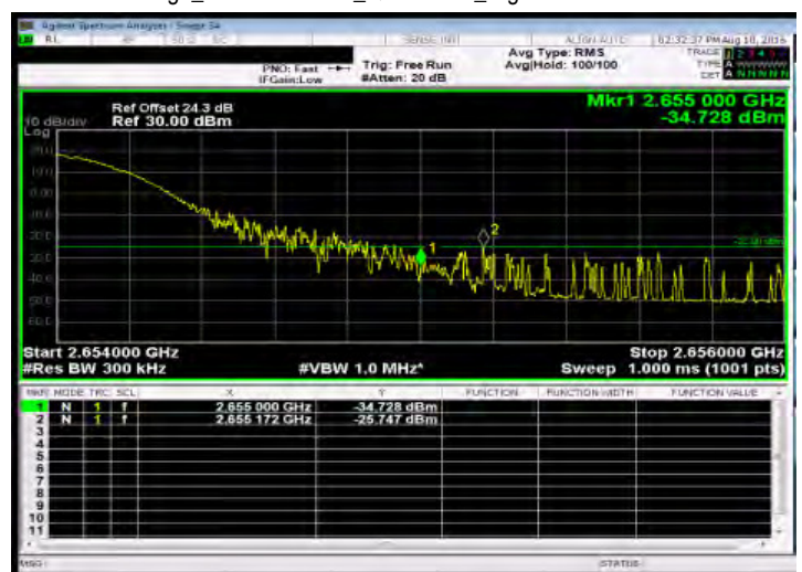
Band Edge_Band41 20MHz_QPSK 1 99_HighCH41140-2645
