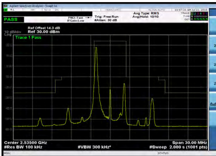
Emission Mask_Band 7_5M_16QAM_MID_RB1,0
