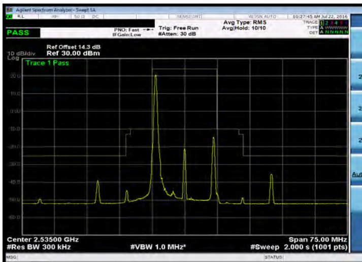
Emission Mask_Band 7_15M_16QAM_MID_RB1,0
