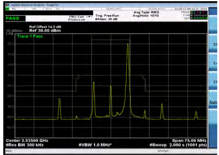
Emission Mask_Band 7_15M_16QAM_MID_RB75,0
