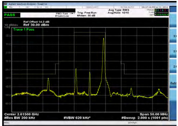
Emission Mask_Band 38_10M_QPSK_HIGH_RB50,0
