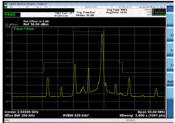
Emission Mask_Band 7_10M_QPSK_LOW_RB50,0
