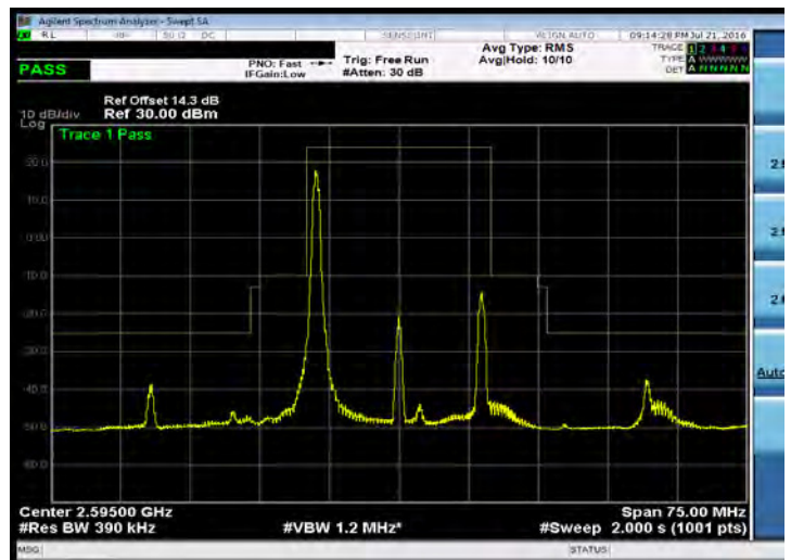
Emission Mask_Band 38_20M_QPSK_MID_RB1,0
