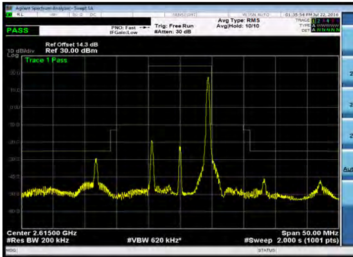
Emission Mask_Band 38_10M_16QAM_HIGH_RB50,0
