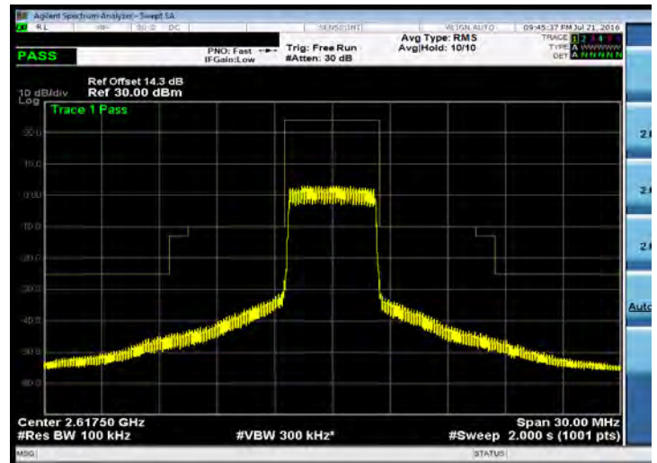
Emission Mask_Band 38_5M_QPSK_HIGH_RB25,0
