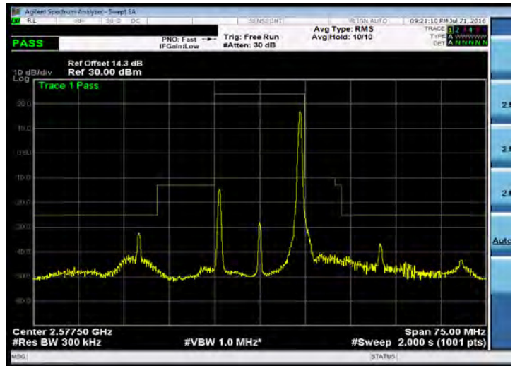
Emission Mask_Band 38_15M_QPSK_LOW_RB75,0
