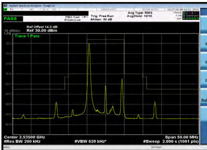
Emission Mask_Band 7_10M_16QAM_MID_RB1,0
