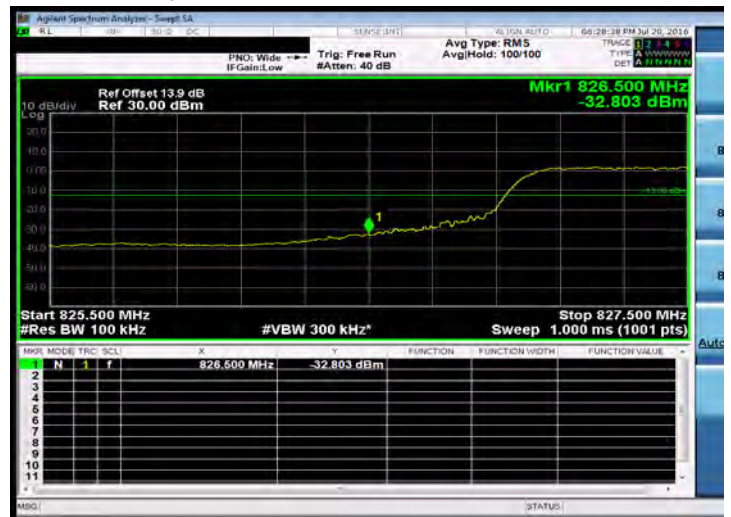
Band Edge_Band 26 for Part 90S_10M-QPSK-50 0-MID/R
