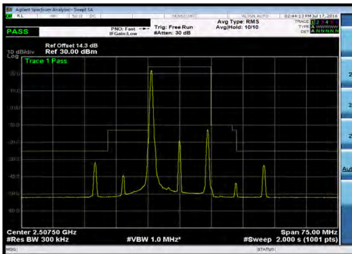
Emission Mask_Band 7_15M_QPSK_LOW_RB1,0
