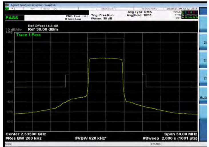
Emission Mask_Band 7_10M_16QAM_MID_RB50,0
