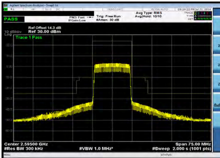
Emission Mask_Band 38_15M_QPSK_MID_RB75,0
