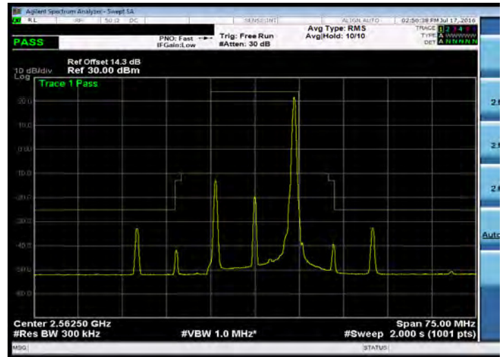
Emission Mask_Band 7_15M_QPSK_HIGH_RB1,74
