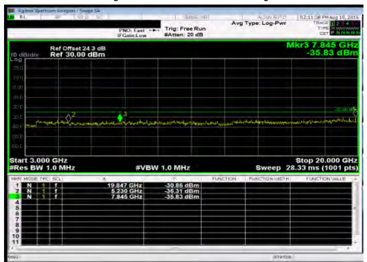
Out of Band Emission High_Band38 10MHz_QPSK 1_0_HighCH38200-2615
