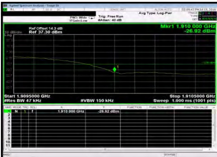
Band Edge_HSUPA_B2_HighCH9538-1907.6
