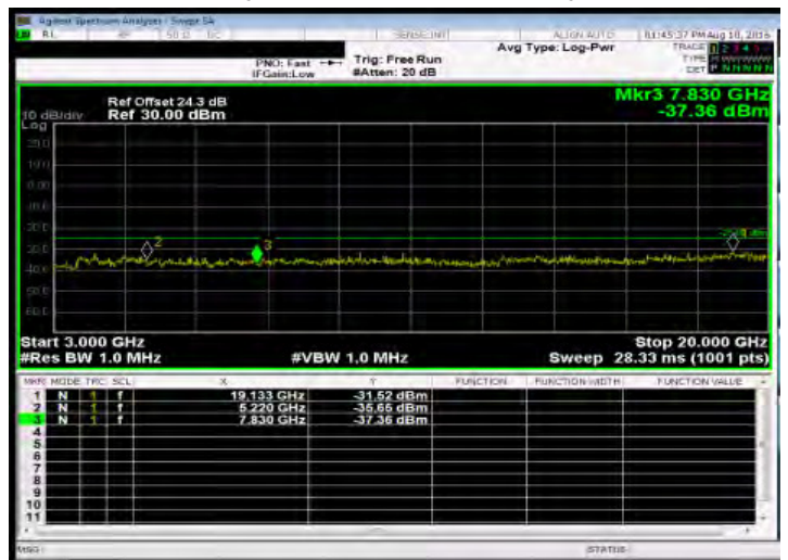
Out of Band Emission High_Band38 20MHz_QPSK 1 0_HighCH38150-2610
