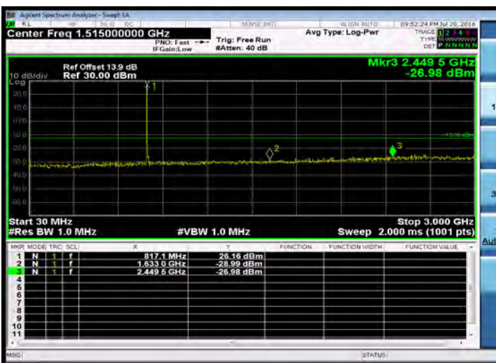
Out of Band Emission_Band26 for Part 90S_5M-QPSK-1 0-LOW-30M-3G
