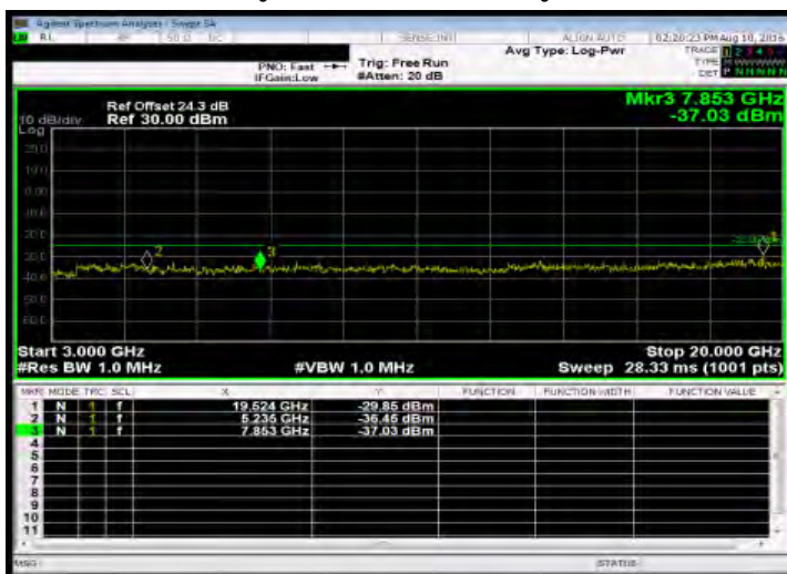
Out of Band Emission High_Band38 5MHz_QPSK 1_0_HighCH38225-2617.5
