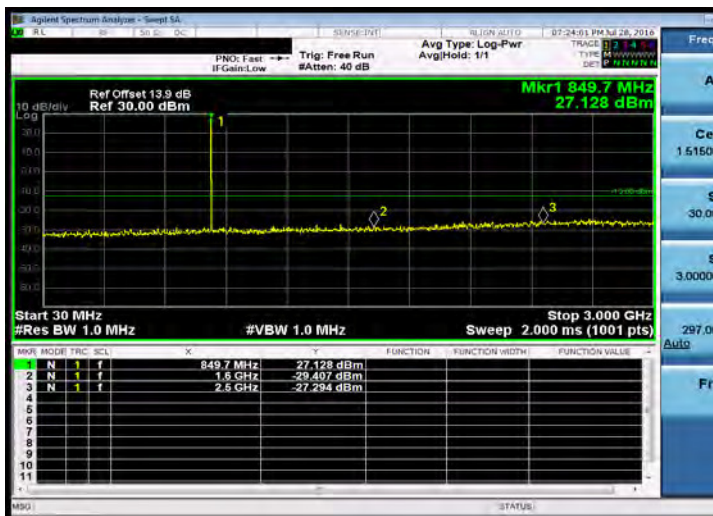
Out of Band Emission Low_Band26 1.4MHz_QPSK 1 0_HighCH27033-848.3
