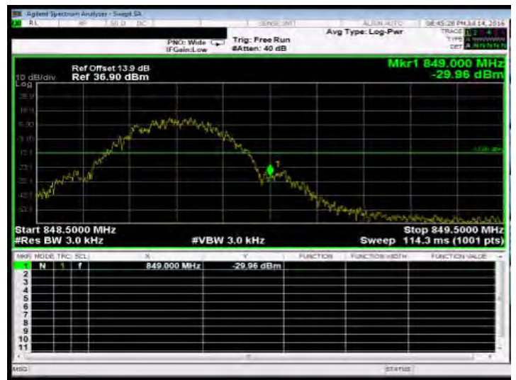
Band Edge_GPRS_850MHz_HighCH251-848.8
