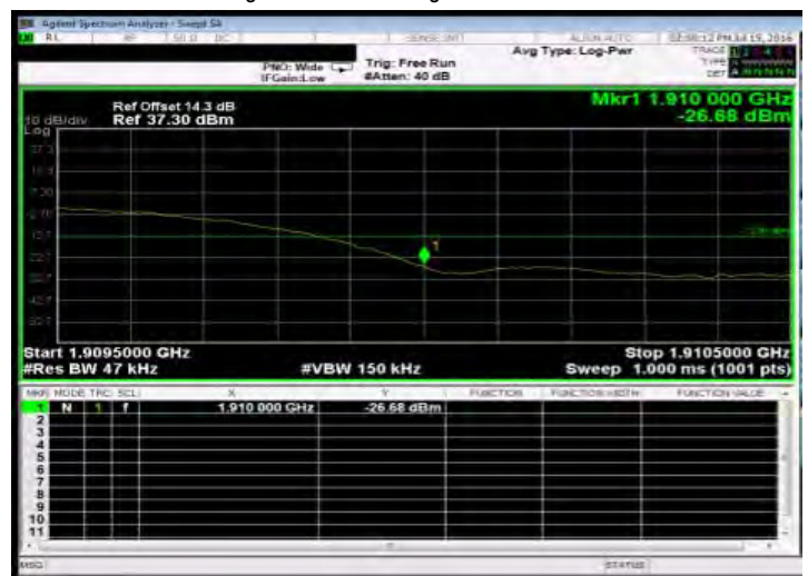
Band Edge_HSDPA_B2_HighCH9538-1907.6
