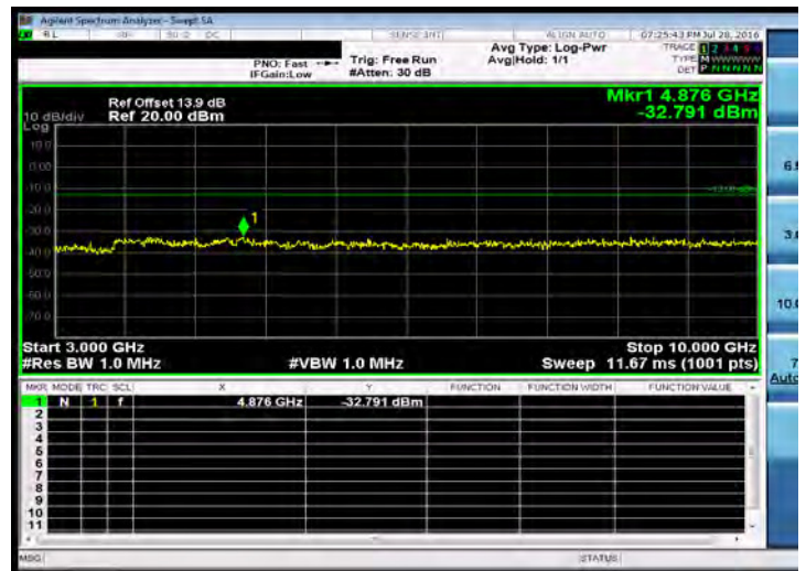
Out of Band Emission High_Band26 1.4MHz_QPSK 1 0_LowCH26797-824.7
