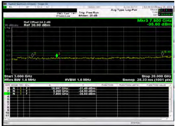
Out of Band Emission High_Band41 20MHz_QPSK 1 0_MidCH40690-2600
