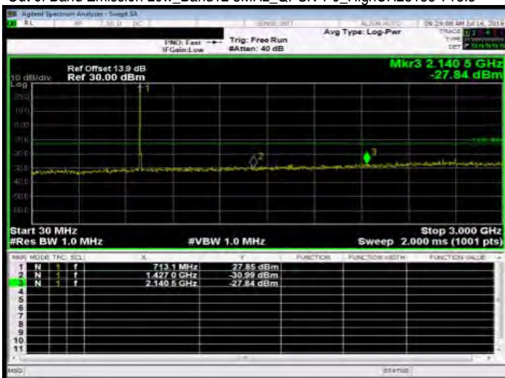
Out of Band Emission Low_Band12 5MHz_QPSK 1_0_HighCH23155-713.5
