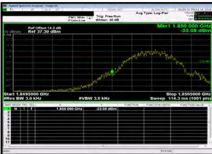
Band Edge_GSM_1900MHz_LowCH512-1850.2
