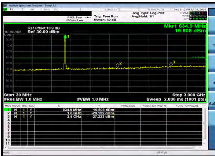
Out of Band Emission Low_Band26 15MHz_QPSK 1 0_Low
