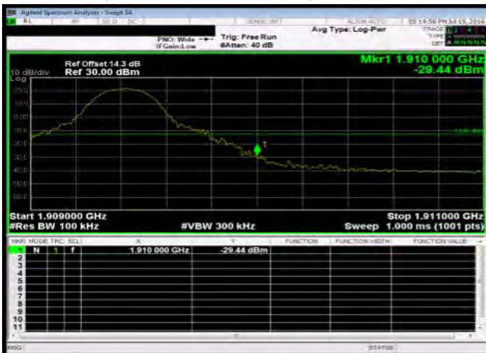
Band Edge_Band2 10MHz_QPSK 1 49_HighCH19150-1905
