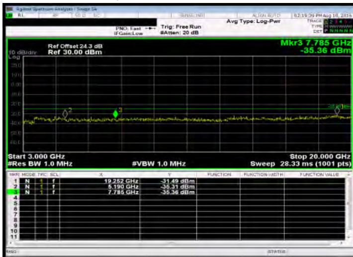
Out of Band Emission High_Band38 5MHz_QPSK 1_0_MidCH38000-2595
