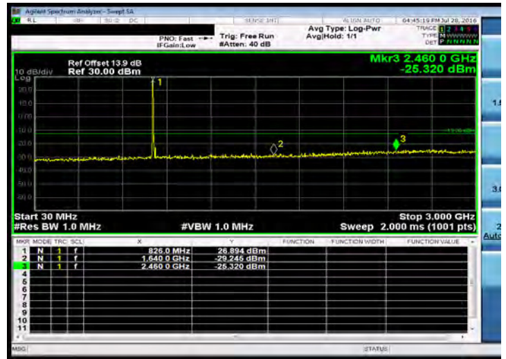
Out of Band Emission Low_Band26 10MHz_QPSK 1 0_MidCH26915-836.5
