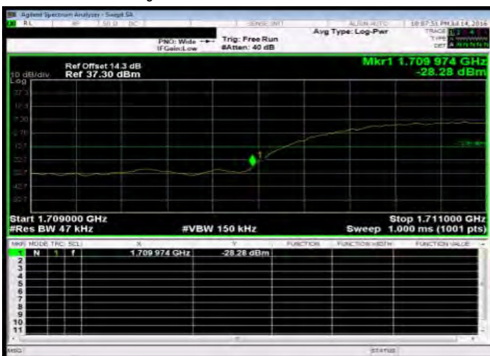
Band Edge_WCDMA_B4_LowCH1312-1712.4
