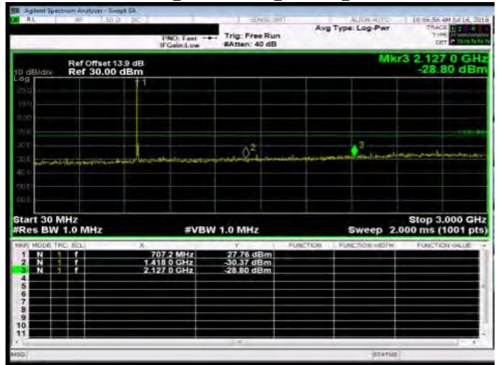
Out of Band Emission Low_Band17 10MHz_QPSK 1_0_MidCH23790-710
