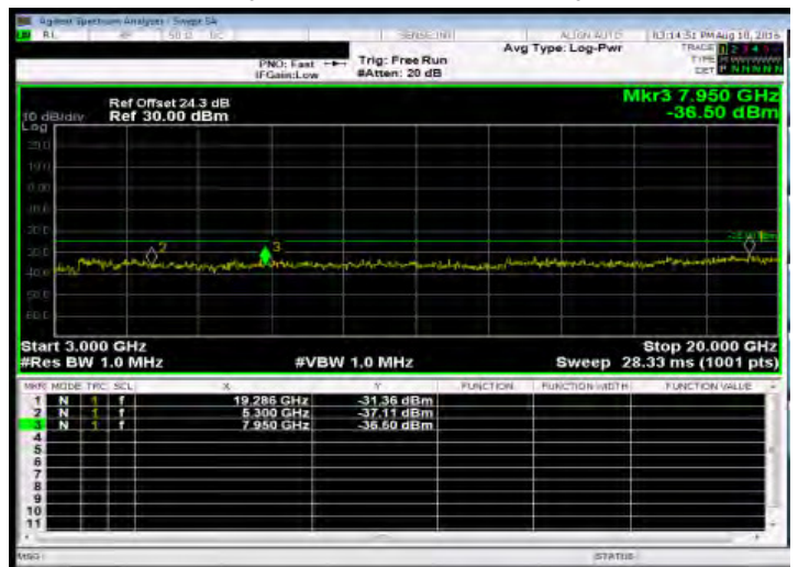
Out of Band Emission High_Band41 10MHz_QPSK 1 0_HighCH41190-2650
