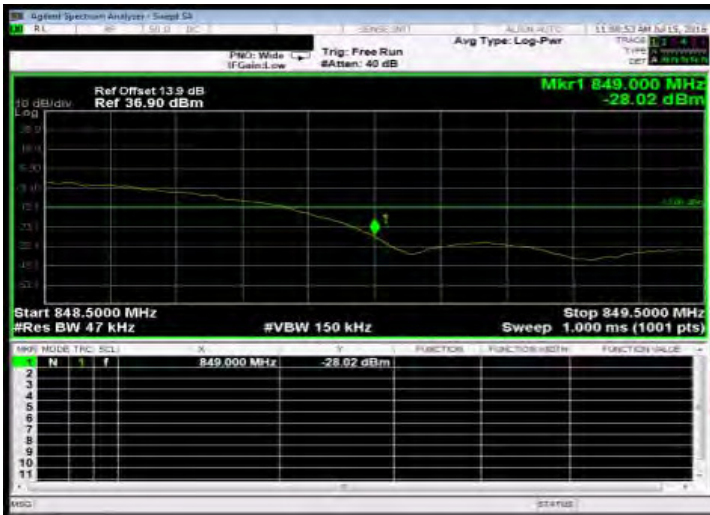
Band Edge_HSUPA_B5_HighCH4233-846.6
