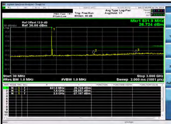
Out of Band Emission Low_Band26 15MHz_QPSK 1 0_Mid
