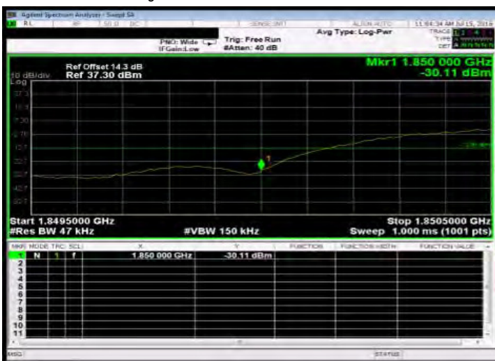
Band Edge_WCDMA_B2_LowCH9262-1852.4
