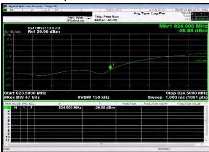
Band Edge_WCDMA_B5_LowCH4132-826.4
