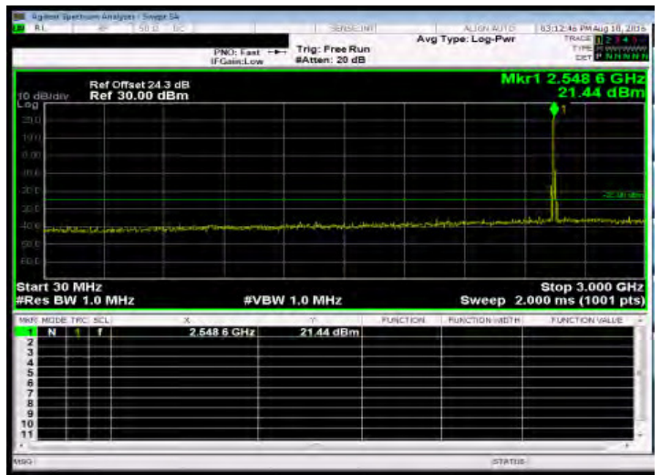
Out of Band Emission Low_Band41 10MHz_QPSK 1 0_MidCH40690-2600
