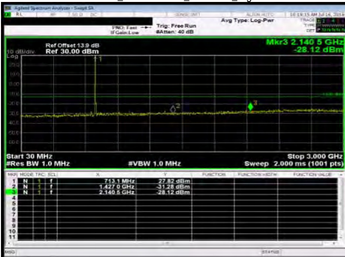
Out of Band Emission Low_Band17 5MHz_QPSK 1_0_HighCH23825-713.5
