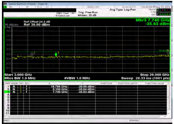
Out of Band Emission High_Band38 20MHz_QPSK 1 0_MidCH38000-2595
