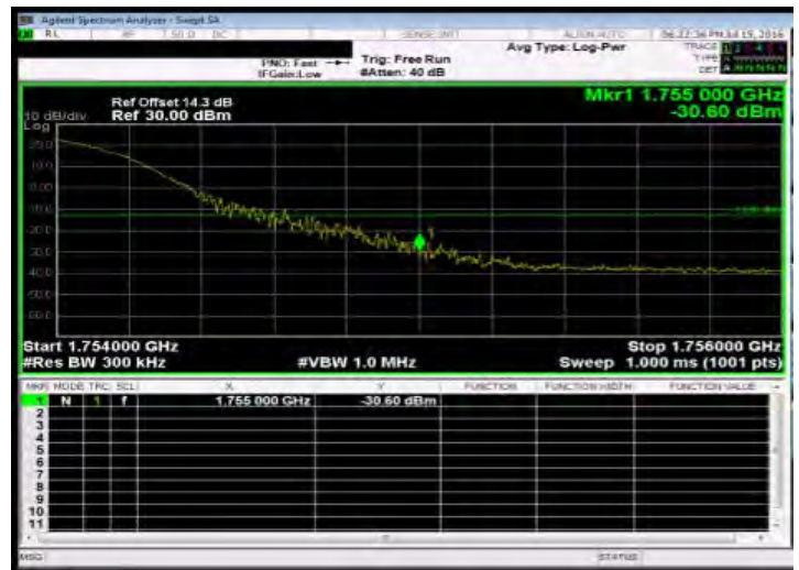
Band Edge_Band4 20MHz_QPSK 1 99_HighCH20300-1745
