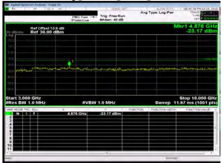
Out of Band Emission High_Band5 3MHz_QPSK 1 0_MidCH20525-836.5
