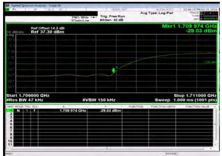
Band Edge_HSDPA_B4_LowCH1312-1712.4
