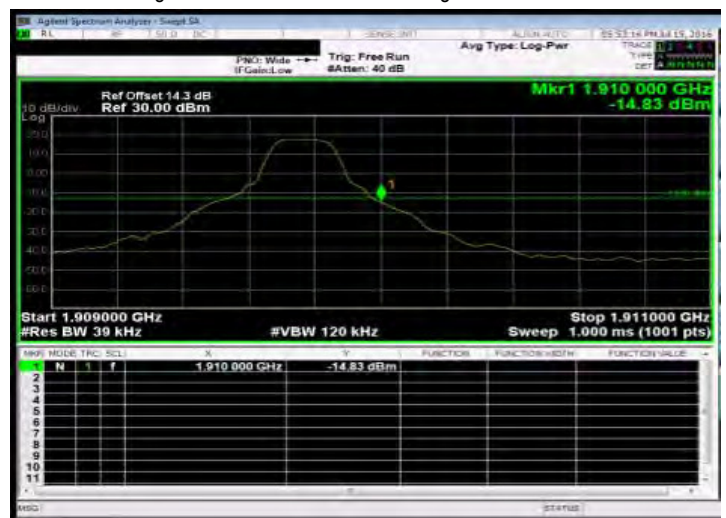
Band Edge_Band2 3MHz_QPSK 1 14_HighCH19185-1908.5
