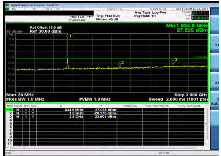
Out of Band Emission Low_Band26 10MHz_QPSK 1 0_HighCH26990-844
