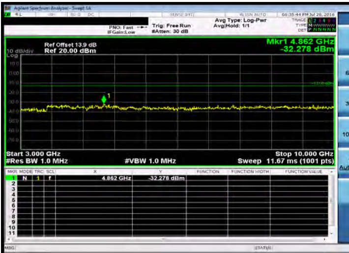
Out of Band Emission High_Band26 3MHz_QPSK 1 0_HighCH27025-847.5
