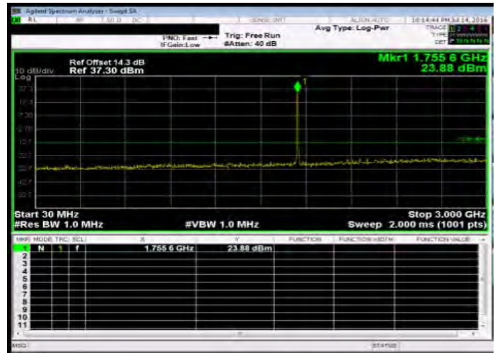
Out of Band Emission Low_WCDMA_B4_HighCH1513-1752.6
