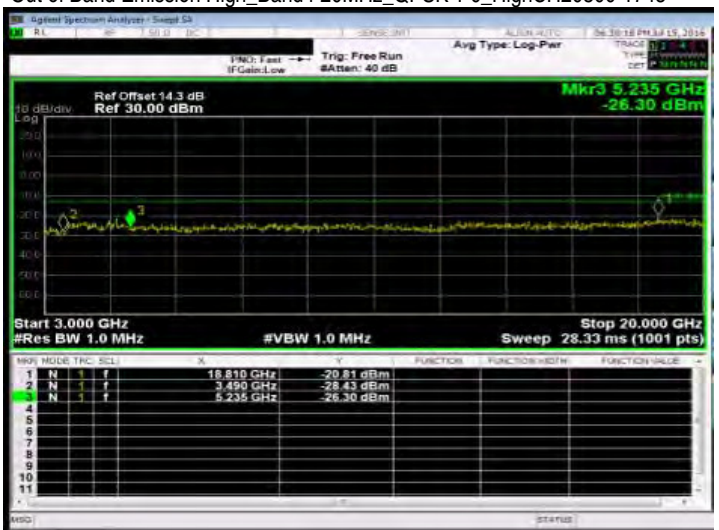
Out of Band Emission High_Band4 20MHz_QPSK 1 0_HighCH20300-1745
