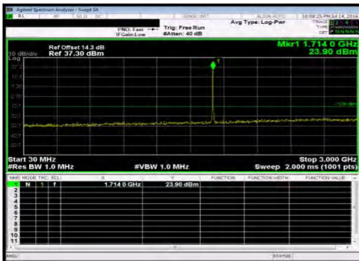
Out of Band Emission Low_WCDMA_B4_LowCH1312-1712.4
