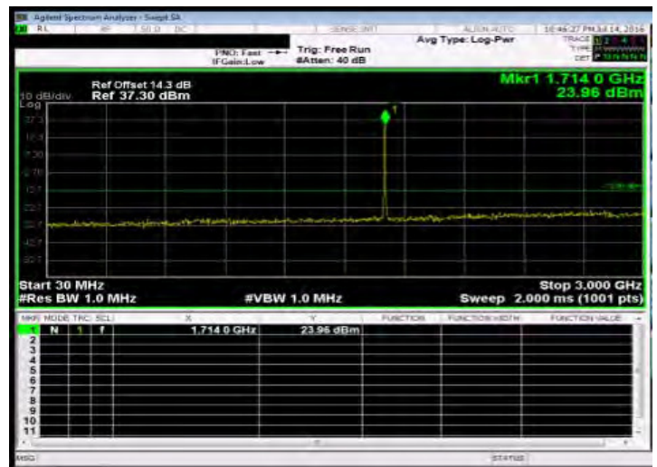
Out of Band Emission Low_HSDPA_B4_LowCH1312-1712.4
