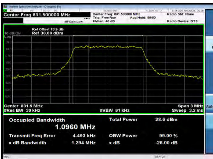
LTE Band 26 for Part 90S_1.4M_16QAM_HIGH
