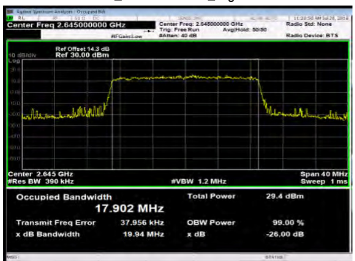
Band41 20MHz_16-QAM 100 0_HighCH41140-2645
