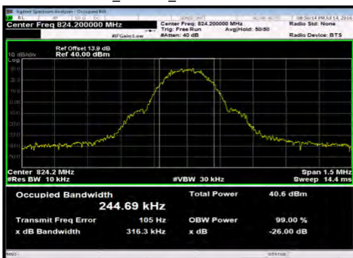
EDGE_850MHz_LowCH128-824.2
