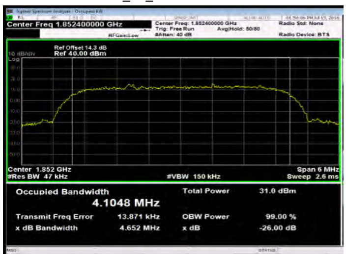
HSDPA_B2_LowCH9262-1852.4
