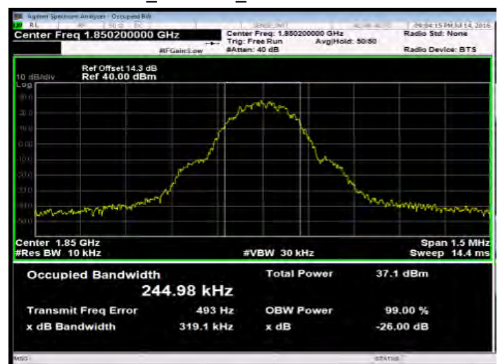
GSM_1900MHz_LowCH512-1850.2
