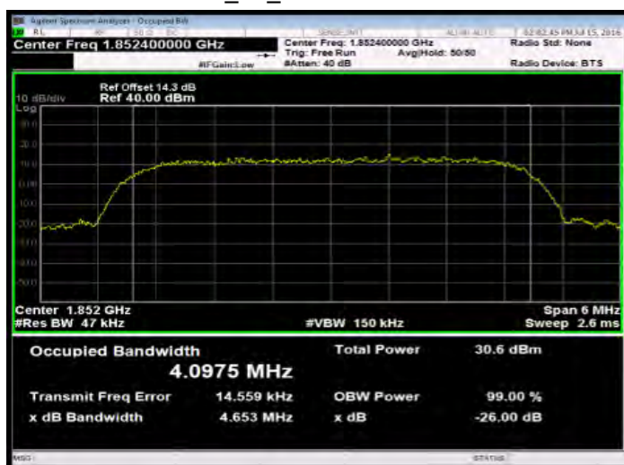
HSUPA_B2_LowCH9262-1852.4
