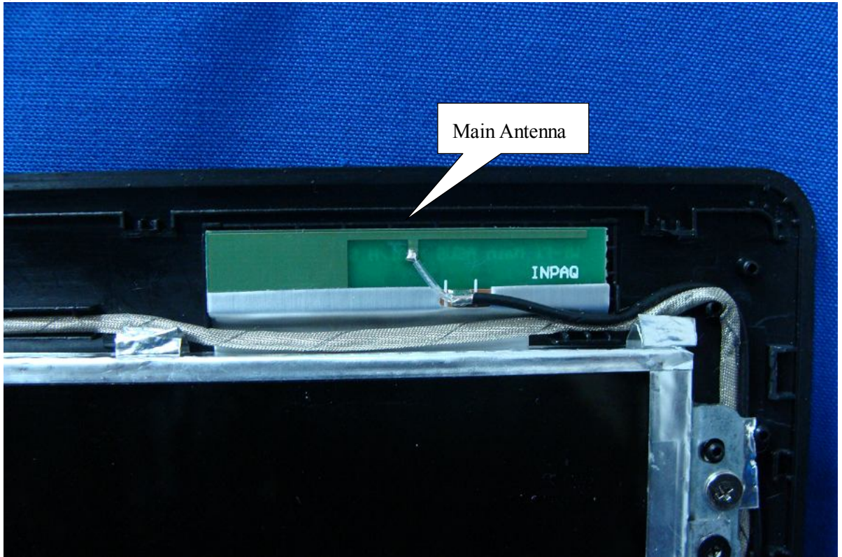
(18) EUT Photo (INPAQ Antenna)
