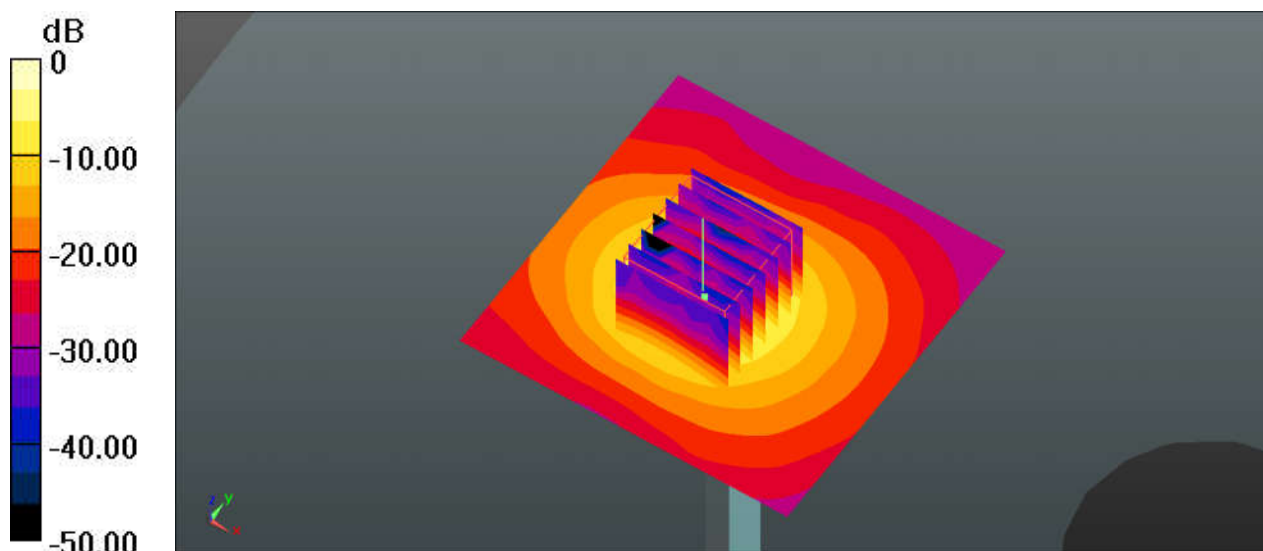
0 dB = 19.3 W/kg
