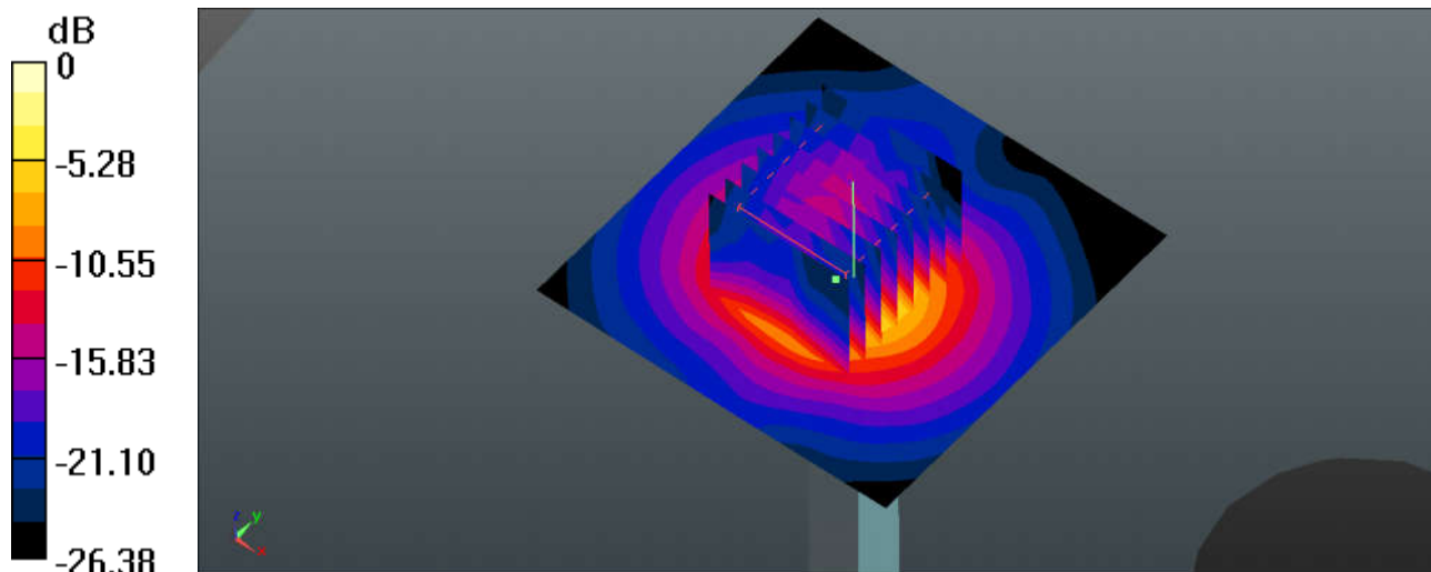
0 dB = 17.5 W/kg
