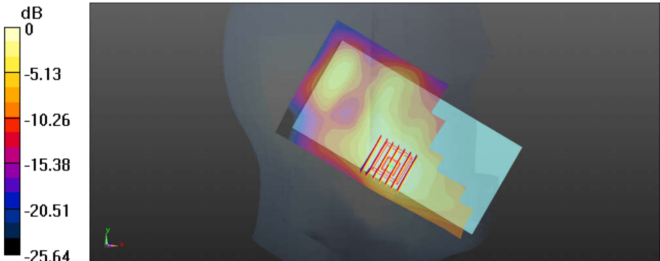
0 dB = 0.714 W/kg
