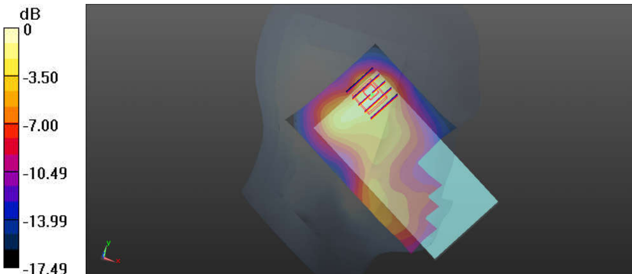
0 dB = 0.140 W/kg
