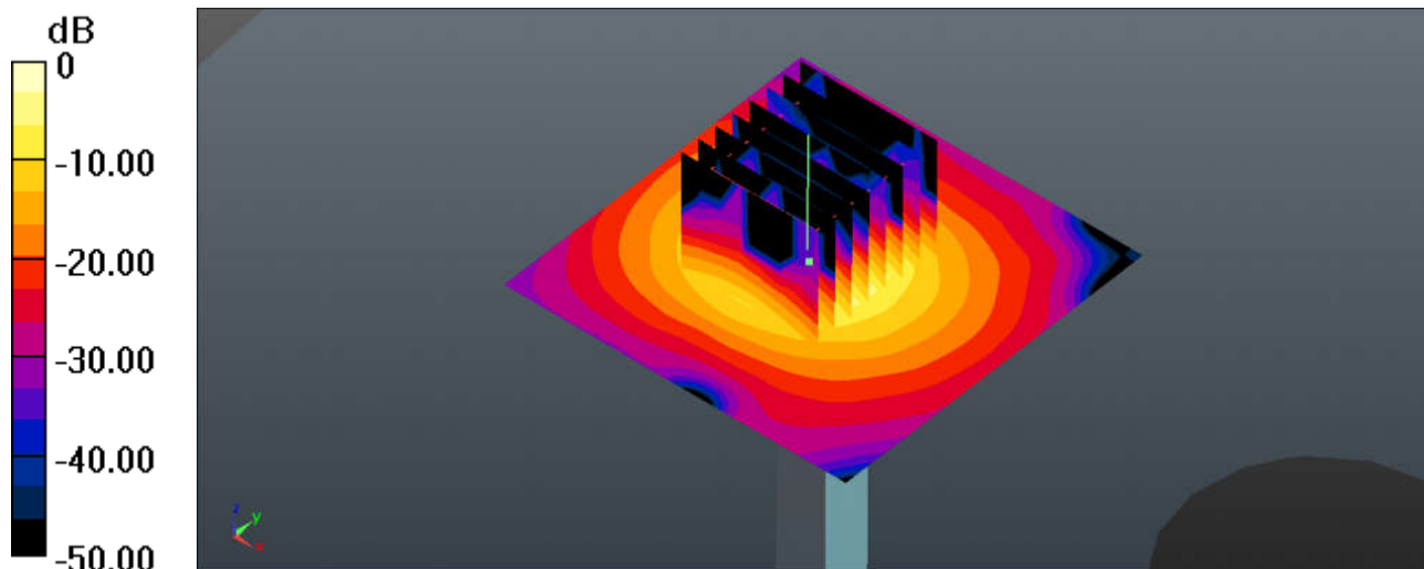
0 dB = 18.2 W/kg
