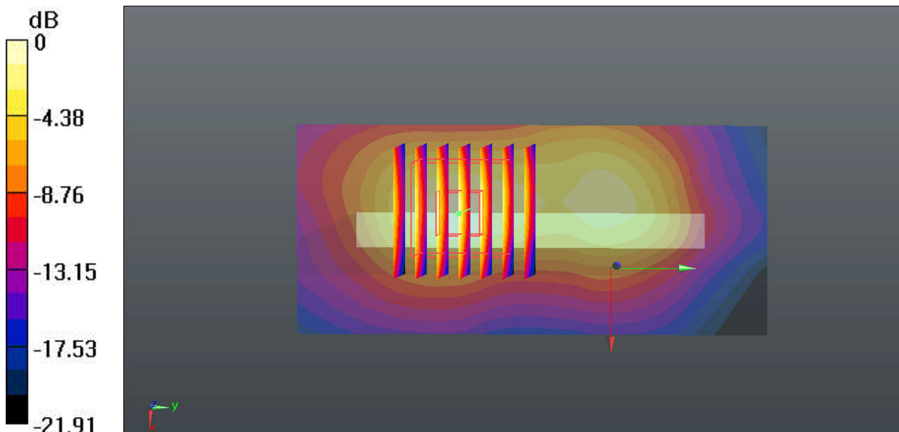
0 dB = 0.960 W/kg
