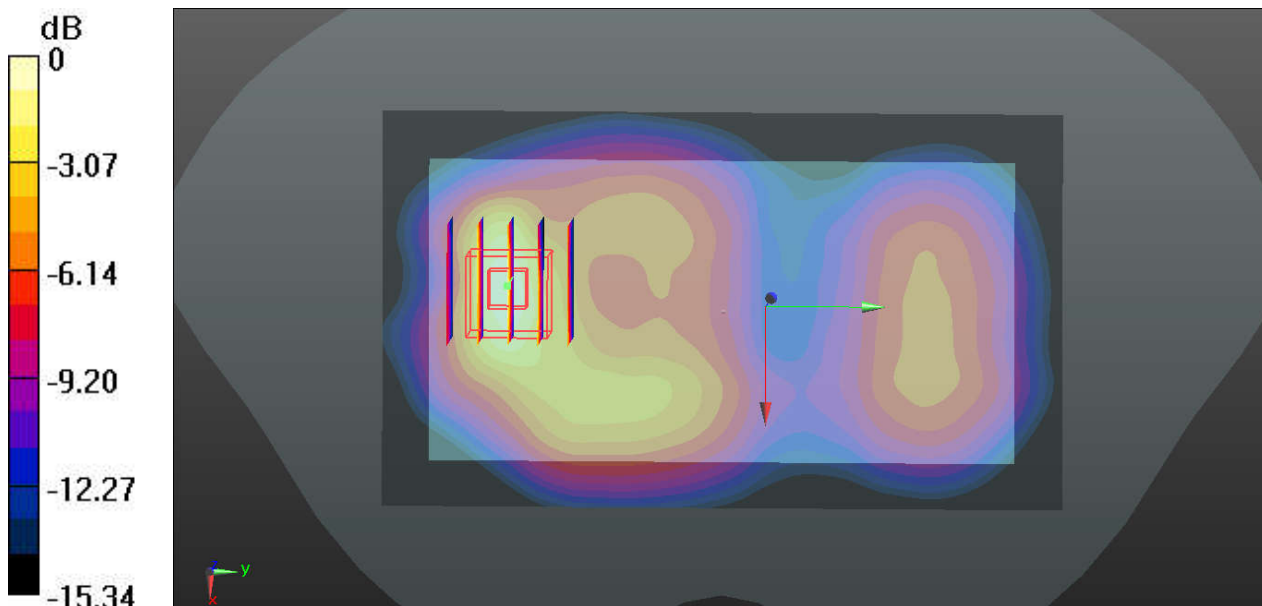
0 dB = 0.891 W/kg
