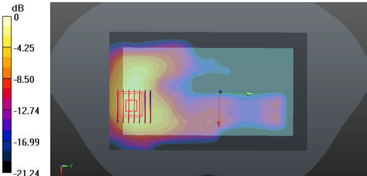
0 dB = 0.482 W/kg
