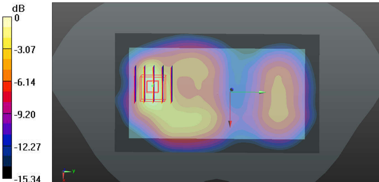
0 dB = 0.891 W/kg
