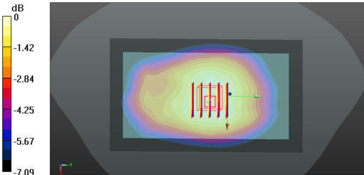
0 dB = 0.536 W/kg
