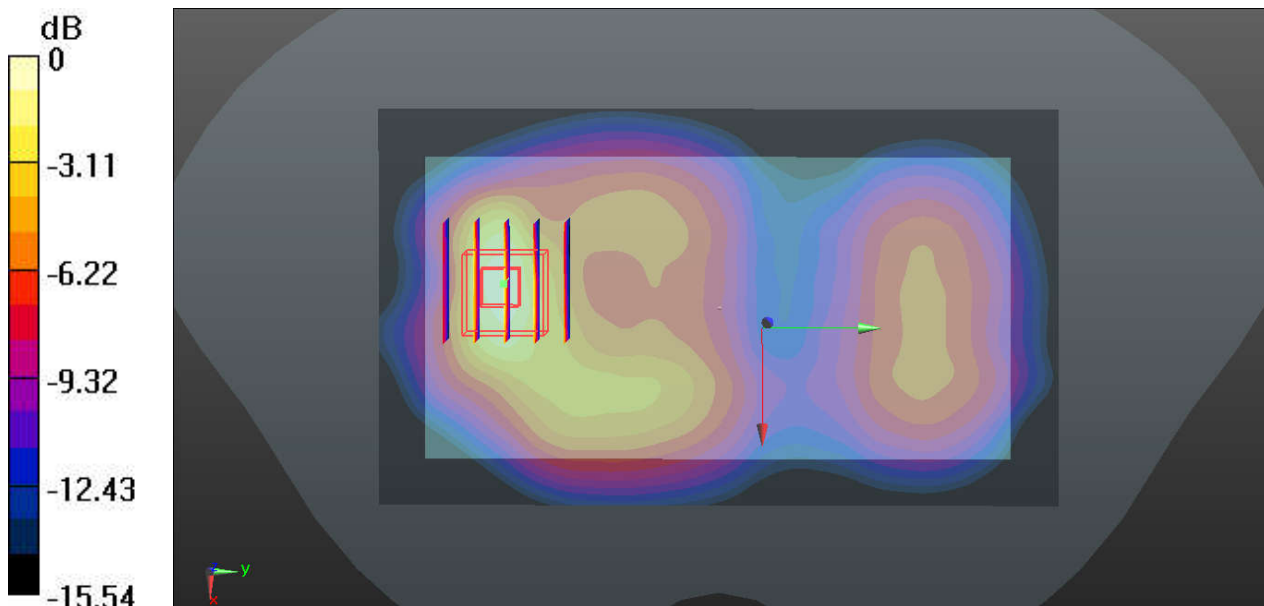
0 dB = 0.863 W/kg
