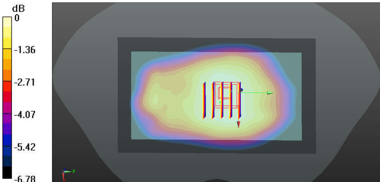
0 dB = 0.601 W/kg
