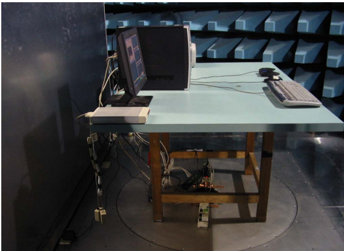
Side View of the Test Configuration
