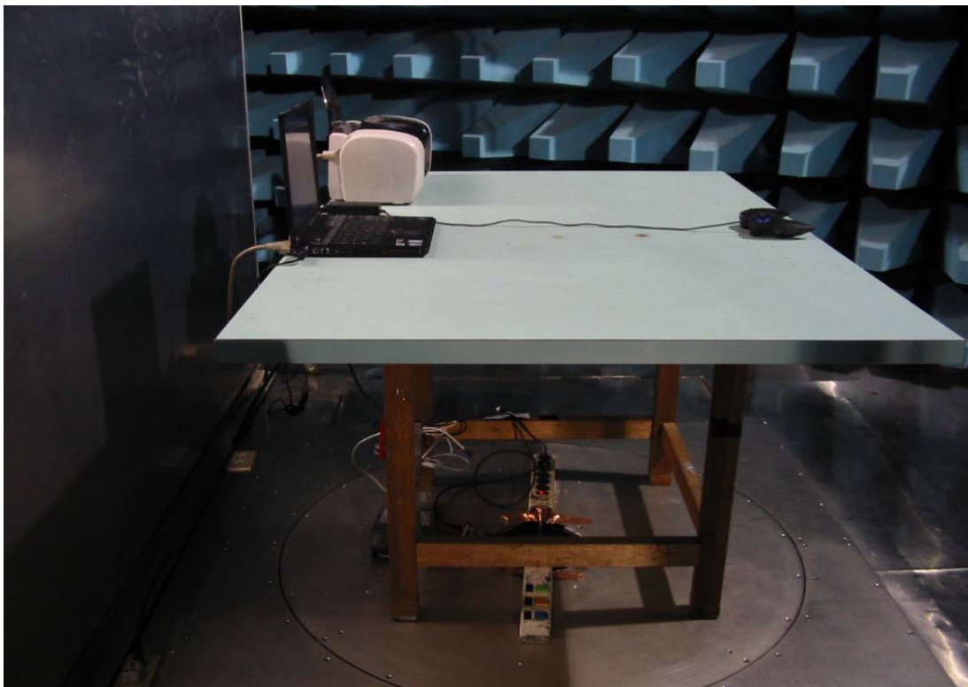
Side View of the Test Configuration
