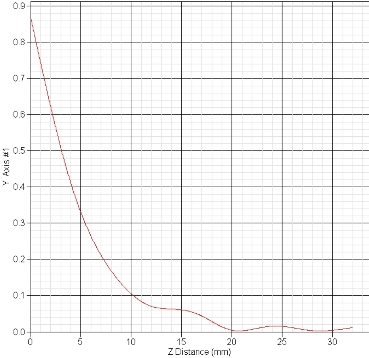
SAR-Z Axis at Hotspot x:16.00 y:15.90
