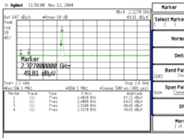
Figure Channel 00: (Horizontal)
