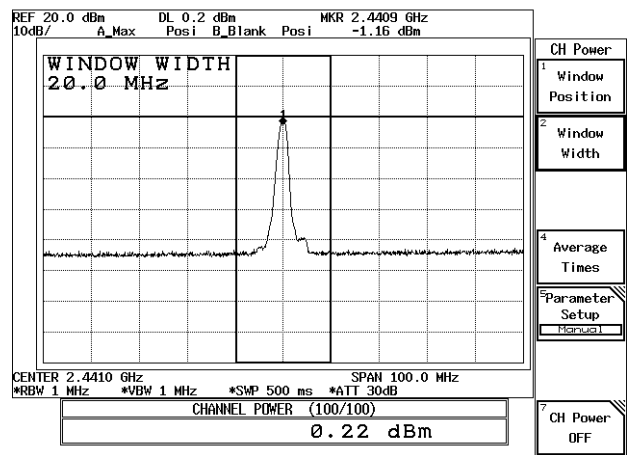
Channel 39
