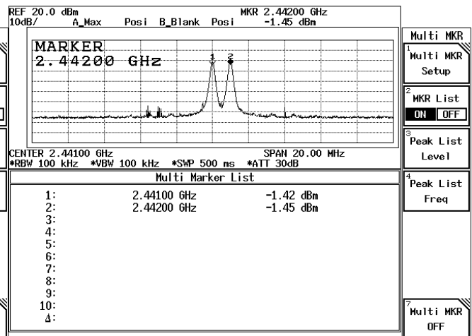
Channel 39 2441MHz
