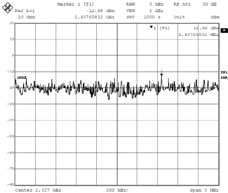
Figure Channel 6: 11Mbps
