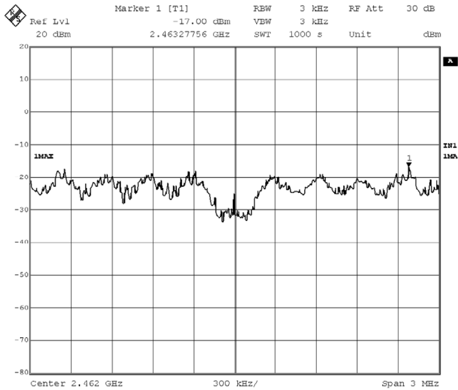
Figure Channel 11: 54Mbps
