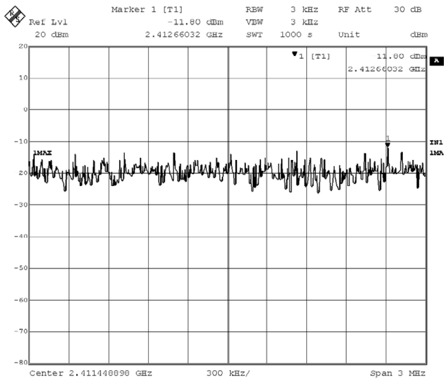
Figure Channel 1: 11Mbps
