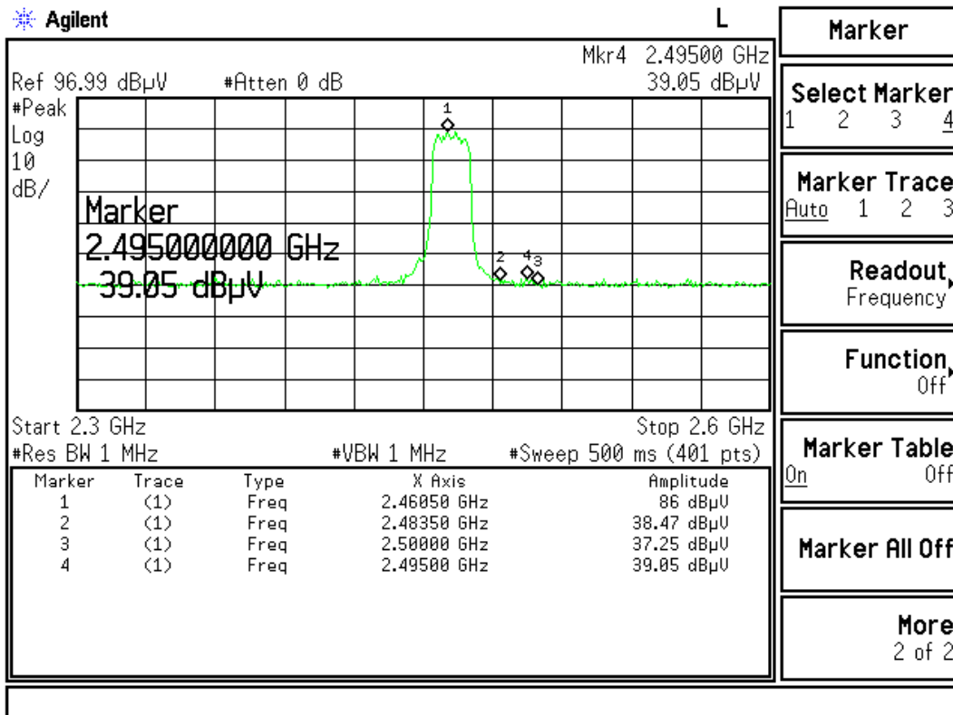
Figure Channel 11: (Horizontal)
