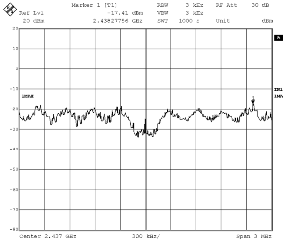
Figure Channel 6: 54Mbps
