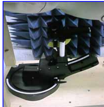
Figure 6. Device Holder
