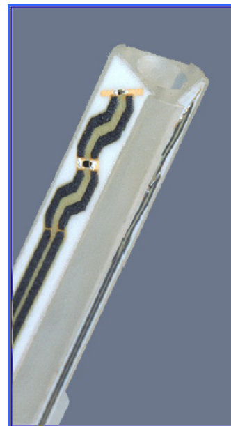
Figure 4. ET3DV6 E-field Probe
