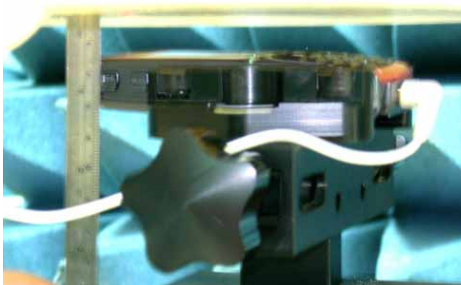
Figure 18. Body SAR Test Setup (Flat Section)
