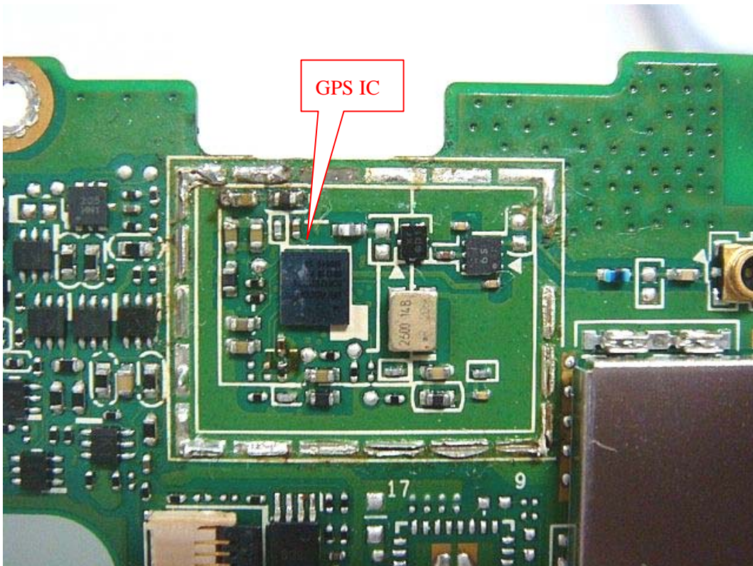
(30) EUT Photo (GPS)
