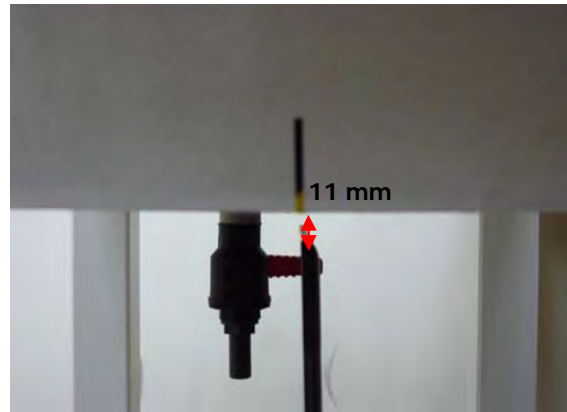
Fig.7 EUT Secondary Landscape mode to flat phantom (Test distance is 11 mm)
