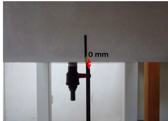
Fig.5 EUT Primary Portrait mode to flat phantom (Test distance is 0 mm)
