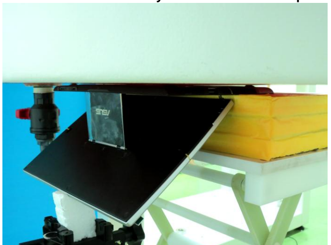
Laptop Mode – Rear Face of EUT with 0 cm Gap
