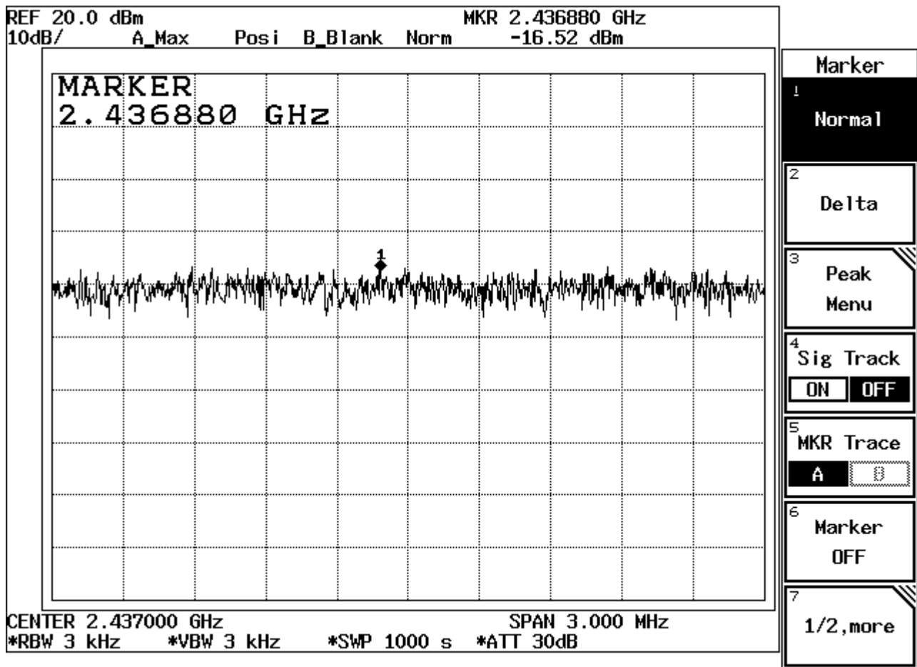
Figure Channel 6: 11Mbps
