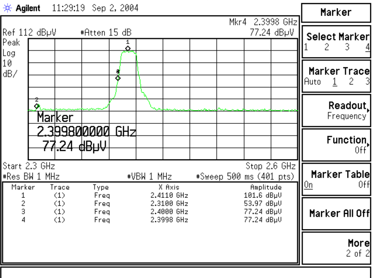
Figure Channel 1: (Horizontal)
