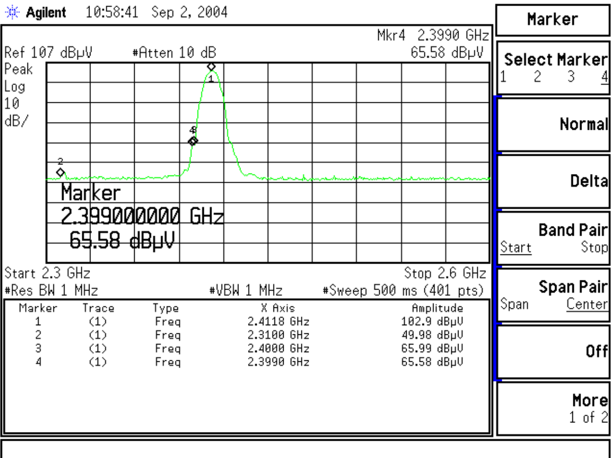
Figure Channel 1: (Vertical)
