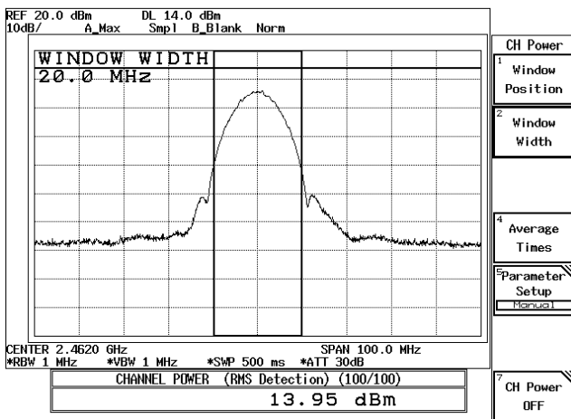
11Mbps-CH11
