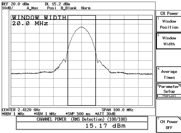
11Mbps-CH01
