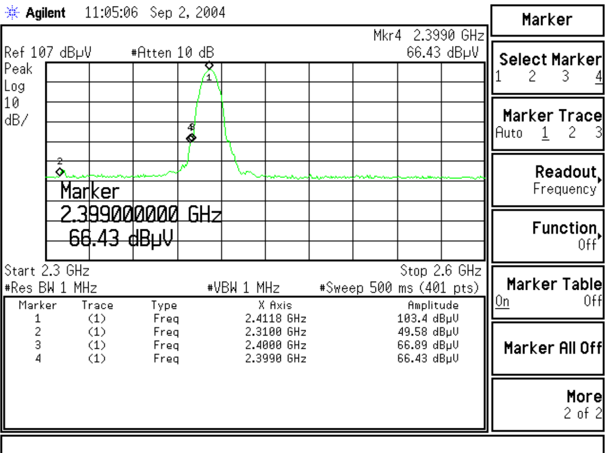
Figure Channel 1: (Horizontal)
