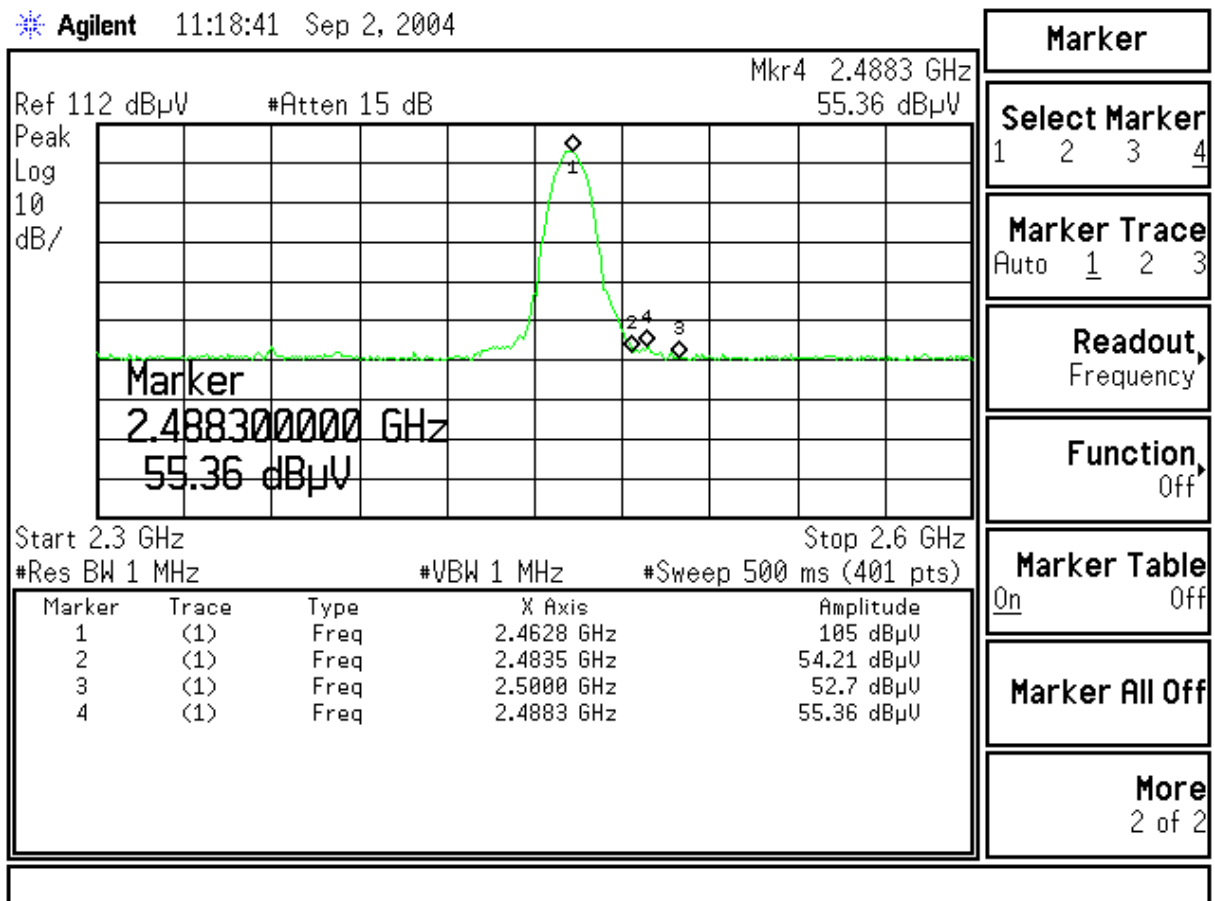
Figure Channel 11: (Vertical)
