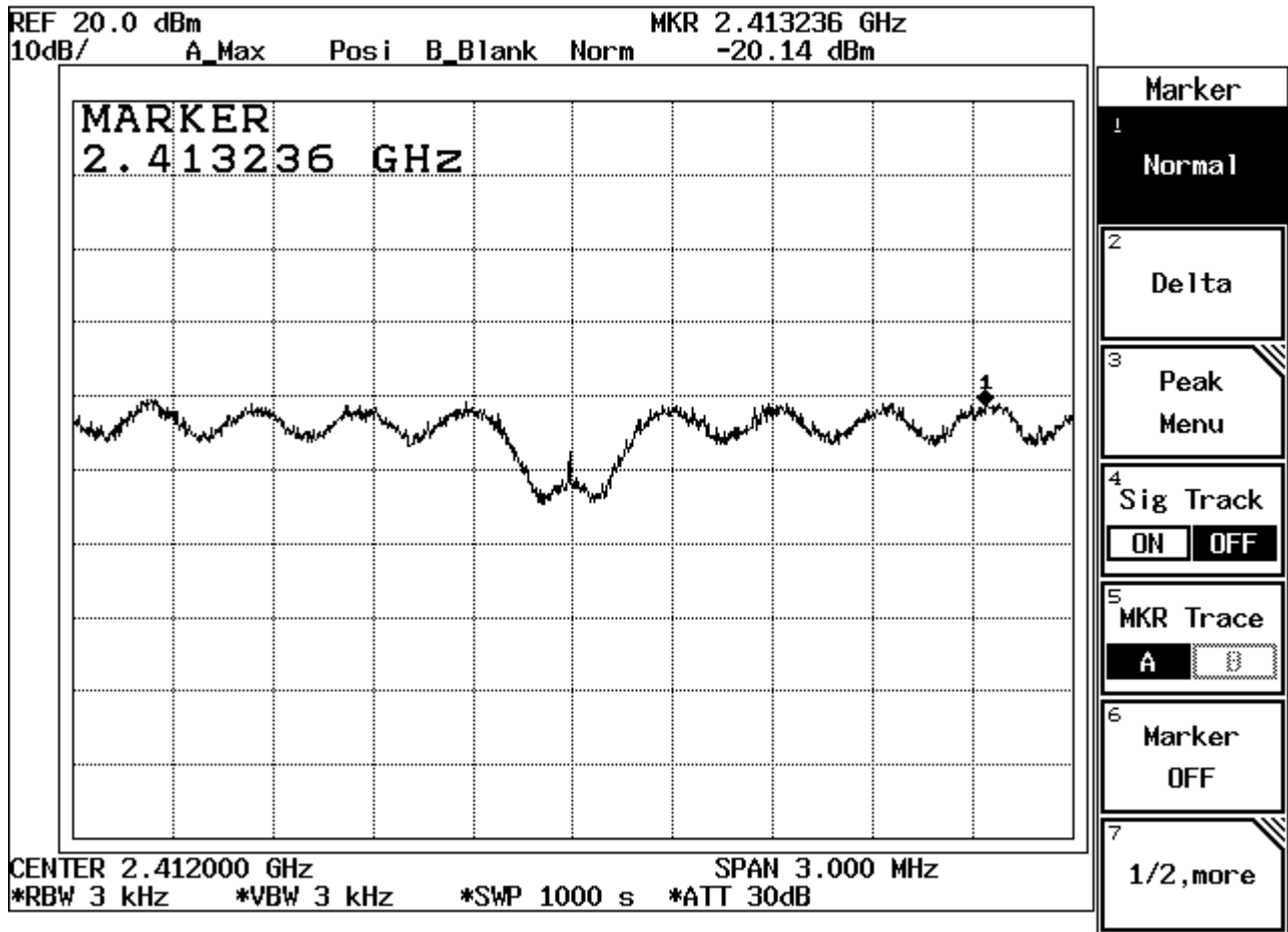
Figure Channel 1: 54Mbps
