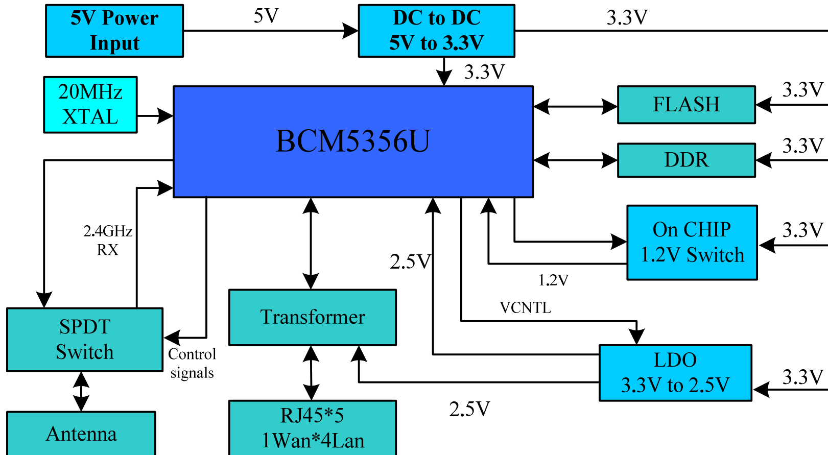
RT-N10U_BLACK Block Diagram
