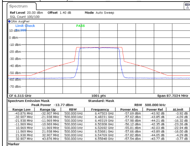
802.11ax (20MHz) 6515MHz Chain C NSS-1
