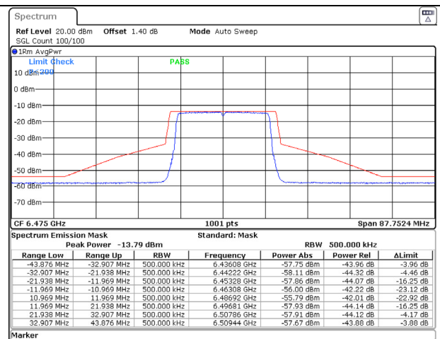
802.11ax (20MHz) 6475MHz Chain D NSS-1
