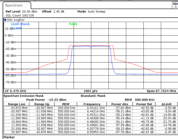
802.11ax (20MHz) 6475MHz Chain A NSS-1
