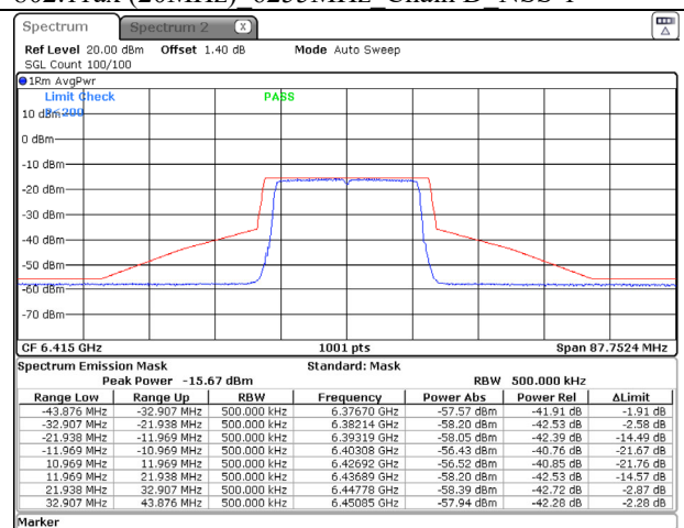
802.11ax (20MHz) 6415MHz Chain B NSS-1
