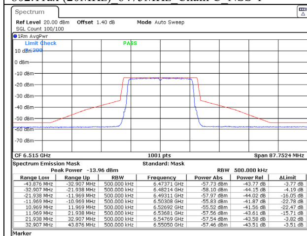
802.11ax (20MHz) 6515MHz Chain A NSS-1
