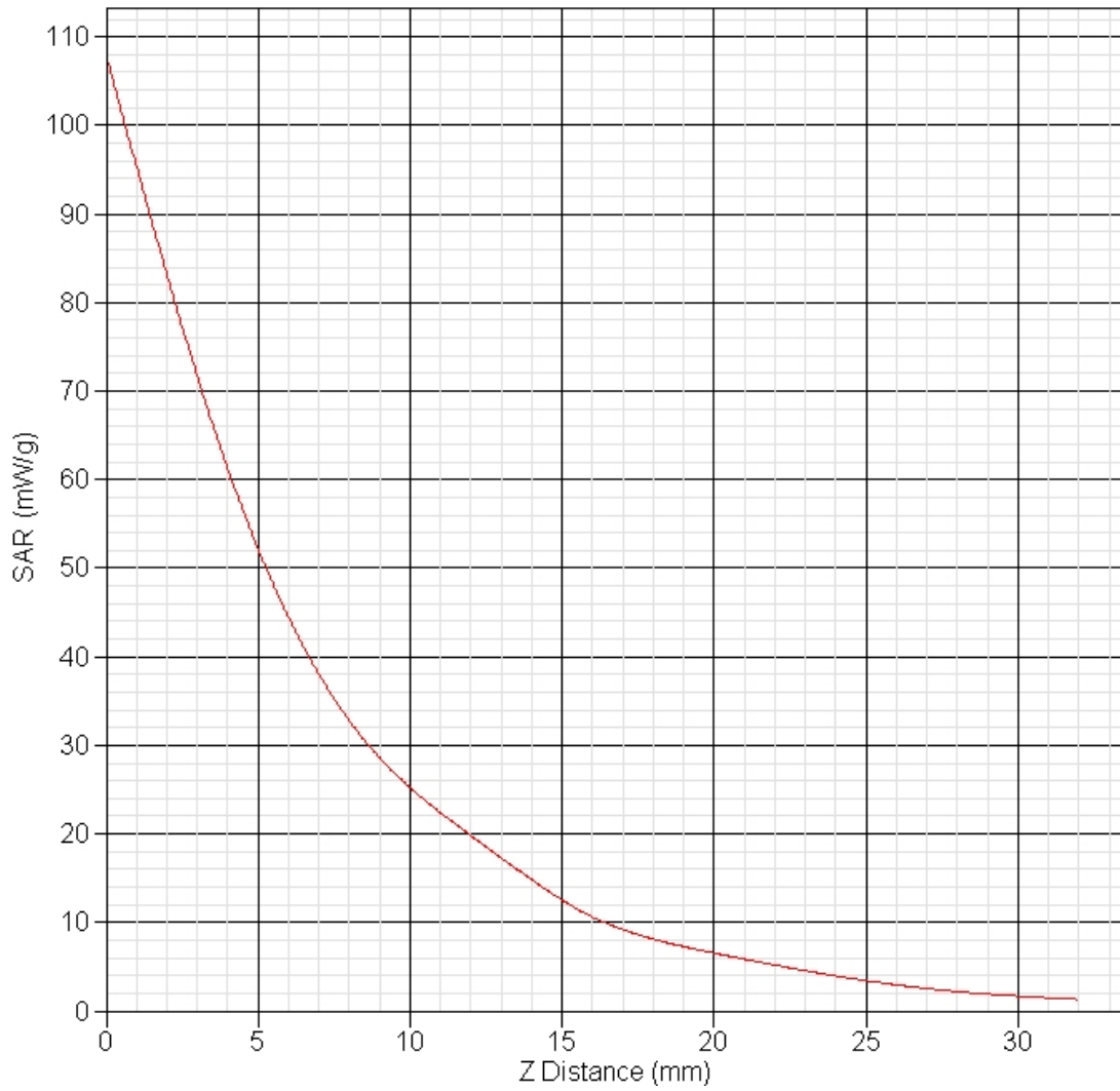
SAR-Z Axis at Hotspot x:0.09 y:-0.01
