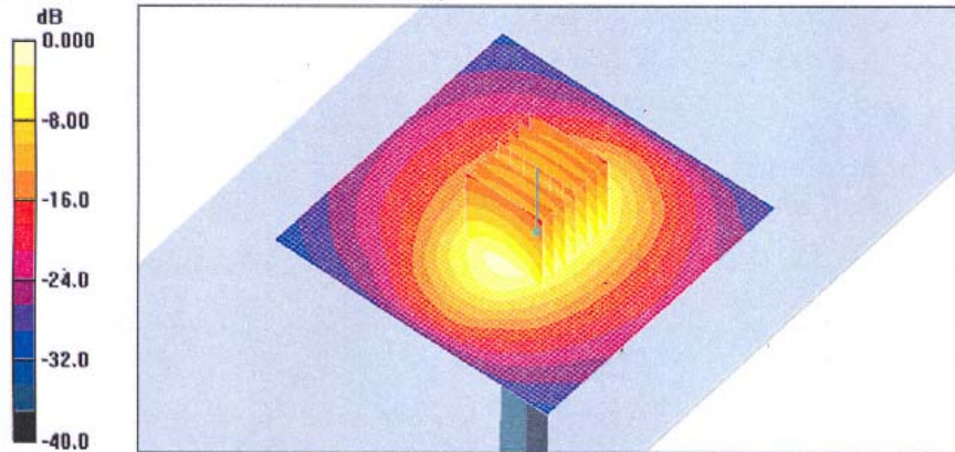
0 dB = 11.1mW/g
