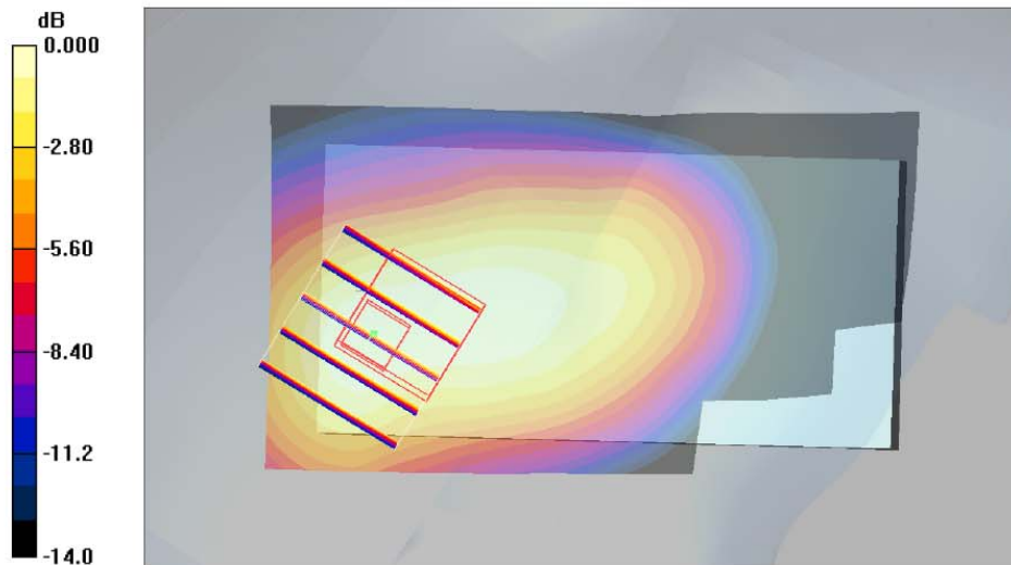
0 dB = 0.377mW/g
