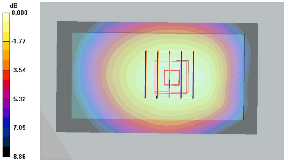
0 dB = 1.11mW/g
