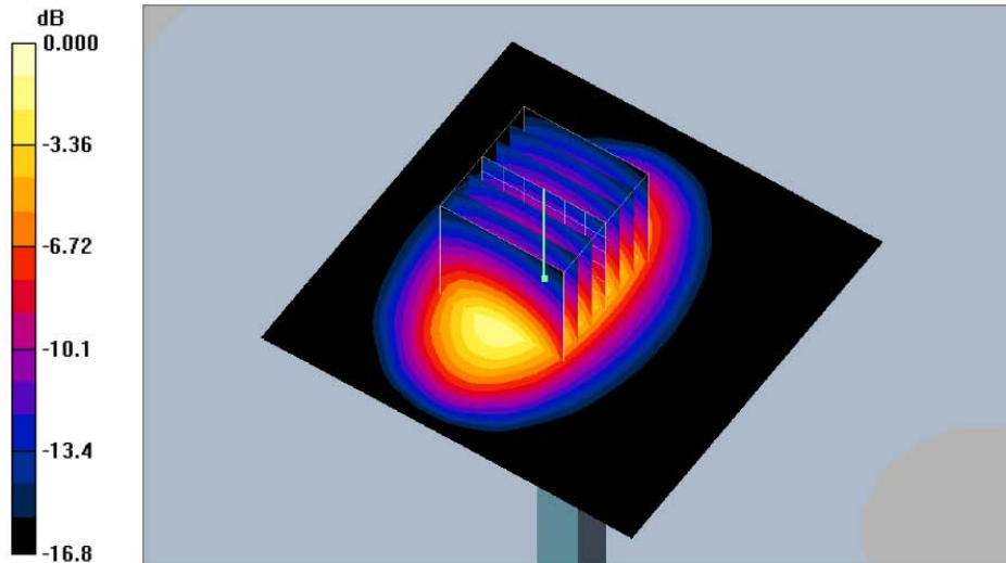
0 dB = 4.51mW/g
