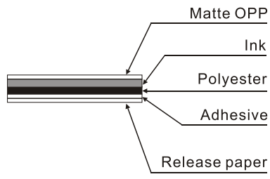
Material Composition Drawing
