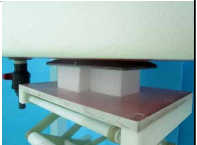
Rear Face of EUT with Cover 1 with 0 cm Gap
