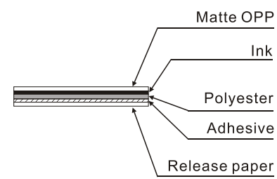
Material Composition Drawing
