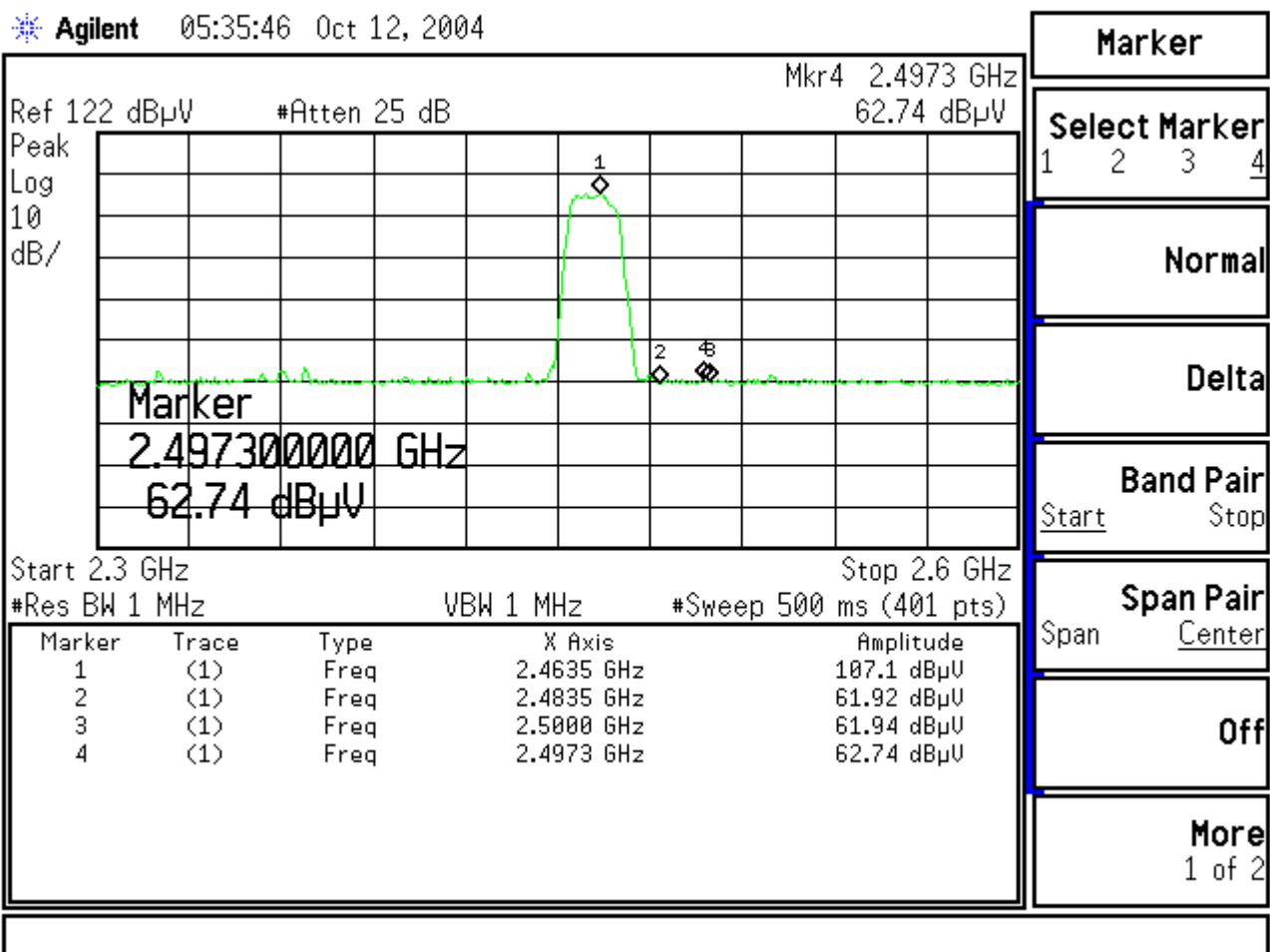
Figure Channel 11: (Vertical)
