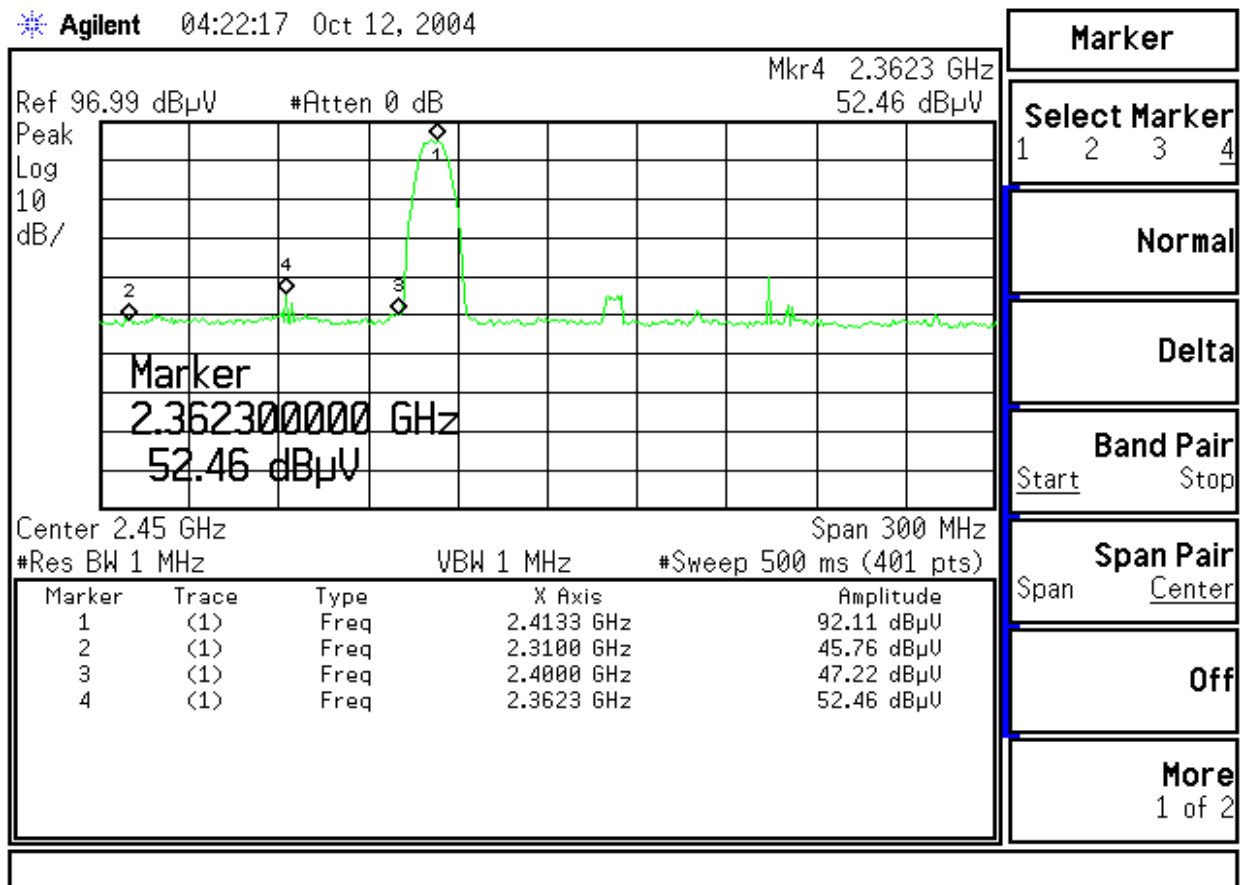
Figure Channel 1: (Horizontal)
