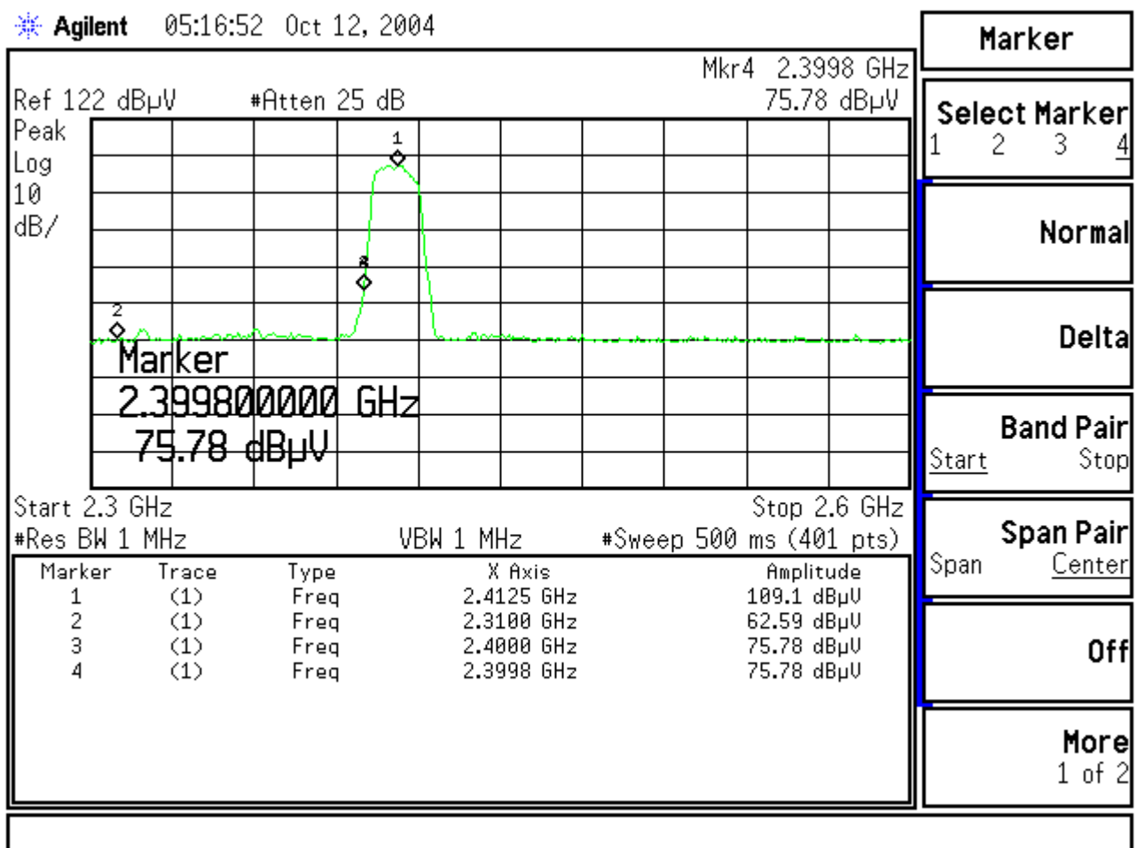
Figure Channel 1: (Vertical)
