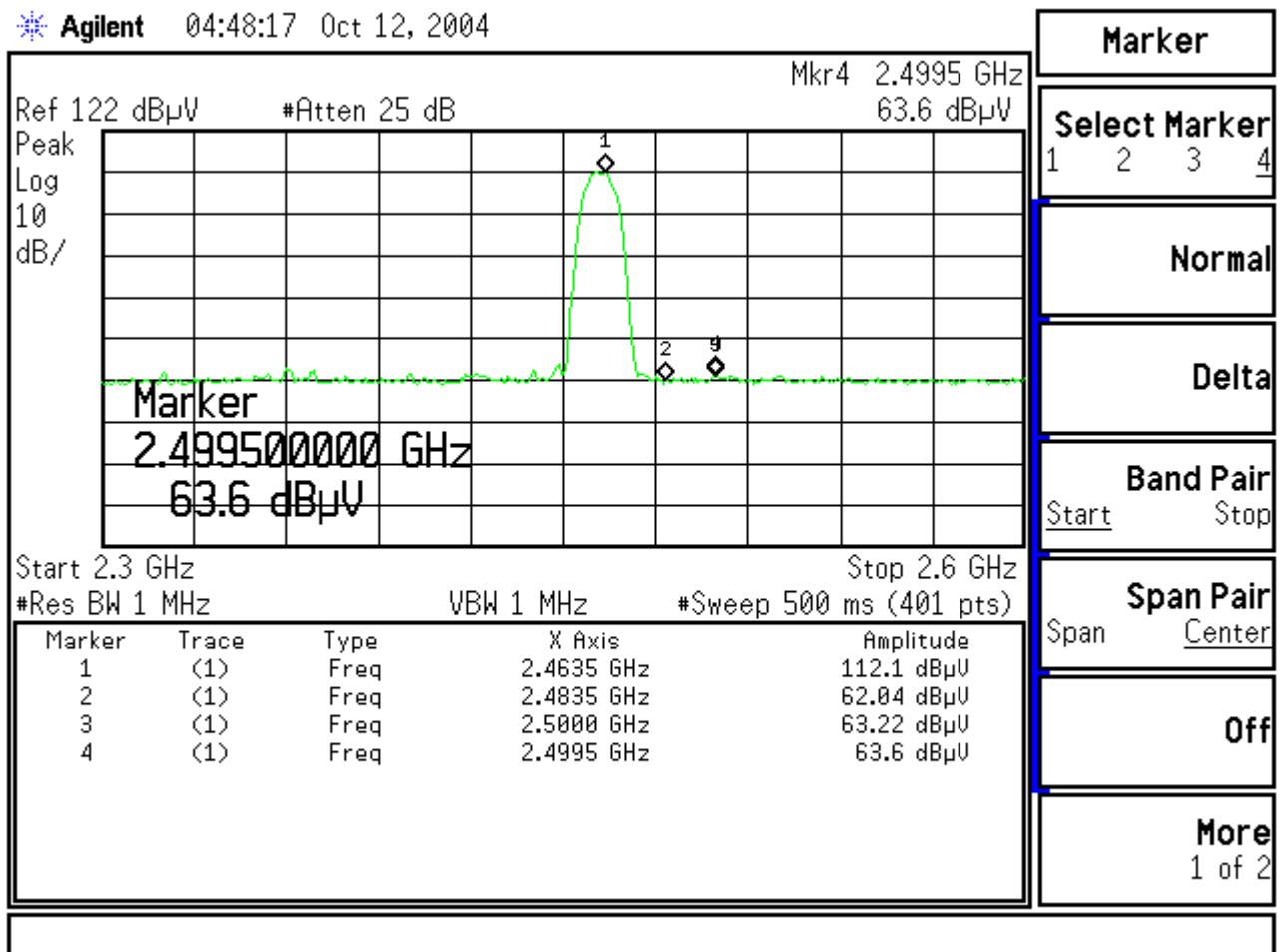
Figure Channel 11: (Vertical)
