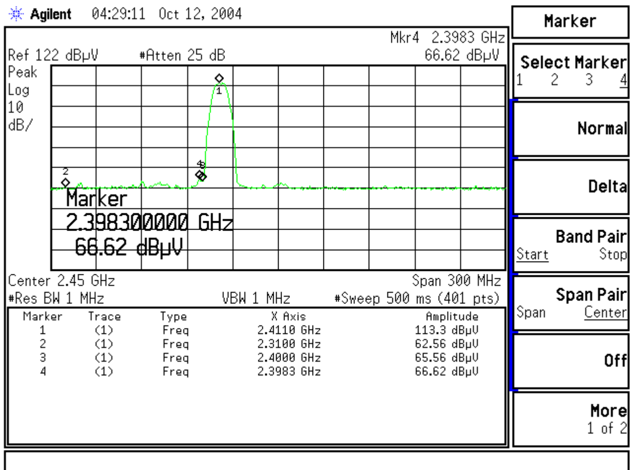
Figure Channel 1: (Vertical)
