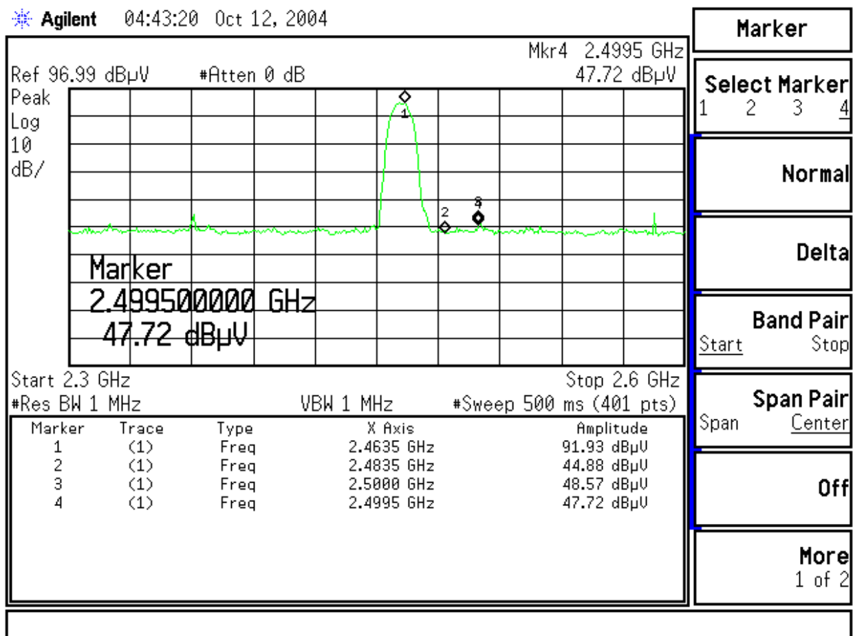
Figure Channel 11: (Horizontal)
