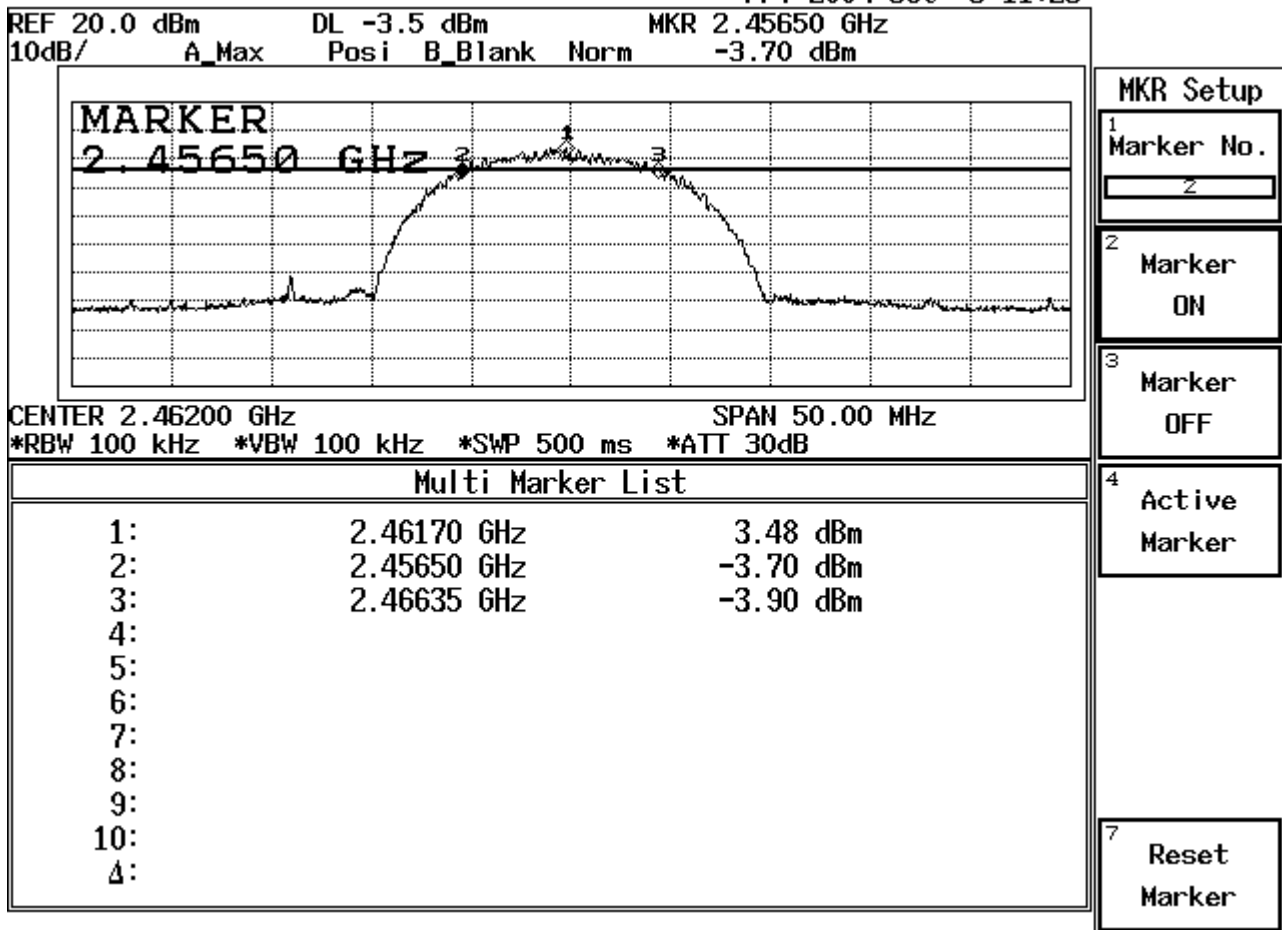
Figure Channel 11:
