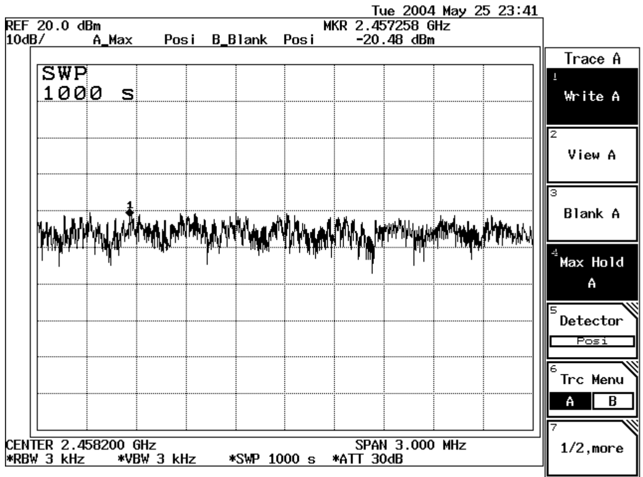
Figure Channel 11: 54Mbps
