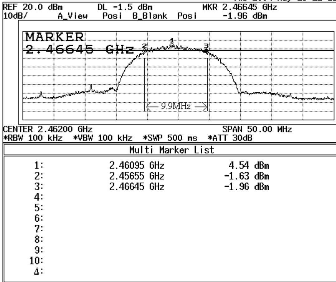
Figure Channel 11:
