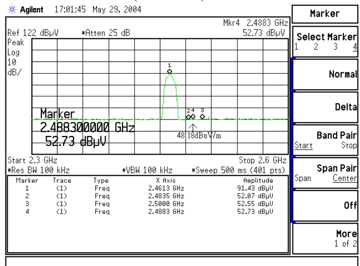
Figure Channel 11: (Vertical)
