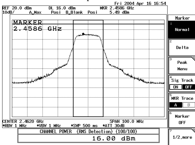
11Mbps-CH11
