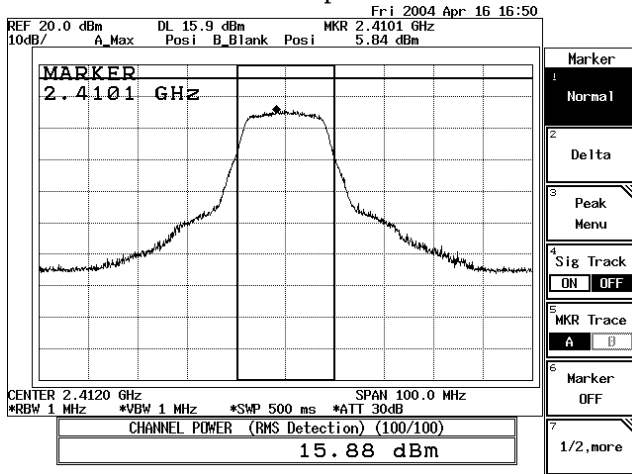
11Mbps-CH01
