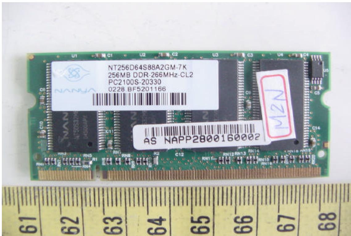
79. Front View of RAM 1
