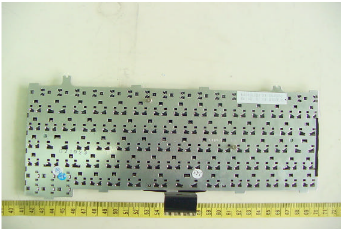
70. Bottom View of Keyboard
