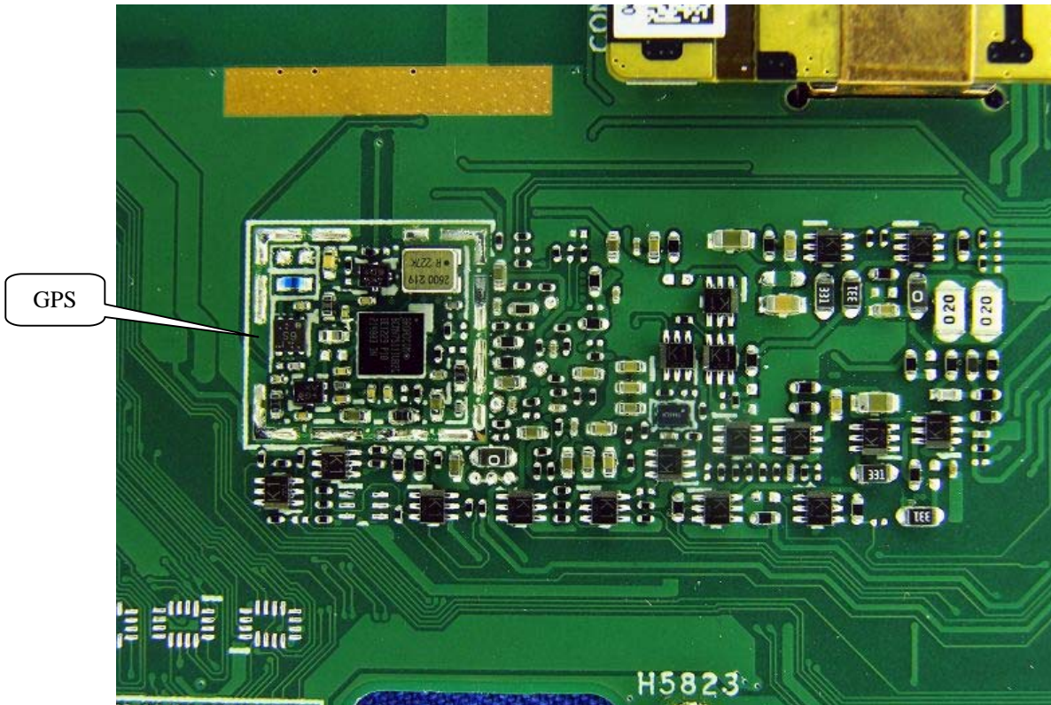
(27) EUT Photo
