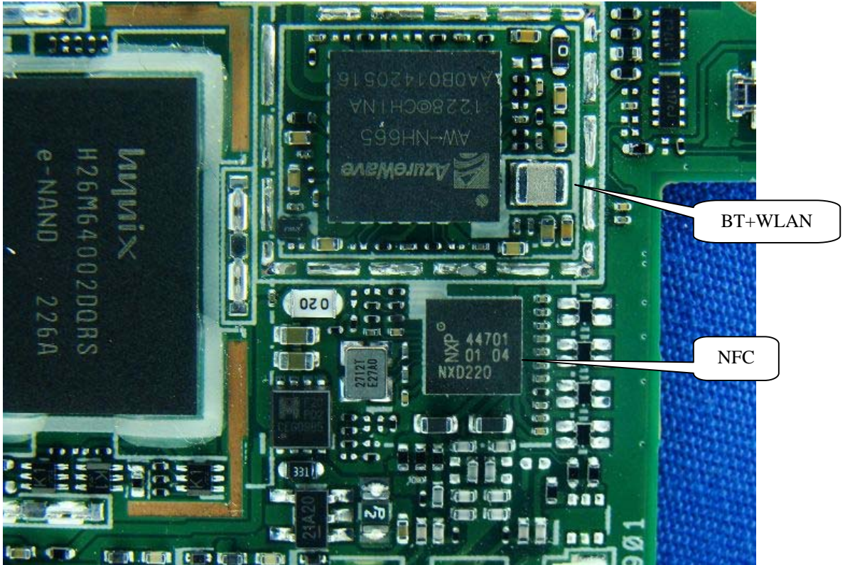
(23) EUT Photo
