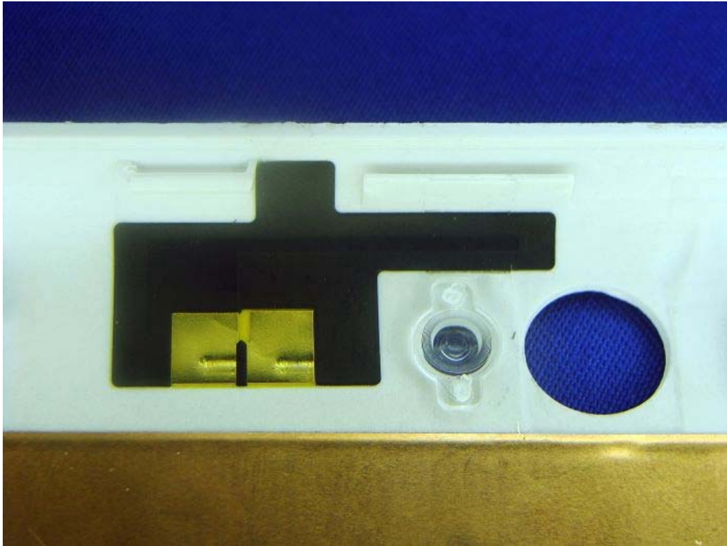
(9) EUT Photo (Antenna-GPS)
