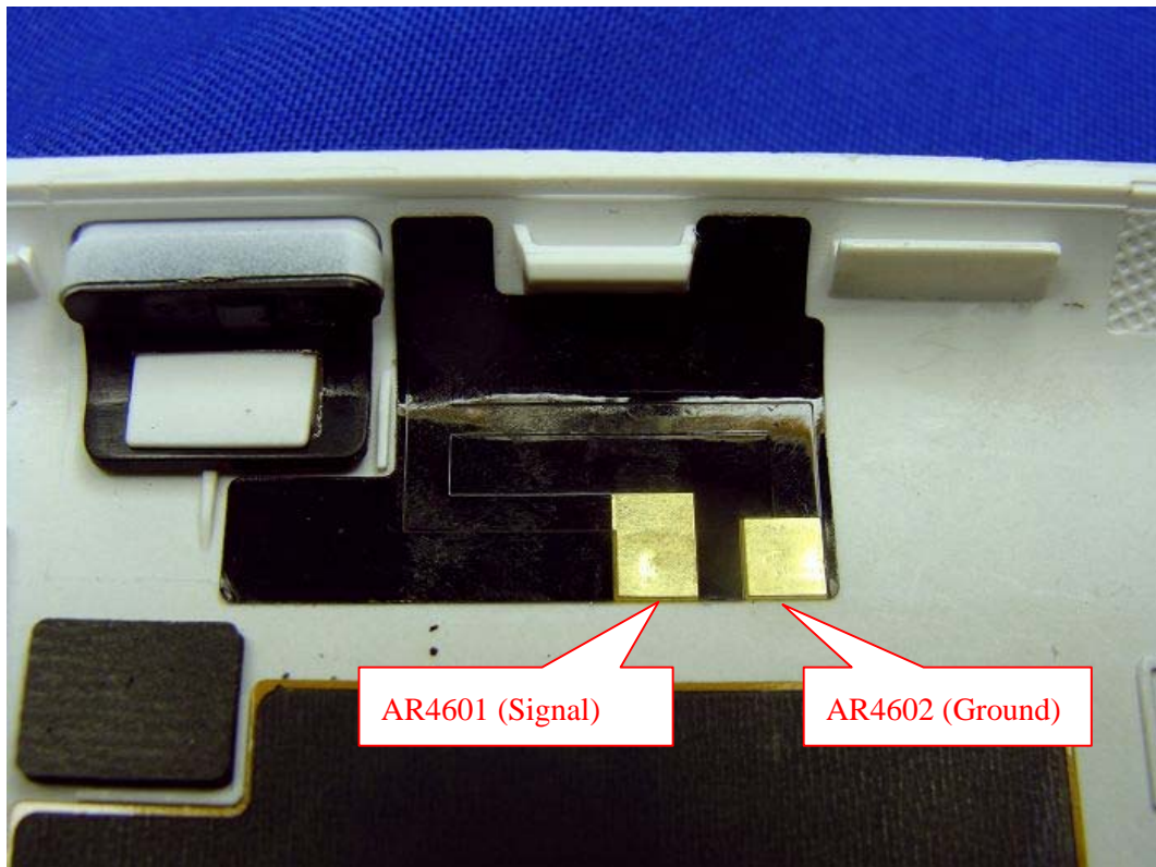
(12) EUT Photo (Antenna-WLAN+BT) - (MFR: SINBON)
