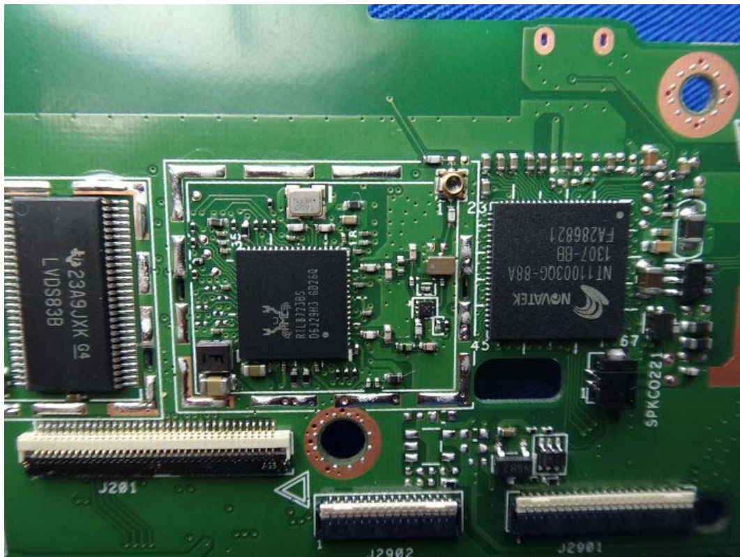
(18) EUT Photo (Bluetooth + WLAN Chip)
