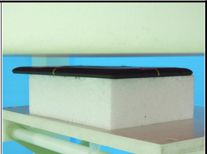
Rear Face of EUT with 12 mm Gap
