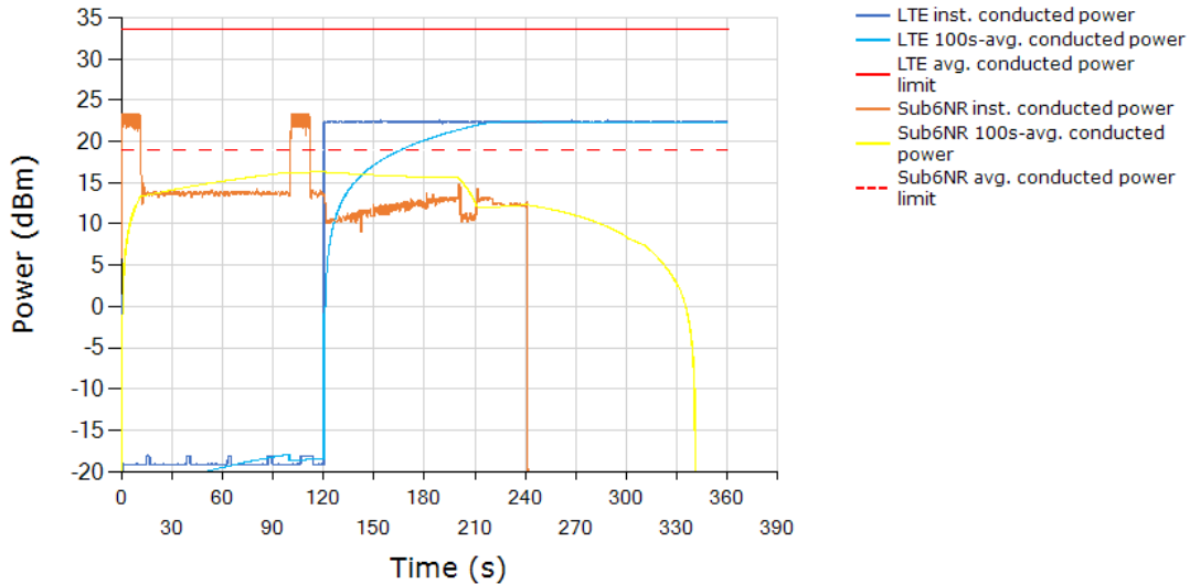
LTE and Sub6NR Instantaneous and Time-averaged TX Power Tech: LTE, Band 66 / Tech: NR5G SUB6, Band n25
