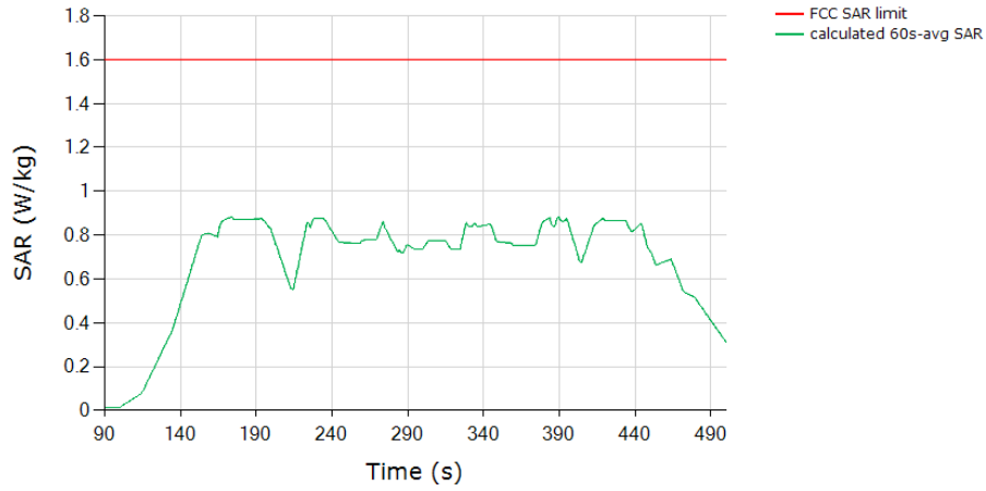
SAR (Test Sequence 2) Tech: LTE, Band 43
