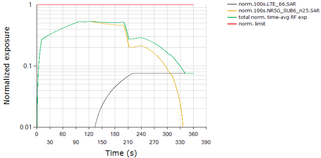
Total Normalized Time-averaged RF Exposure Tech: LTE, Band 66 / Tech: NR5G SUB6, Band n25
