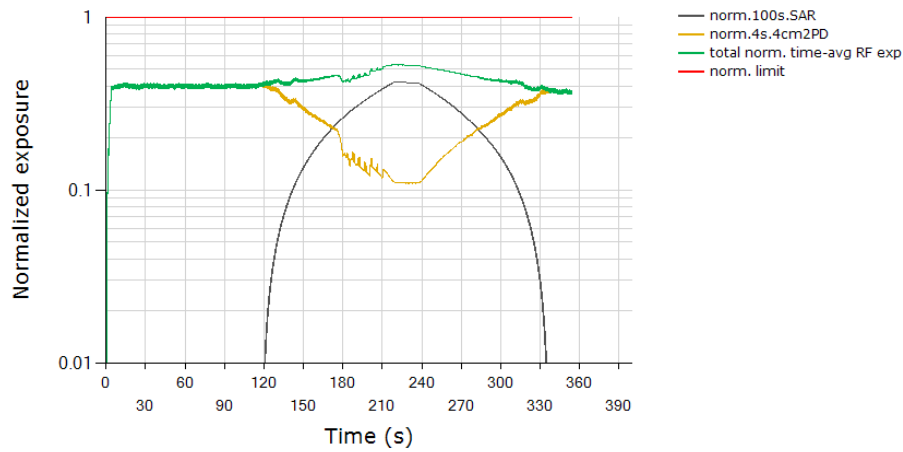
Total Normalized Time-averaged RF Exposure Tech: LTE, Band 2 / Tech: NR5G MMW, Band n257
