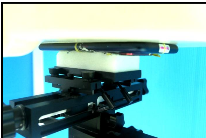
Body - Front Face of EUT at 0 mm
