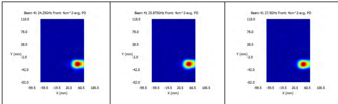
n258 / Beam ID: 42 / Back surface
