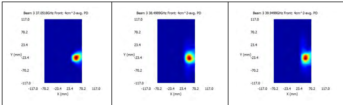
n260 / Beam ID: 4 / Back surface
