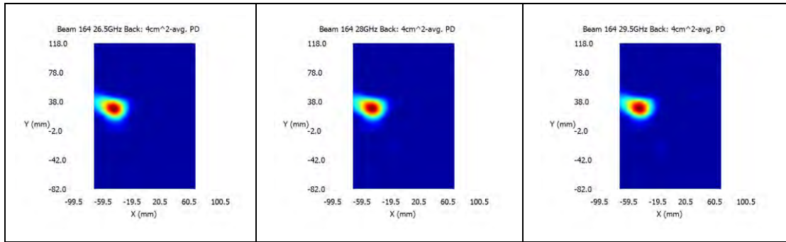
n257 / Beam ID: 164 / Front surface
