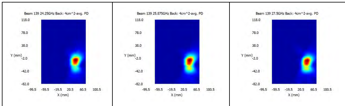
n258 / Beam ID: 139 / Front surface
