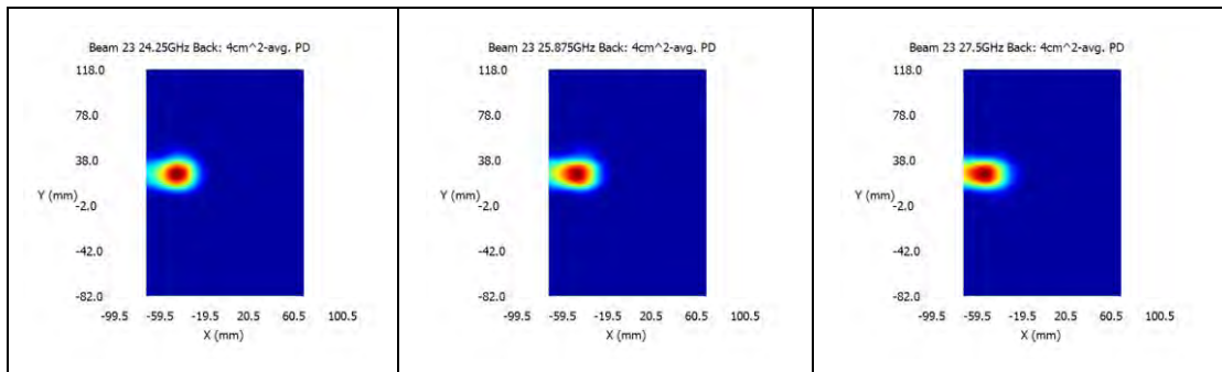
n258 / Beam ID: 23 / Front surface
