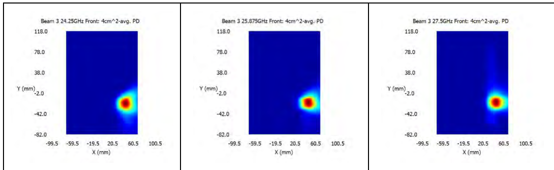
n258 / Beam ID: 4 / Back surface
