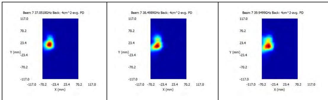
n262 / Beam ID: 7 / Front surface
