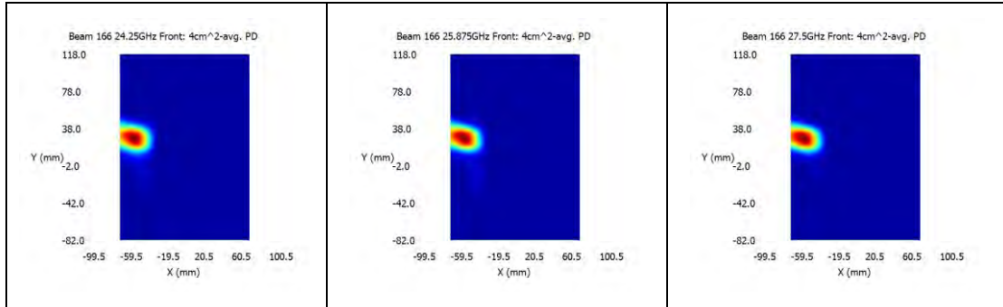
n258 / Beam ID: 167 / Back surface
