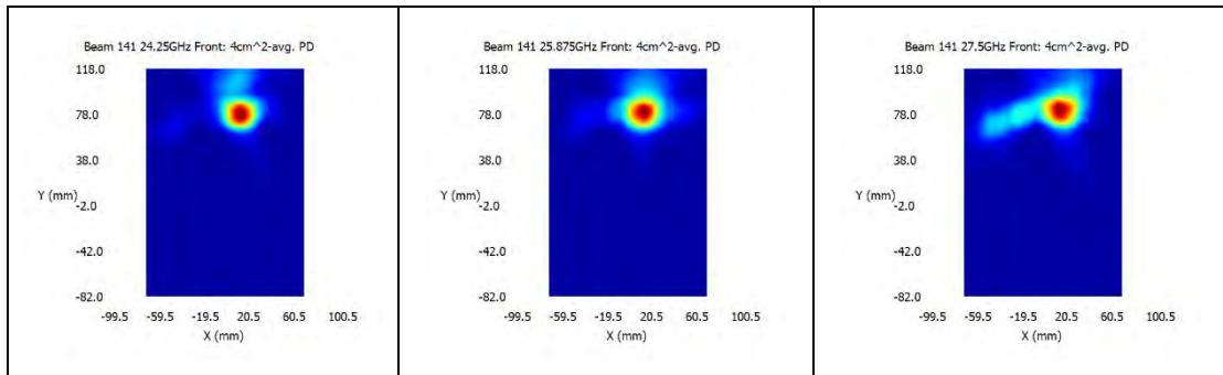
n258 / Beam ID: 142 / Back surface
