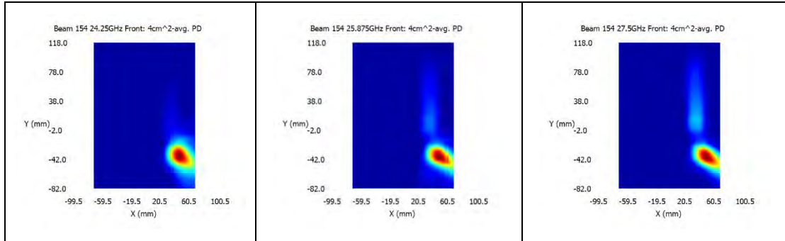
n258 / Beam ID: 155 / Back surface
