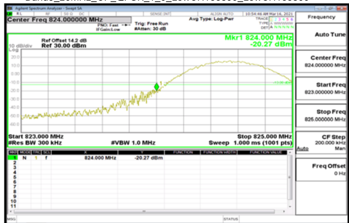
Band5_20MHz_CP_QPSK_1_0_LowCH166800_LowCH166800
