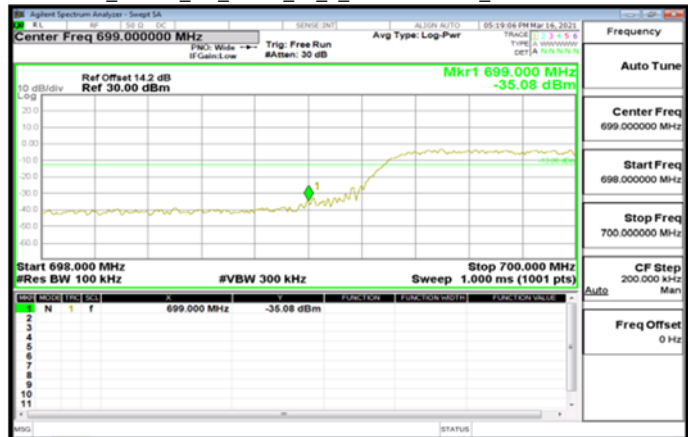
Band12_10MHz_CP_QPSK_52_0_LowCH140800_LowCH140800
