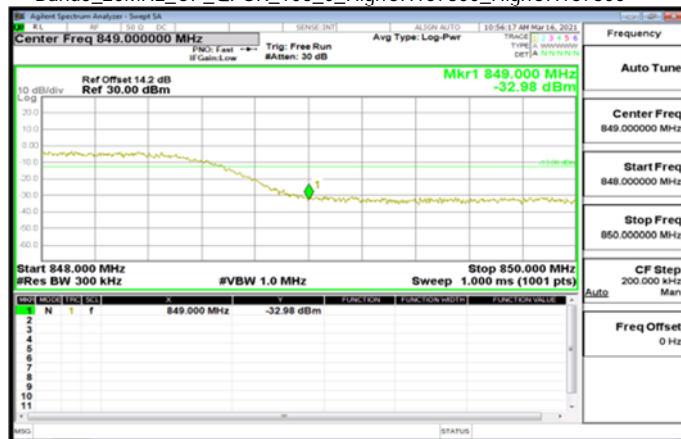
Band5_20MHz_CP_QPSK_106_0_HighCH167800_HighCH167800
