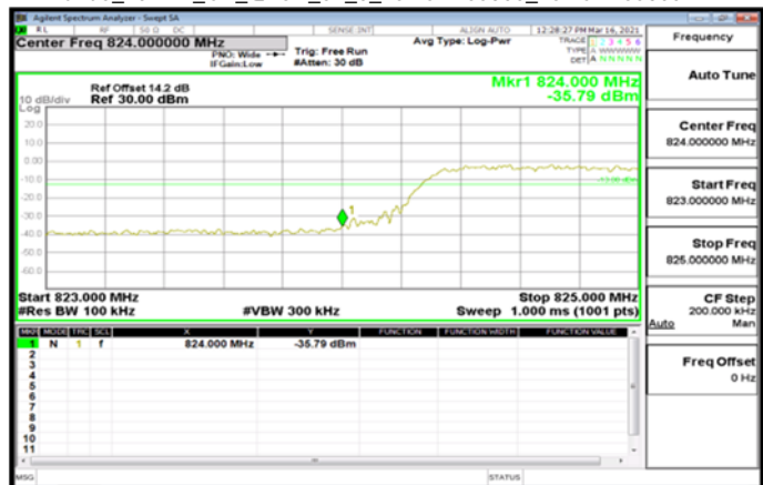
Band5_10MHz_CP_QPSK_52_0_LowCH165800_LowCH165800
