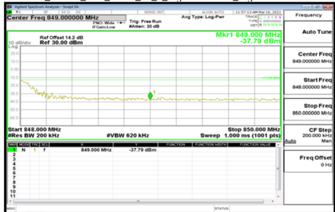
Band5_15MHz_DFT_BPSK_75_0_HighCH168300_HighCH168300
