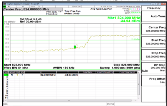
Band5_5MHz_DFT_BPSK_25_0_LowCH165300_LowCH165300
