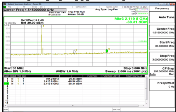
Band12_15MHz_DFT_BPSK_1_1_MidCH141500_MidCH141500
