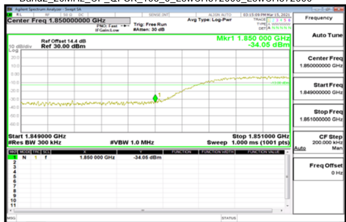
Band2_20MHz_CP_QPSK_106_0_LowCH372000_LowCH372000
