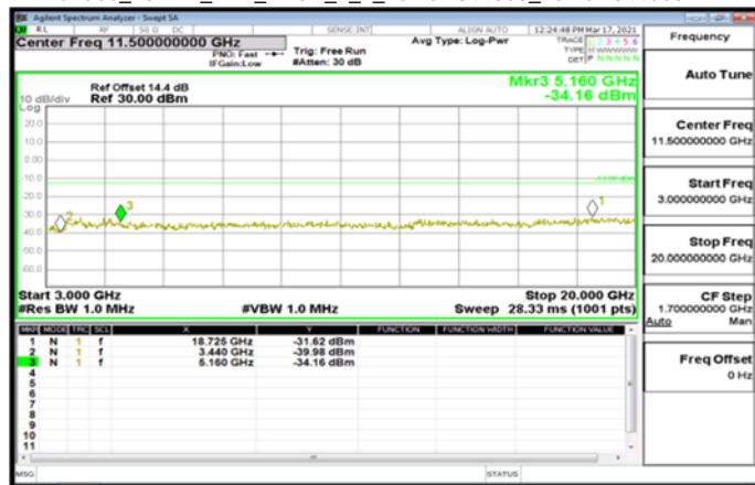
Band66_20MHz_DFT_BPSK_1_1_MidCH349000_MidCH349000
