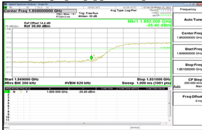
Band2_15MHz_DFT_BPSK_75_0_LowCH371500_LowCH371500
