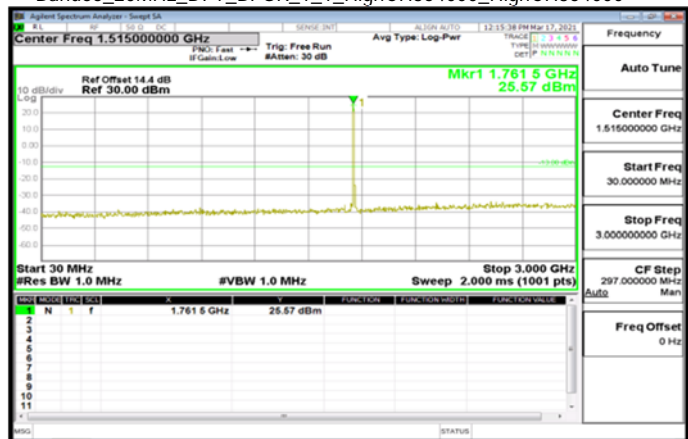
Band66_20MHz_DFT_BPSK_1_1_HighCH354000_HighCH354000
