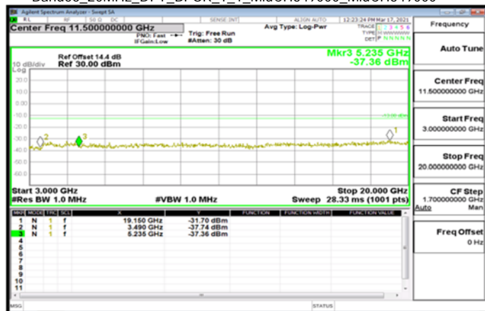
Band66_20MHz_DFT_BPSK_1_1_HighCH354000_HighCH354000
