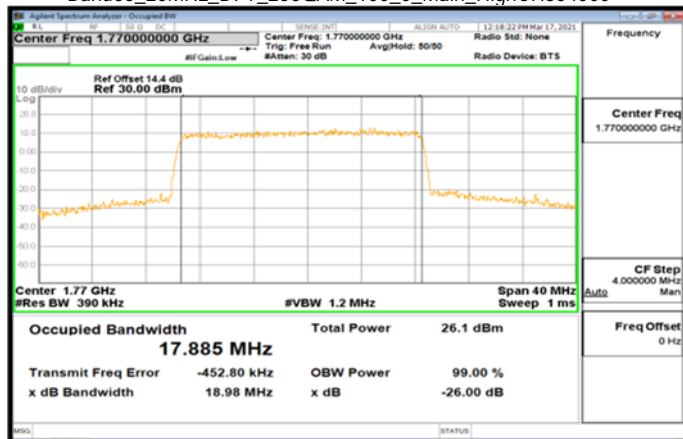
Band66_20MHz_DFT_256QAM_100_0_Main_HighCH354000
