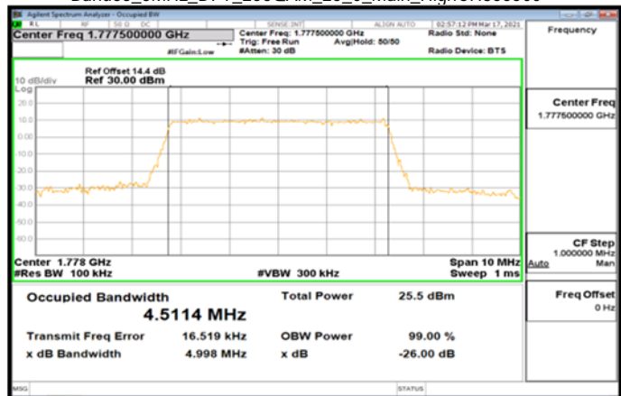
Band66_5MHz_DFT_256QAM_25_0_Main_HighCH355500
