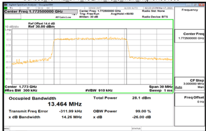
Band66_15MHz_DFT_16QAM_75_0_Main_HighCH354500
