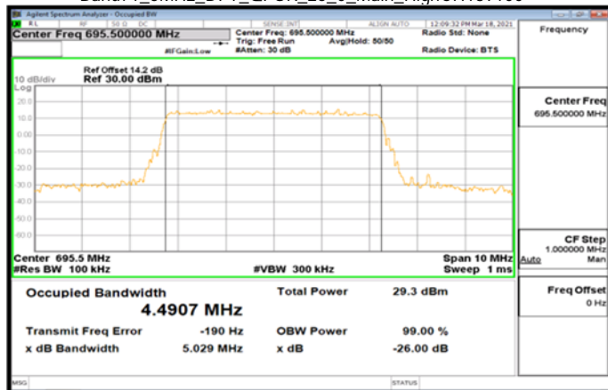
Band71_5MHz_DFT_QPSK_25_0_Main_HighCH139100
