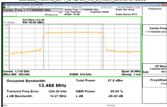
Band66_15MHz_DFT_64QAM_75_0_Main_MidCH349000
