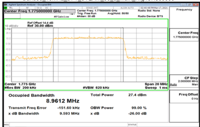
Band66_10MHz_DFT_64QAM_50_0_Main_HighCH355000
