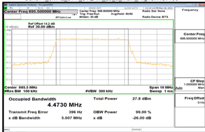
Band71_5MHz_DFT_64QAM_25_0_Main_HighCH139100
