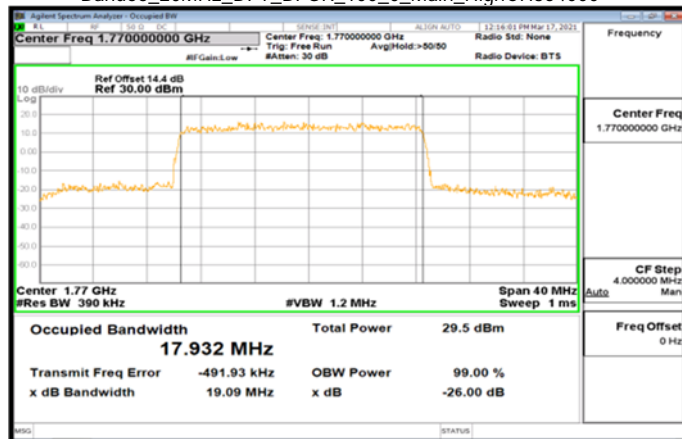
Band66_20MHz_DFT_BPSK_100_0_Main_HighCH354000
