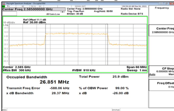
Band38_30MHz_DFT_QPSK_75_0_Main_LowCH517000
