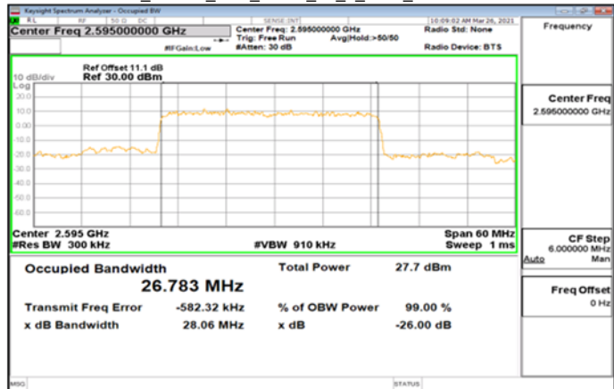
Band38_30MHz_DFT_BPSK_75_0_Main_MidCH519000
