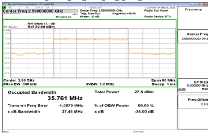
Band38_40MHz_DFT_BPSK_100_0_Main_LowCH518000
