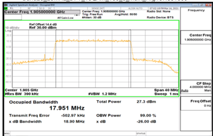
Band25_20MHz_DFT_16QAM_100_0_Main_HighCH381000
