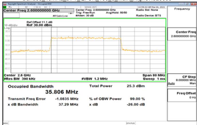
Band38_40MHz_DFT_QPSK_100_0_Main_HighCH520000
