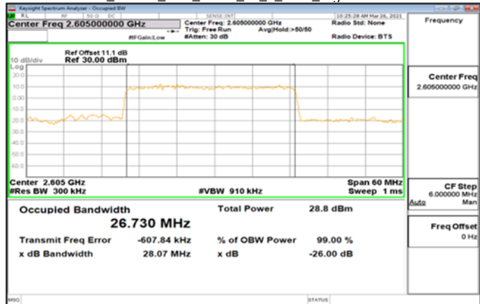
Band38_30MHz_DFT_BPSK_75_0_Main_HighCH521000
