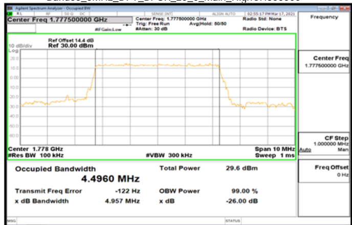
Band66_5MHz_DFT_BPSK_25_0_Main_HighCH355500
