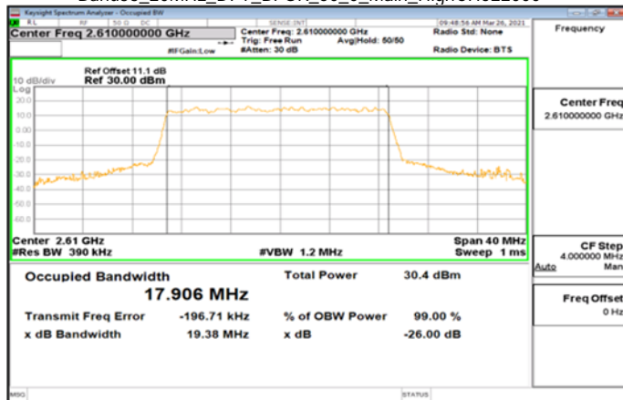
Band38_20MHz_DFT_BPSK_50_0_Main_HighCH522000
