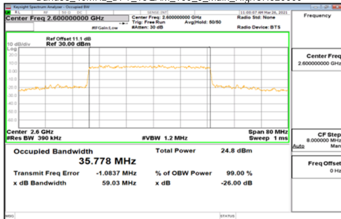
Band38_40MHz_DFT_16QAM_100_0_Main_HighCH520000
