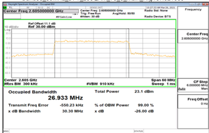
Band38_30MHz_DFT_256QAM_75_0_Main_HighCH521000
