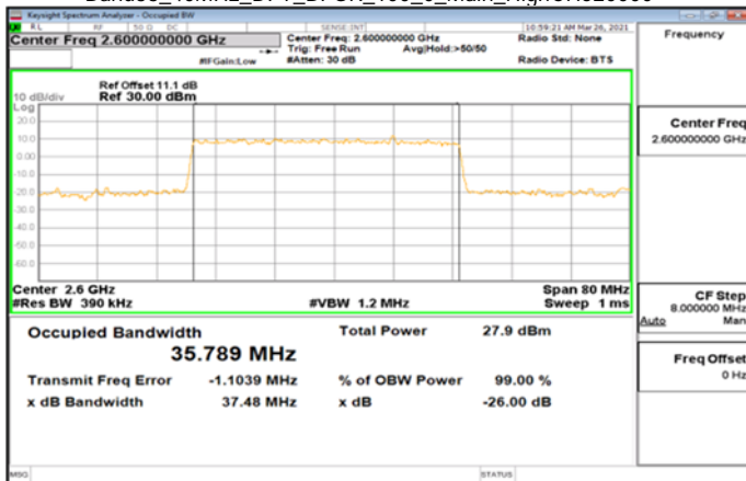
Band38_40MHz_DFT_BPSK_100_0_Main_HighCH520000
