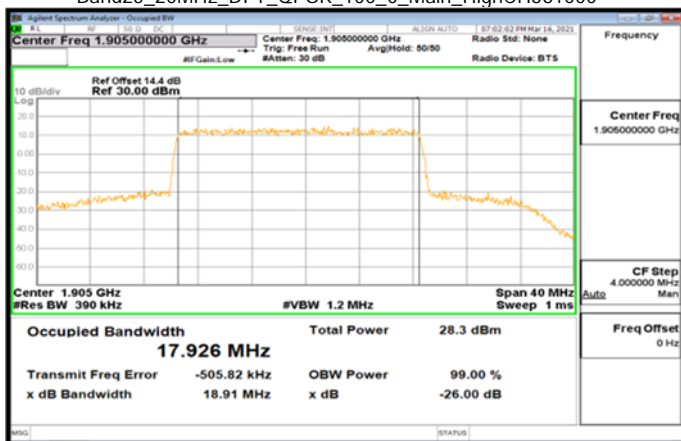
Band25_20MHz_DFT_QPSK_100_0_Main_HighCH381000
