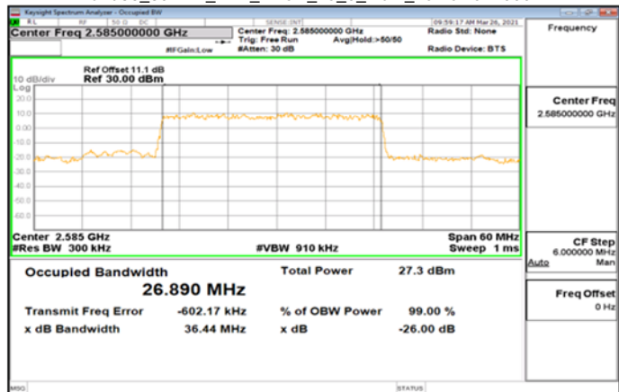
Band38_30MHz_DFT_BPSK_75_0_Main_LowCH517000
