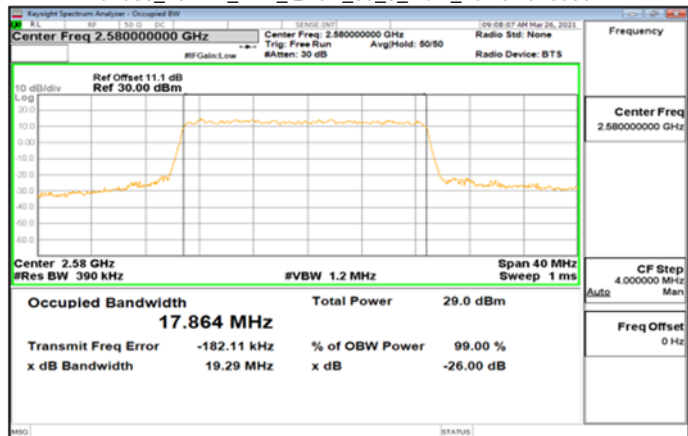
Band38_20MHz_DFT_QPSK_50_0_Main_LowCH516000
