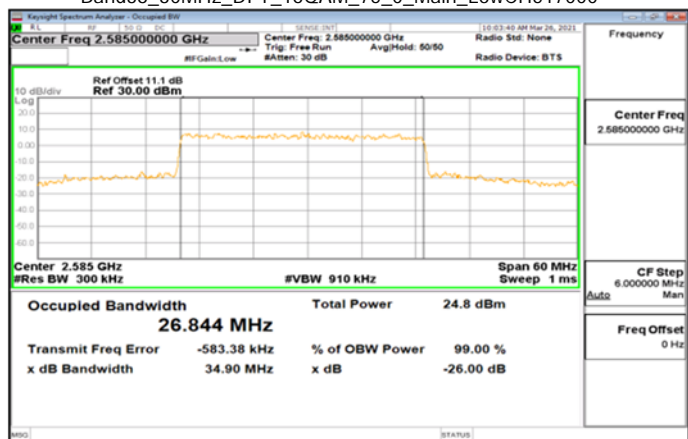
Band38_30MHz_DFT_16QAM_75_0_Main_MidCH519000
