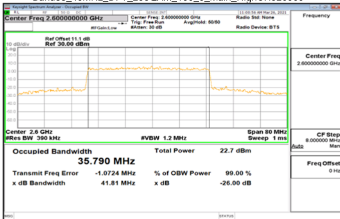
Band38_40MHz_DFT_256QAM_100_0_Main_HighCH520000
