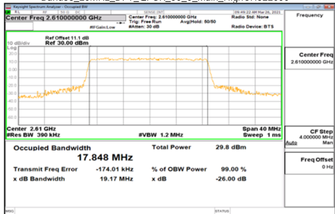
Band38_20MHz_DFT_QPSK_50_0_Main_HighCH522000
