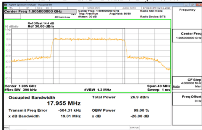
Band25_20MHz_DFT_64QAM_100_0_Main_HighCH381000
