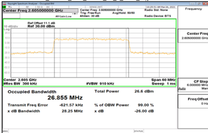
Band38_30MHz_DFT_QPSK_75_0_Main_HighCH521000
