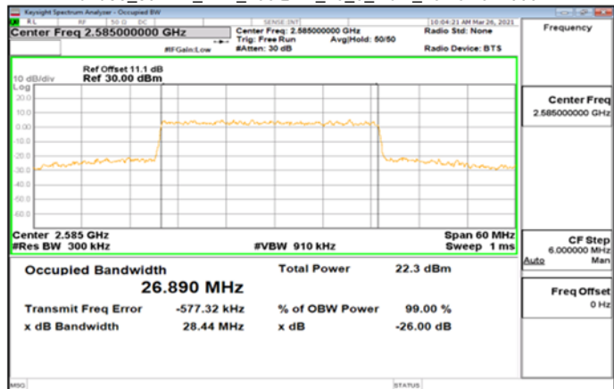
Band38_30MHz_DFT_256QAM_75_0_Main_LowCH517000
