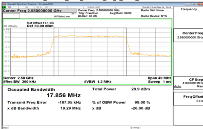
Band38_20MHz_DFT_16QAM_50_0_Main_LowCH516000
