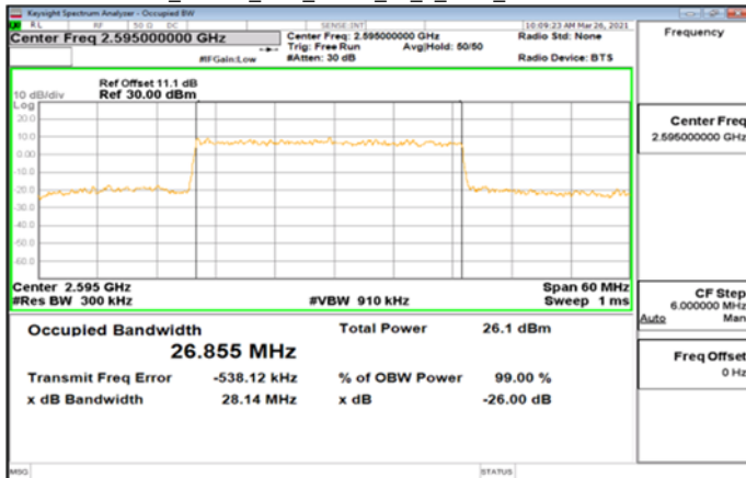
Band38_30MHz_DFT_QPSK_75_0_Main_MidCH519000
