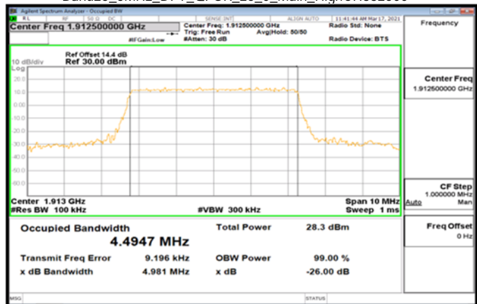
Band25_5MHz_DFT_QPSK_25_0_Main_HighCH382500
