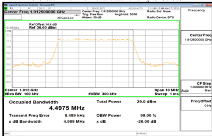
Band25_5MHz_DFT_BPSK_25_0_Main_HighCH382500
