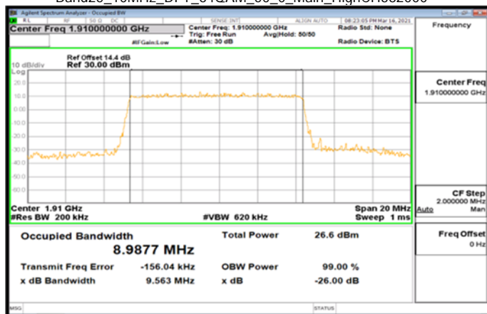
Band25_10MHz_DFT_64QAM_50_0_Main_HighCH382000
