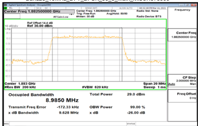
Band25_10MHz_DFT_BPSK_50_0_Main_MidCH376500
