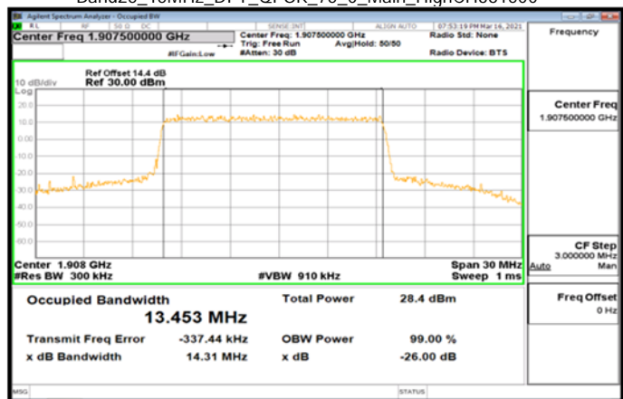
Band25_15MHz_DFT_QPSK_75_0_Main_HighCH381500
