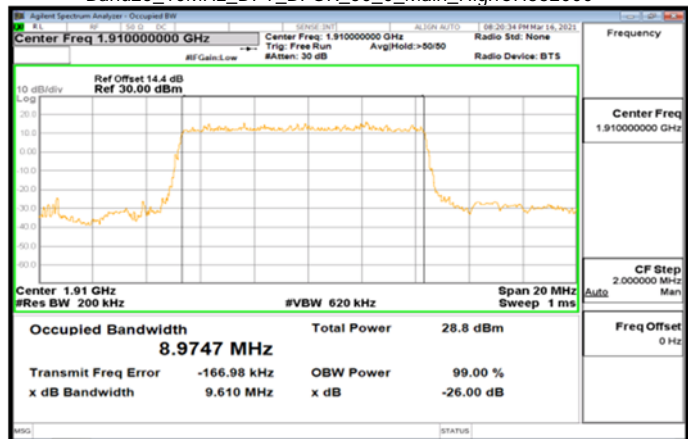
Band25_10MHz_DFT_BPSK_50_0_Main_HighCH382000
