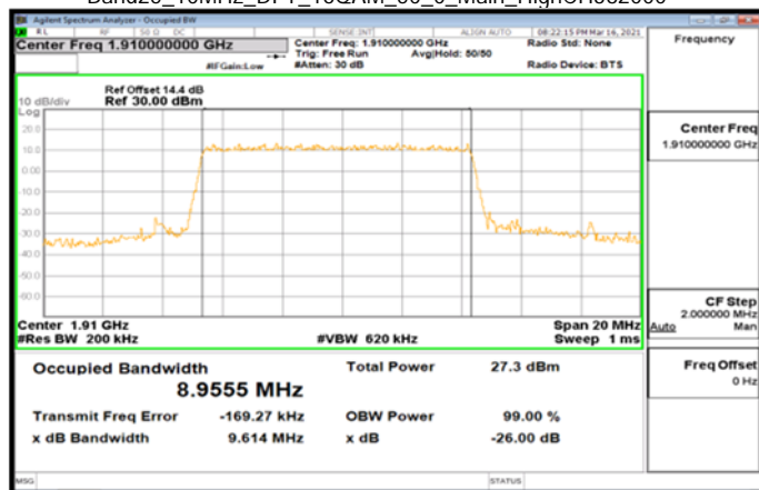
Band25_10MHz_DFT_16QAM_50_0_Main_HighCH382000
