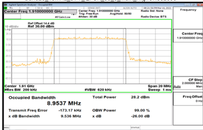
Band25_10MHz_DFT_QPSK_50_0_Main_HighCH382000
