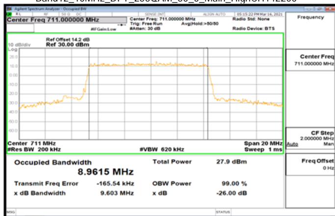
Band12_10MHz_DFT_256QAM_50_0_Main_HighCH142200
