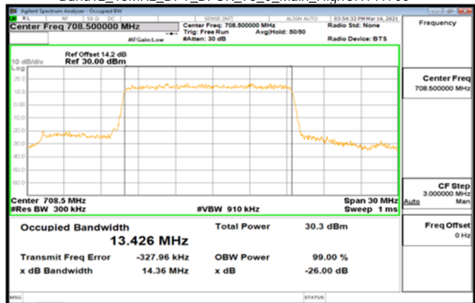
Band12_15MHz_DFT_BPSK_75_0_Main_HighCH141700
