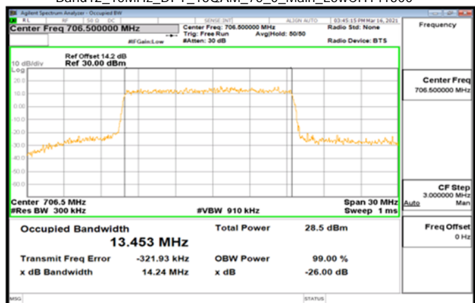
Band12_15MHz_DFT_16QAM_75_0_Main_MidCH141500
