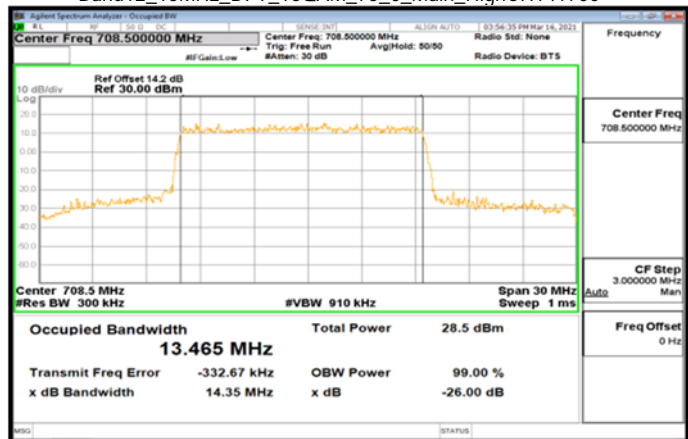
Band12_15MHz_DFT_16QAM_75_0_Main_HighCH141700
