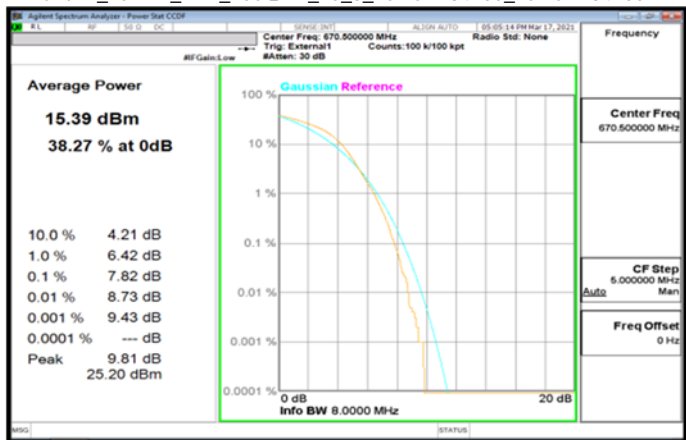
Band71_15MHz_DFT_256QAM_75_0_LowCH134100_LowCH134100
