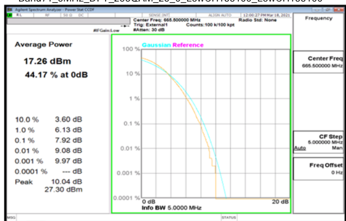
Band71_5MHz_DFT_256QAM_25_0_MidCH136100_MidCH136100
