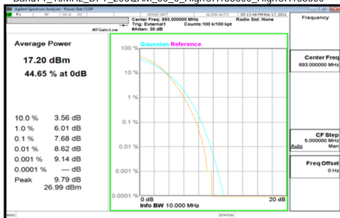
Band71_10MHz_DFT_256QAM_50_0_HighCH138600_HighCH138600
