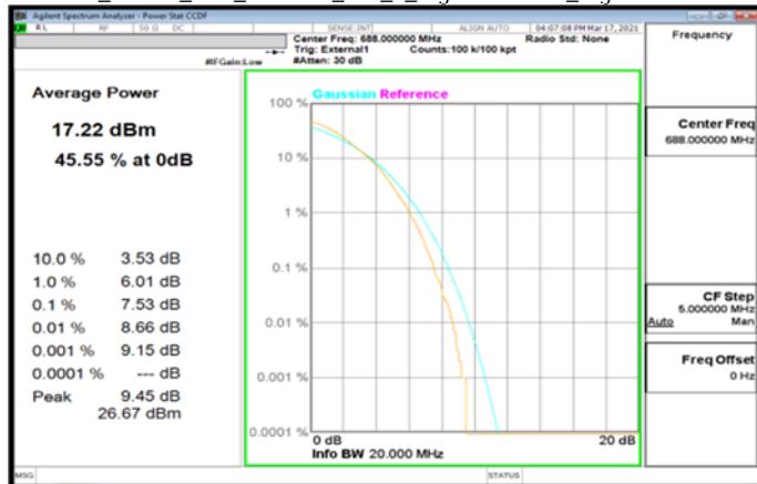
Band71_20MHz_DFT_256QAM_100_0_HighCH137600_HighCH137600
