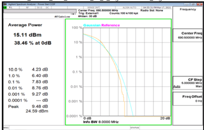
Band71_15MHz_DFT_256QAM_75_0_HighCH138100_HighCH138100
