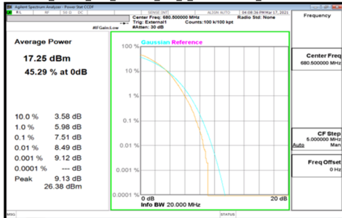
Band71_20MHz_DFT_256QAM_100_0_MidCH136100_MidCH136100
