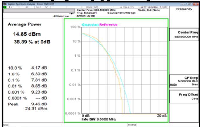
Band71_15MHz_DFT_256QAM_75_0_MidCH136100_MidCH136100
