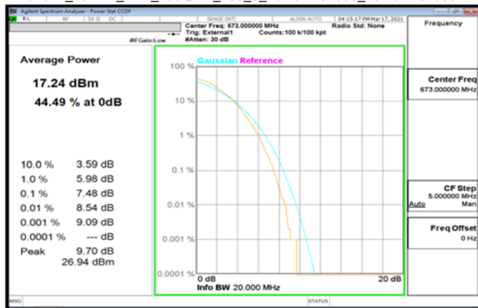
Band71_20MHz_DFT_256QAM_100_0_LowCH134600_LowCH134600
